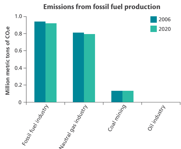
Figure 3.9 Baseline (2006) vs. Projected (2020) 'business-as-usual' emissions for fossil fuel production.
