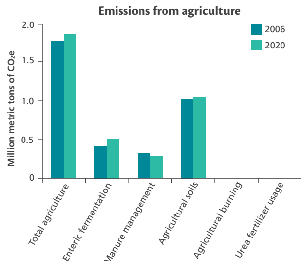
Figure 3.10 Baseline (2006) vs. Projected (2020) 'business-as-usual' emissions for agriculture.
