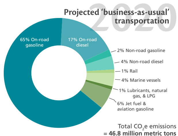
Figure 3.7 Baseline transportation emissions in 2006 compared with projected ‘business-as-usual’ transportation emissions in 2020 by sector. Overall CO 2 e transportation emissions are projected to increase by 11.3 million metric tons.
