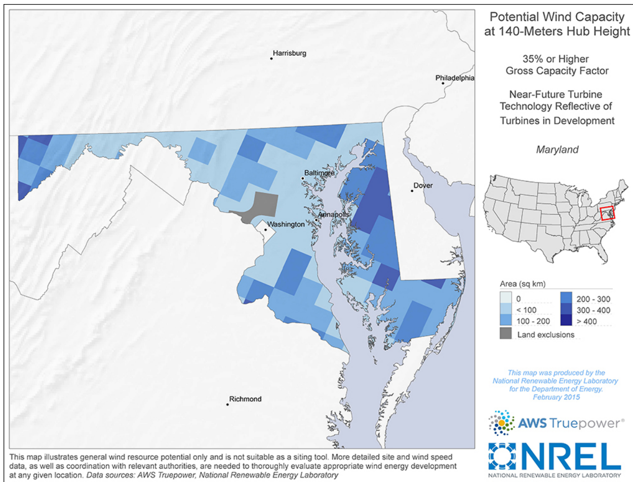
Figure XI-5: Areas where good quality wind resources (140-meter hub height) are available in Maryland Source: http://apps2.eere.energy.gov/wind/windexchange/wind_resource_maps.asp?stateab=md (DOE WINDEXchange 2015 (Maryland))
