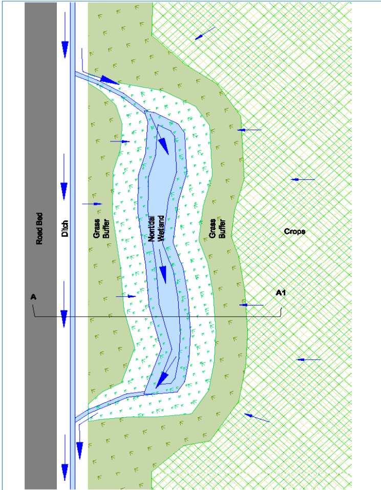
OFF-LINE WETLAND PLAN VIEW
