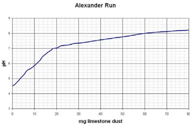
Figure 20. Titration Graph for Alexander Run
