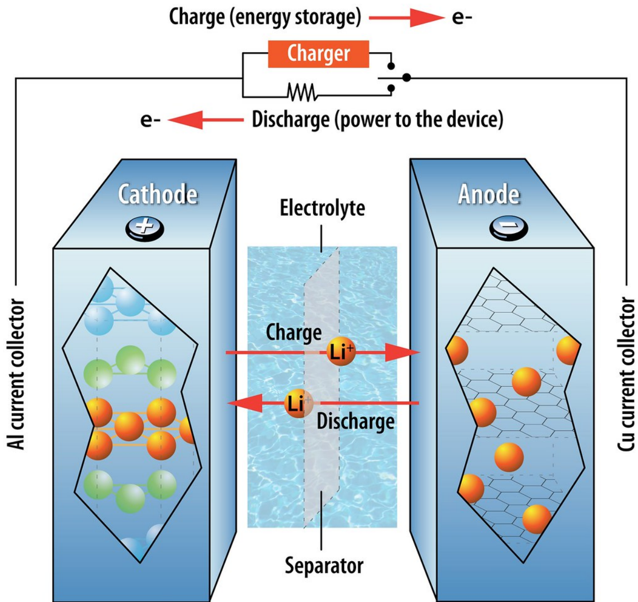
Figure 1: Diagram of an LIB.
