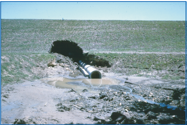
A failure due to internal erosion often leaves a tunnel-shaped void along the conduit.
