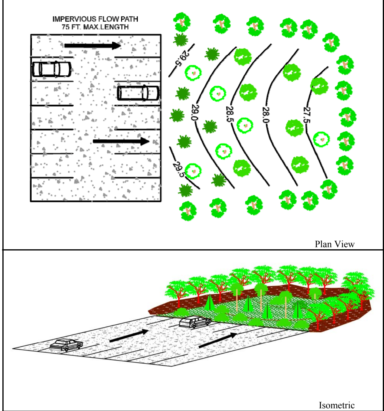
Figure 5.6 Non-Rooftop Disconnection
