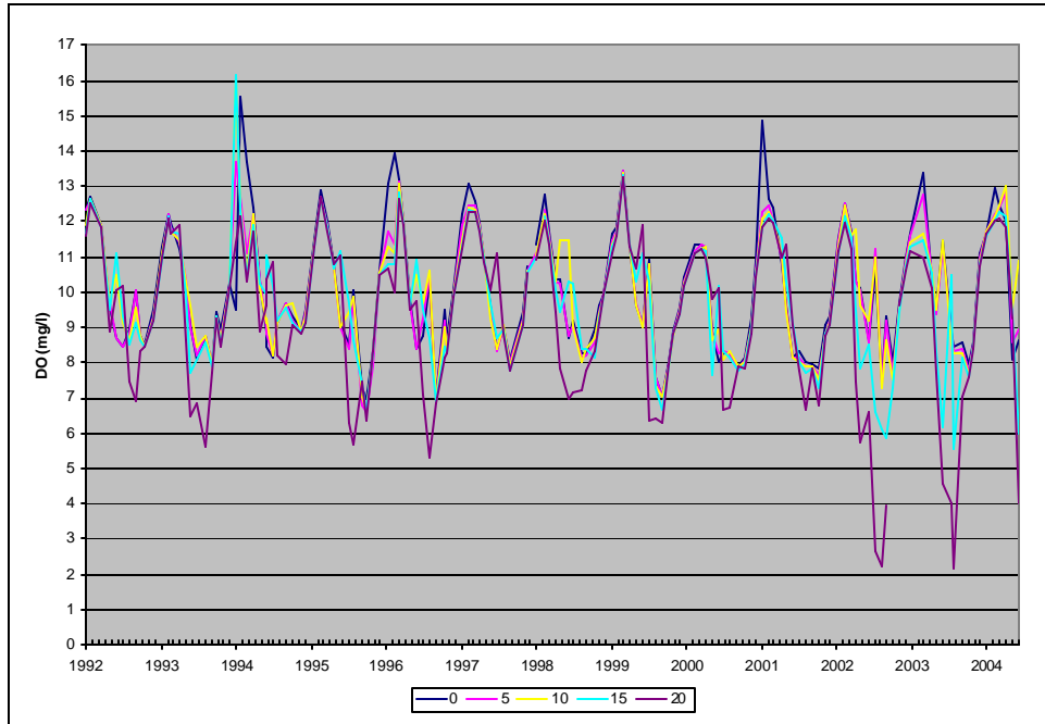
Figure A27: Average Surface Dissolved Oxygen. Middle Sampling Location, Prettyboy Reservoir.
