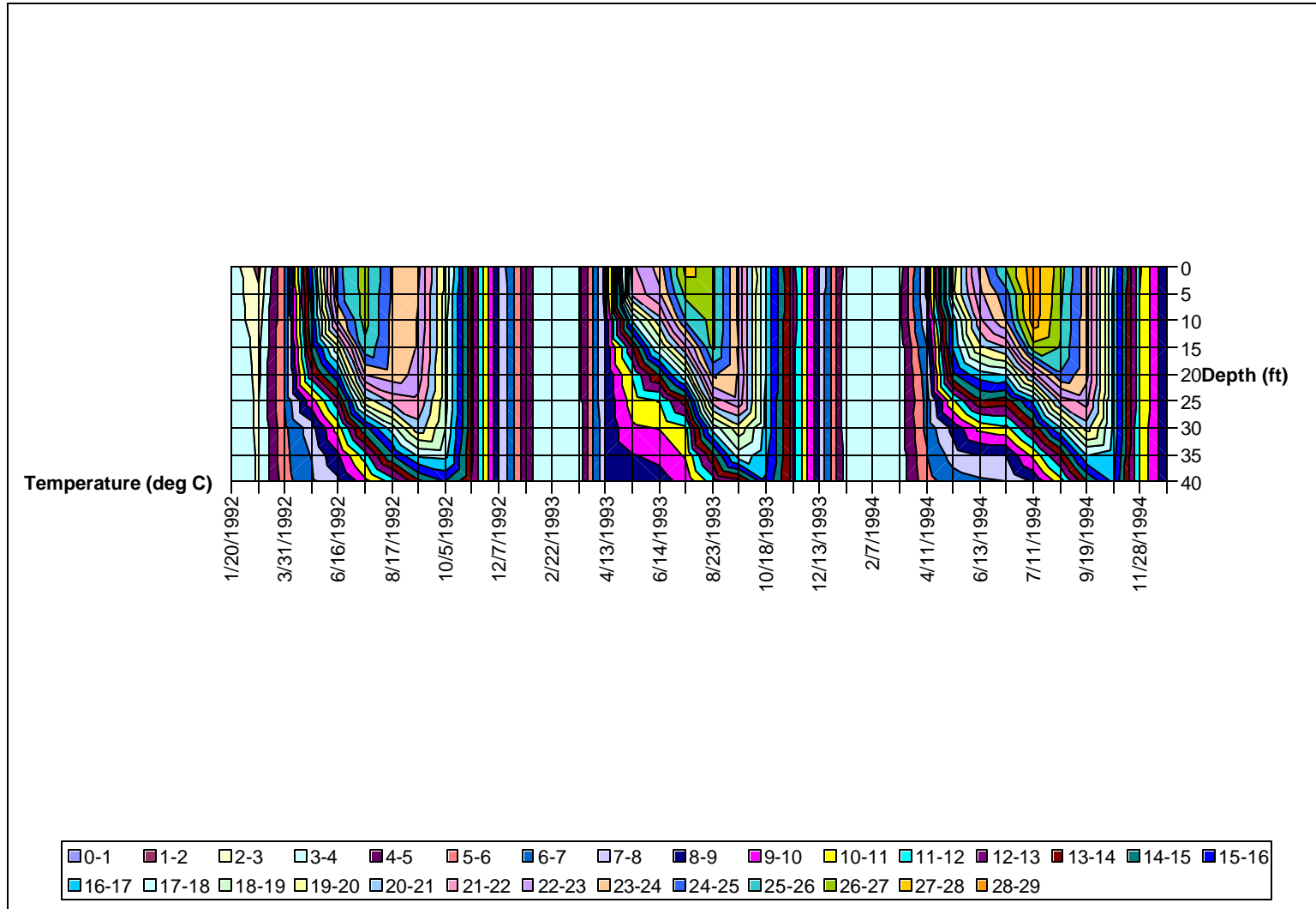
Figure A1: Isothermal Contours, Prettyboy Reservoir, Lower Sampling Locations, 1992-1995
