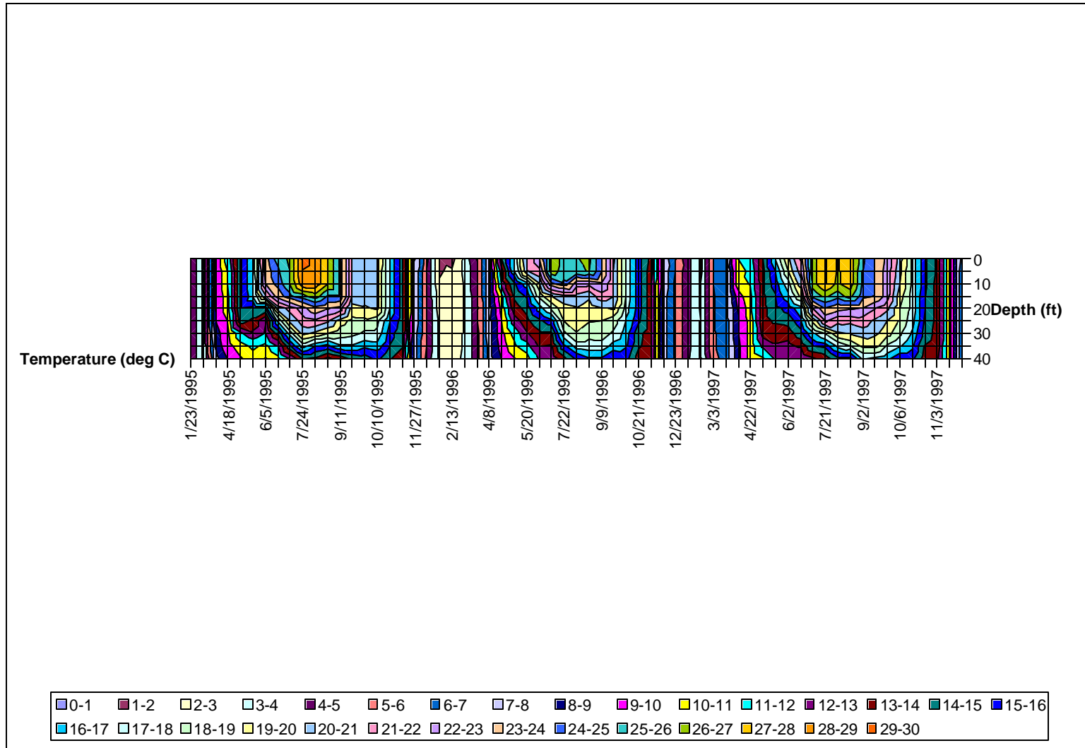
Figure A10: Isothermal Contours, Loch Raven Reservoir, Lower Sampling Locations, 1995-1997
