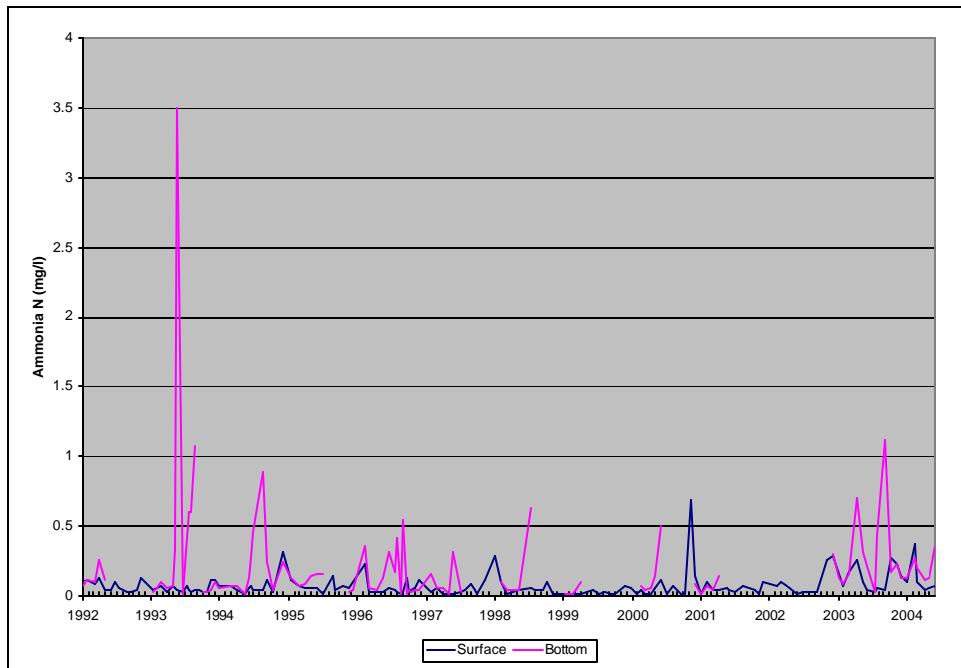
Figure A40: Average Ammonia Nitrogen. Upper Sampling Locations, Loch Raven Reservoir.
