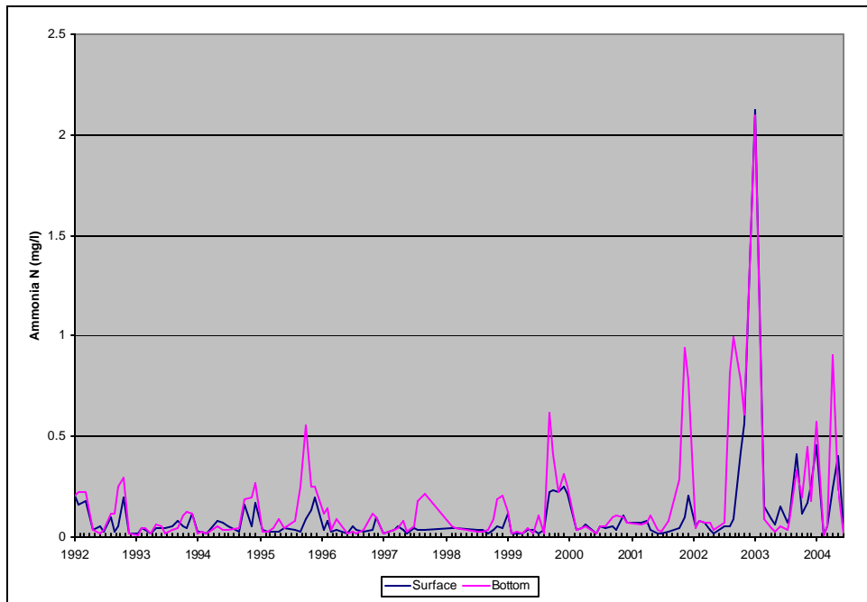
Figure A36: Average Ammonia Nitrogen. Lower Sampling Locations, Prettyboy Reservoir.
