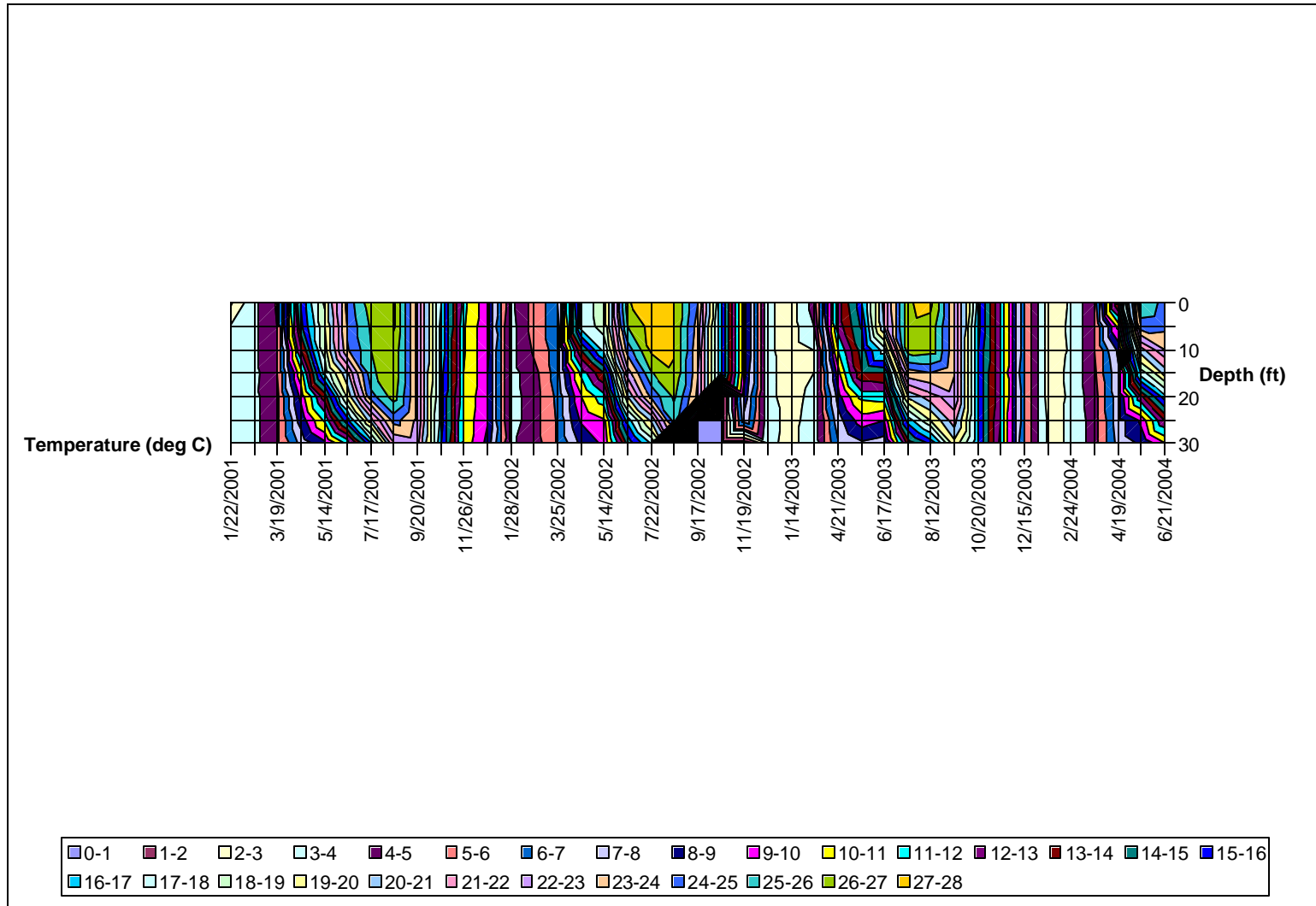
Figure A8: Isothermal Contours, Prettyboy Reservoir, Middle Sampling Location, 2001-2004
