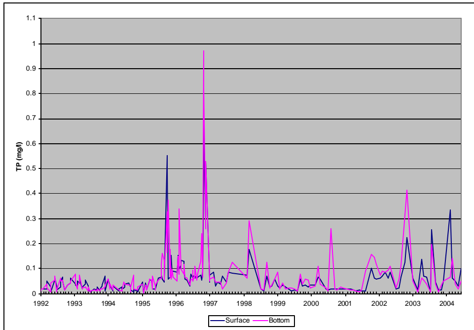
Figure A33: Average Total Phosphorus. Lower Sampling Location, Loch Raven Reservoir.
