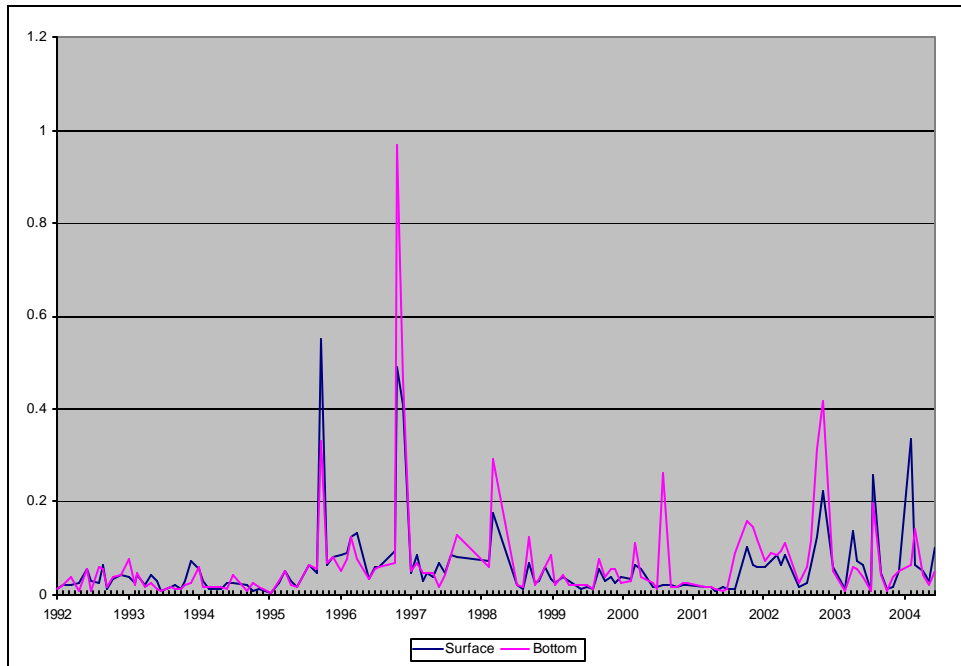
Figure A31: Average Total Phosphorus. Lower Sampling Locations, Prettyboy Reservoir.
