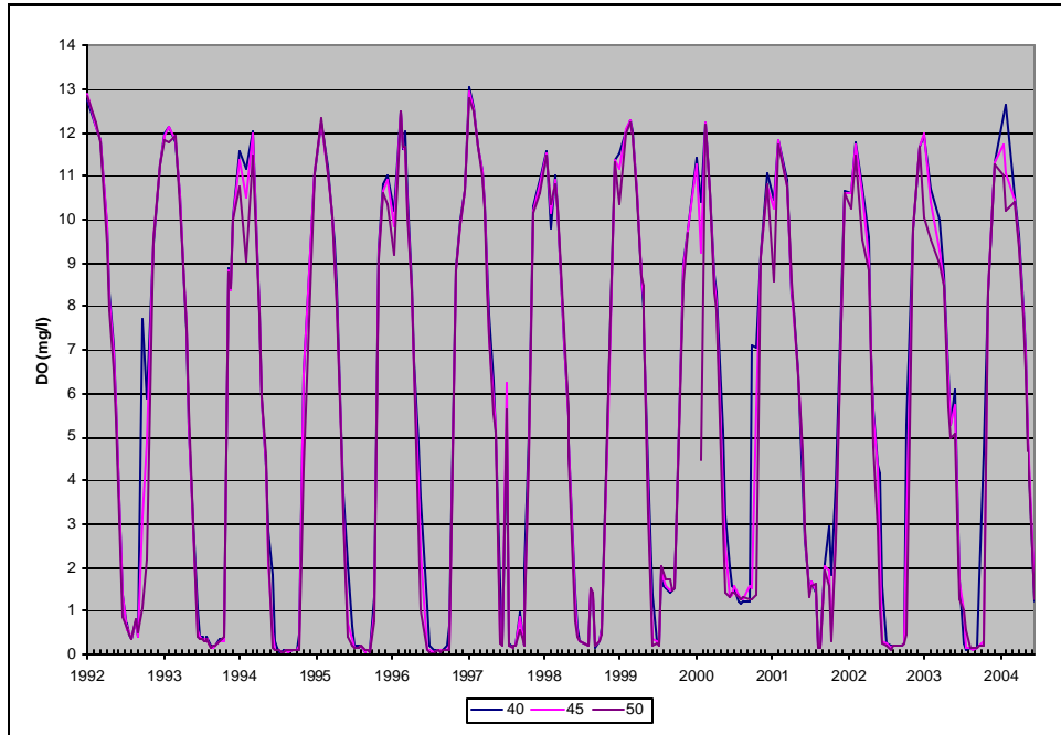
Figure A23: Average Bottom Dissolved Oxygen. Lower Sampling Location, Loch Raven Reservoir.
