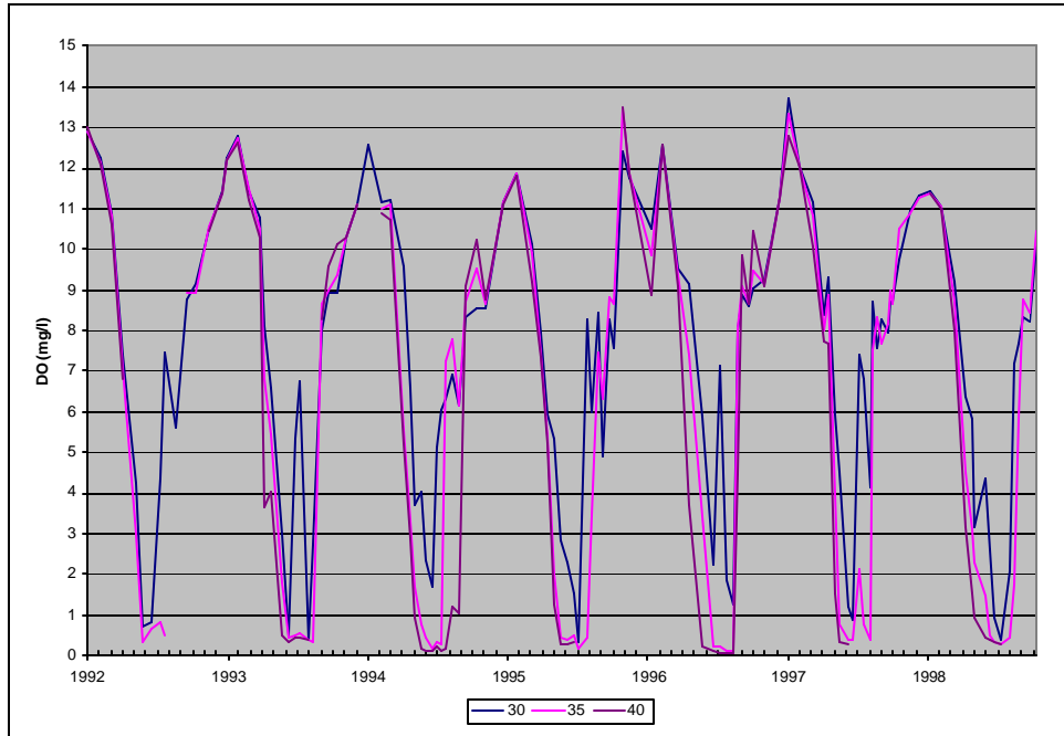
Figure A25: Average Bottom Dissolved Oxygen. Upper Sampling Locations, Loch Raven Reservoir.
