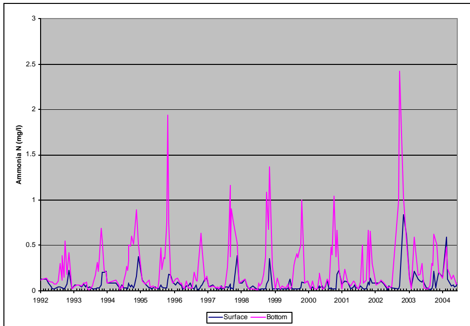
Figure A38: Average Ammonia Nitrogen. Lower Sampling Location, Loch Raven Reservoir.
