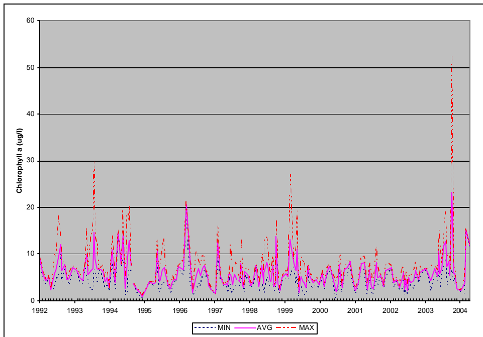
Figure A49: Surface Chlorophyll a. Middle Sampling Locations, Loch Raven Reservoir.
