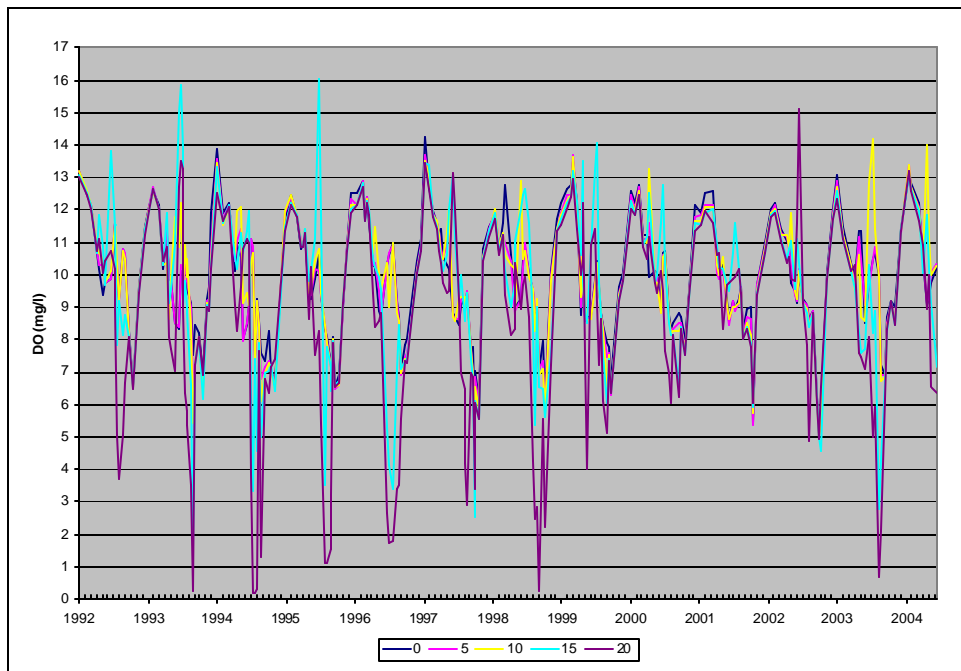
Figure A28: Average Surface Dissolved Oxygen. Lower Sampling Location, Loch Raven Reservoir.
