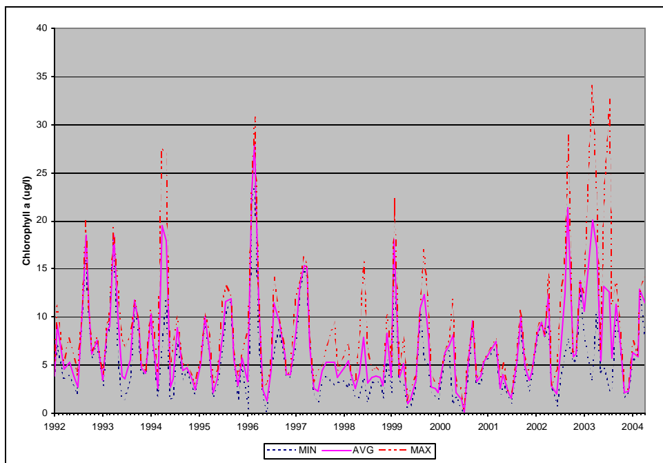
Figure A46: Surface Chlorophyll a. Lower Sampling Locations, Prettyboy Reservoir.
