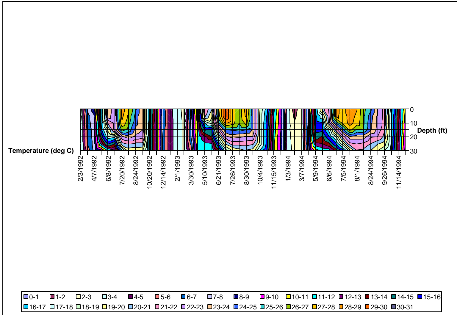
Figure A13: Isothermal Contours, Loch Raven Reservoir, Middle Sampling Locations, 1992-1994
