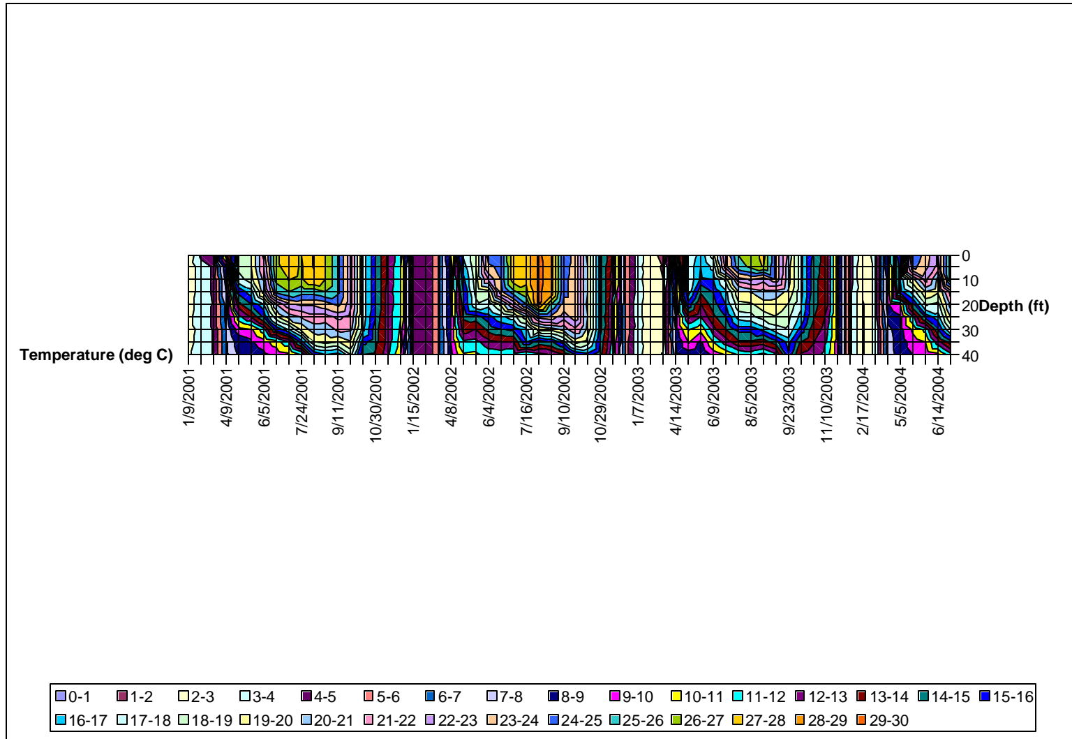
Figure A12: Isothermal Contours, Loch Raven Reservoir, Lower Sampling Locations, 2001-2004
