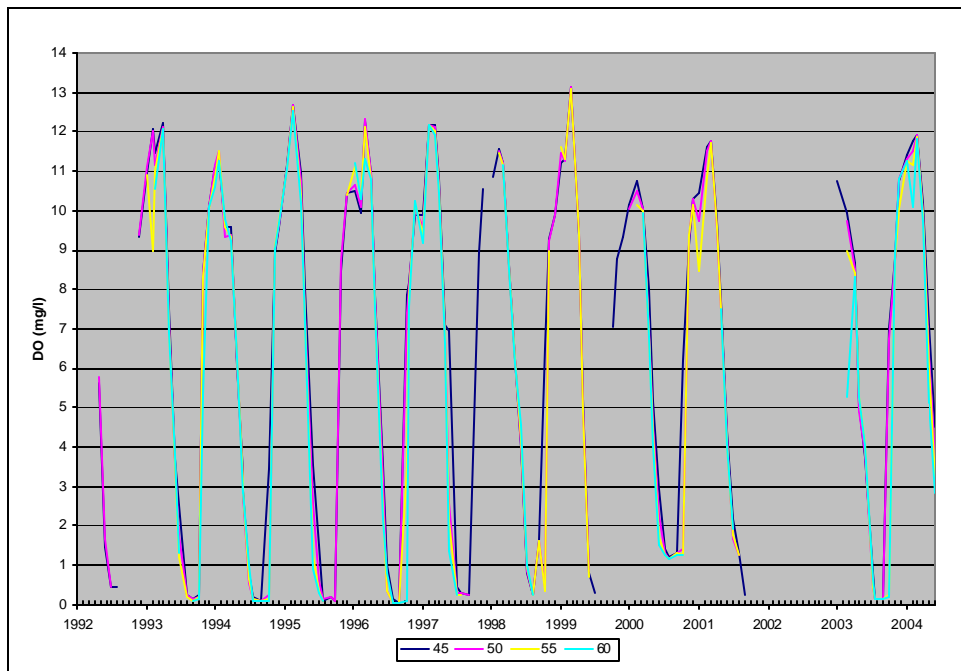
Figure A22: Average Bottom Dissolved Oxygen. Middle Sampling Location, Prettyboy Reservoir.
