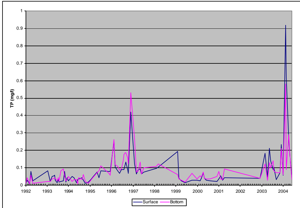
Figure A35: Average Total Phosphorus. Upper Sampling Locations, Loch Raven Reservoir.
