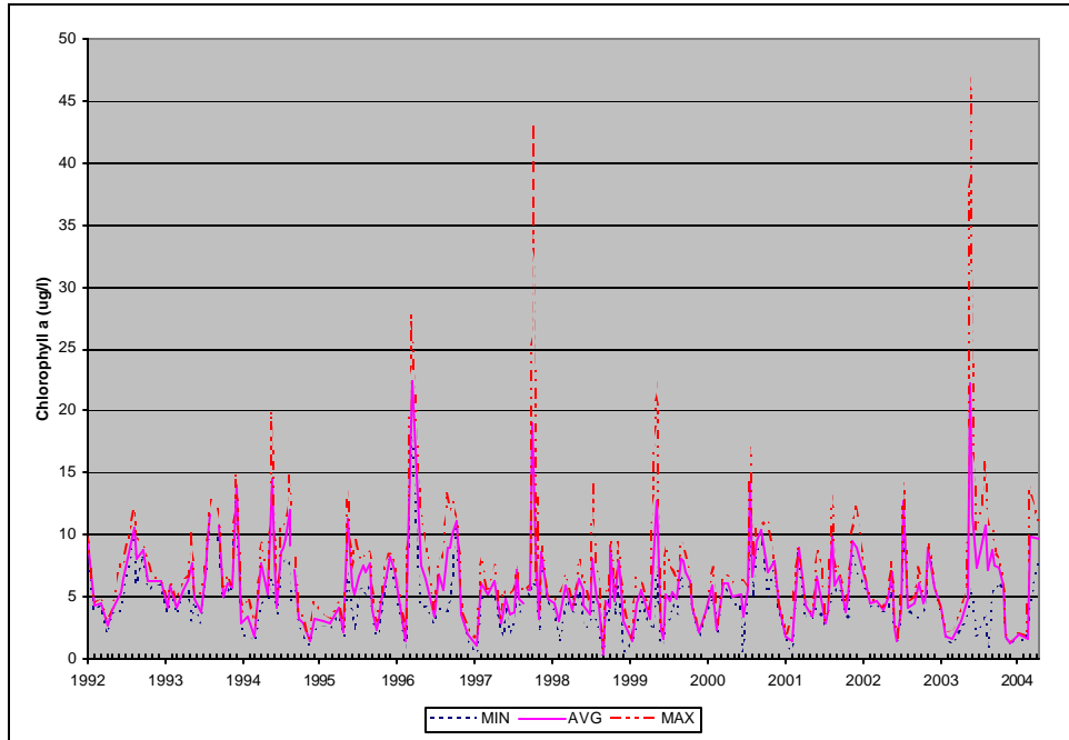
Figure A50: Surface Chlorophyll a. Upper Sampling Locations, Loch Raven Reservoir.
