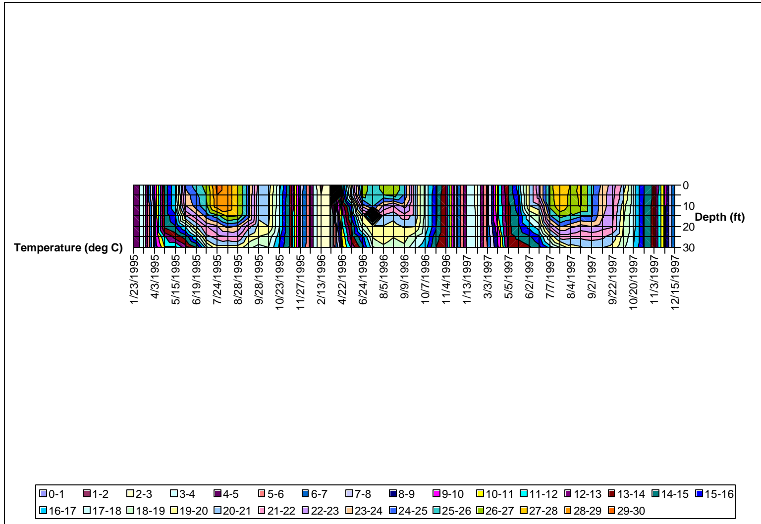
Figure A14: Isothermal Contours, Loch Raven Reservoir, Middle Sampling Locations, 1995-1997
