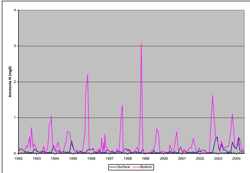
Figure A39: Average Ammonia Nitrogen. Middle Sampling Locations, Loch Raven Reservoir.
