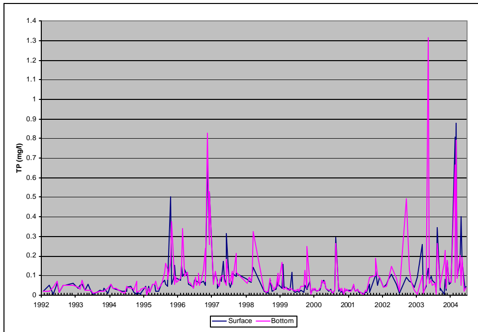
Figure A34: Average Total Phosphorus. Middle Sampling Locations, Loch Raven Reservoir.
