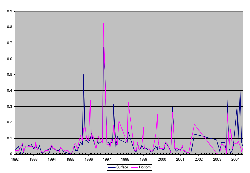
Figure A32: Average Total Phosphorus. Middle Sampling Location, Prettyboy Reservoir.
