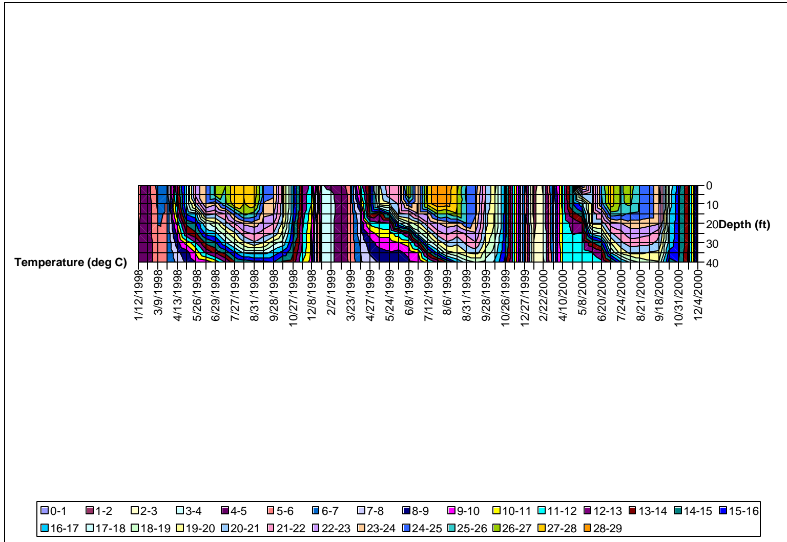
Figure A11: Isothermal Contours, Loch Raven Reservoir, Lower Sampling Locations, 1998-2000
