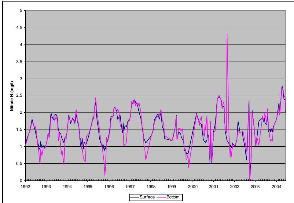
Figure A43: Average Nitrate Nitrogen. Lower Sampling Location, Loch Raven Reservoir.
