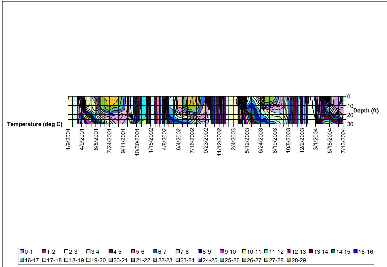
Figure A20: Isothermal Contours, Loch Raven Reservoir, Upper Sampling Location, 2001-2004
