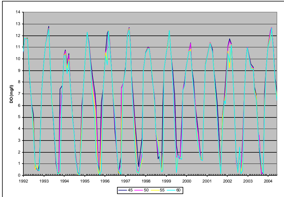
Figure A21: Average Bottom Dissolved Oxygen. Lower Sampling Locations, Prettyboy Reservoir
