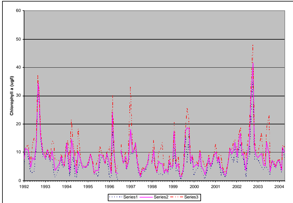
Figure A47: Surface Chlorophyll a. Middle Sampling Location, Prettyboy Reservoir.
