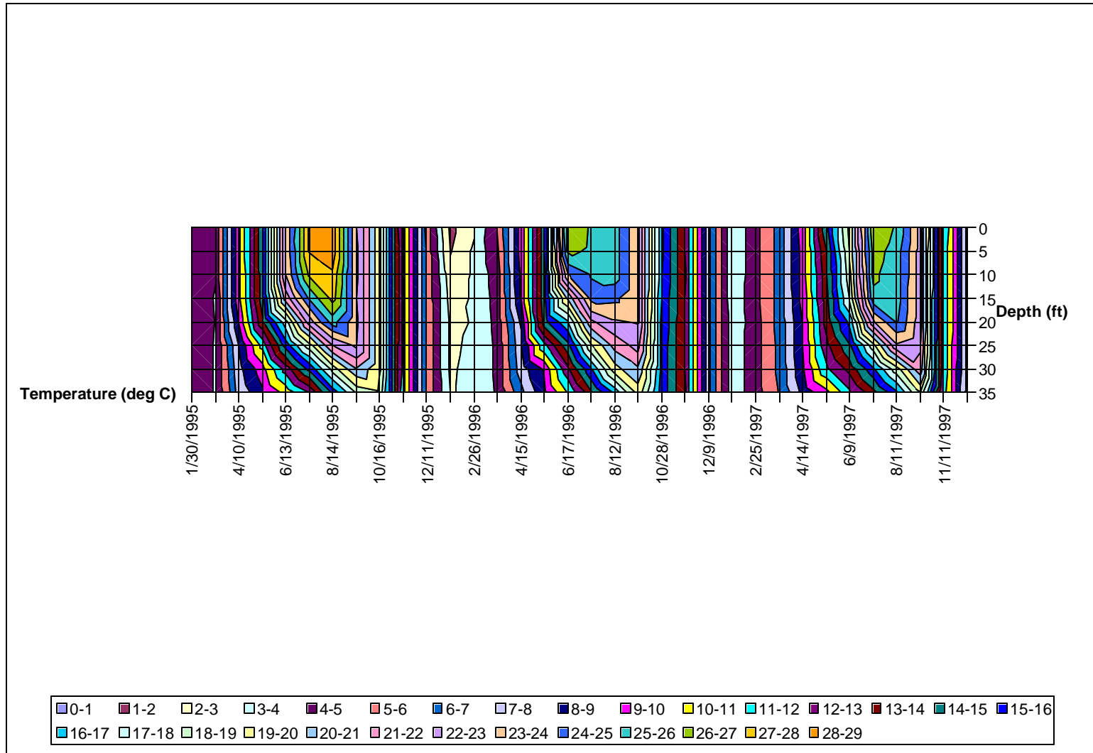
Figure A6: Isothermal Contours, Prettyboy Reservoir, Middle Sampling Location, 1995-1997
