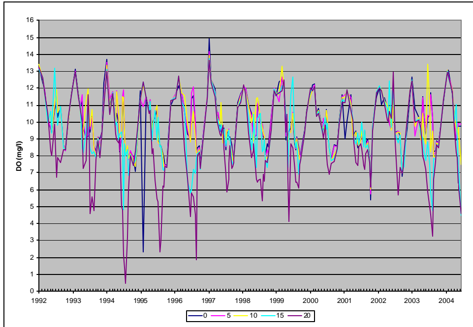
Figure A29: Average Surface Dissolved Oxygen. Middle Sampling Locations, Loch Raven Reservoir.
