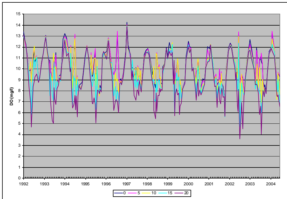
Figure A30: Average Surface Dissolved Oxygen. Upper Sampling Locations, Loch Raven Reservoir.
