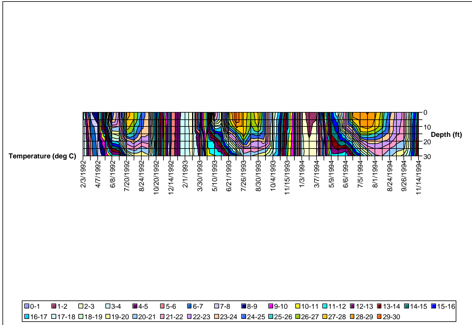
Figure A17: Isothermal Contours, Loch Raven Reservoir, Upper Sampling Location, 1992-1994
