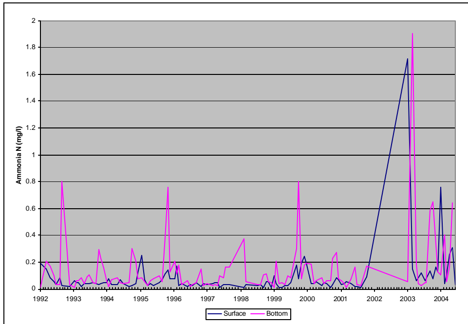
Figure A37: Average Ammonia Nitrogen. Middle Sampling Location, Prettyboy Reservoir.
