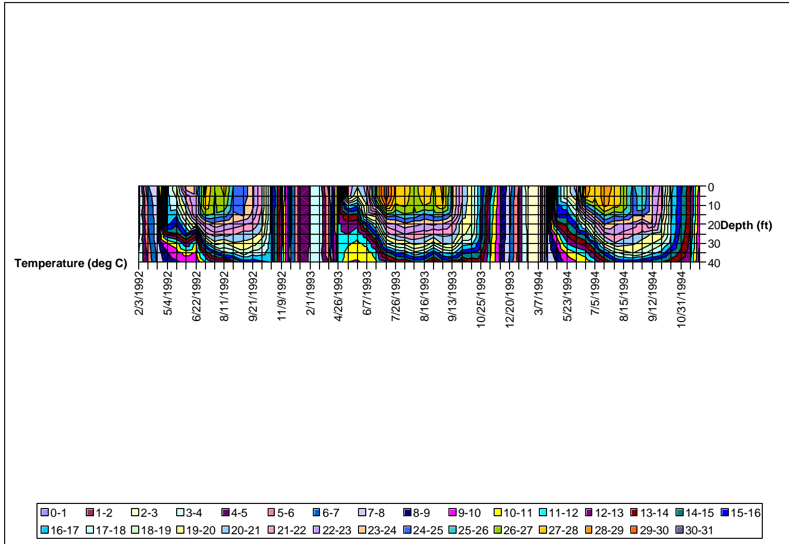
Figure A9: Isothermal Contours, Loch Raven Reservoir, Lower Sampling Locations, 1992-1994
