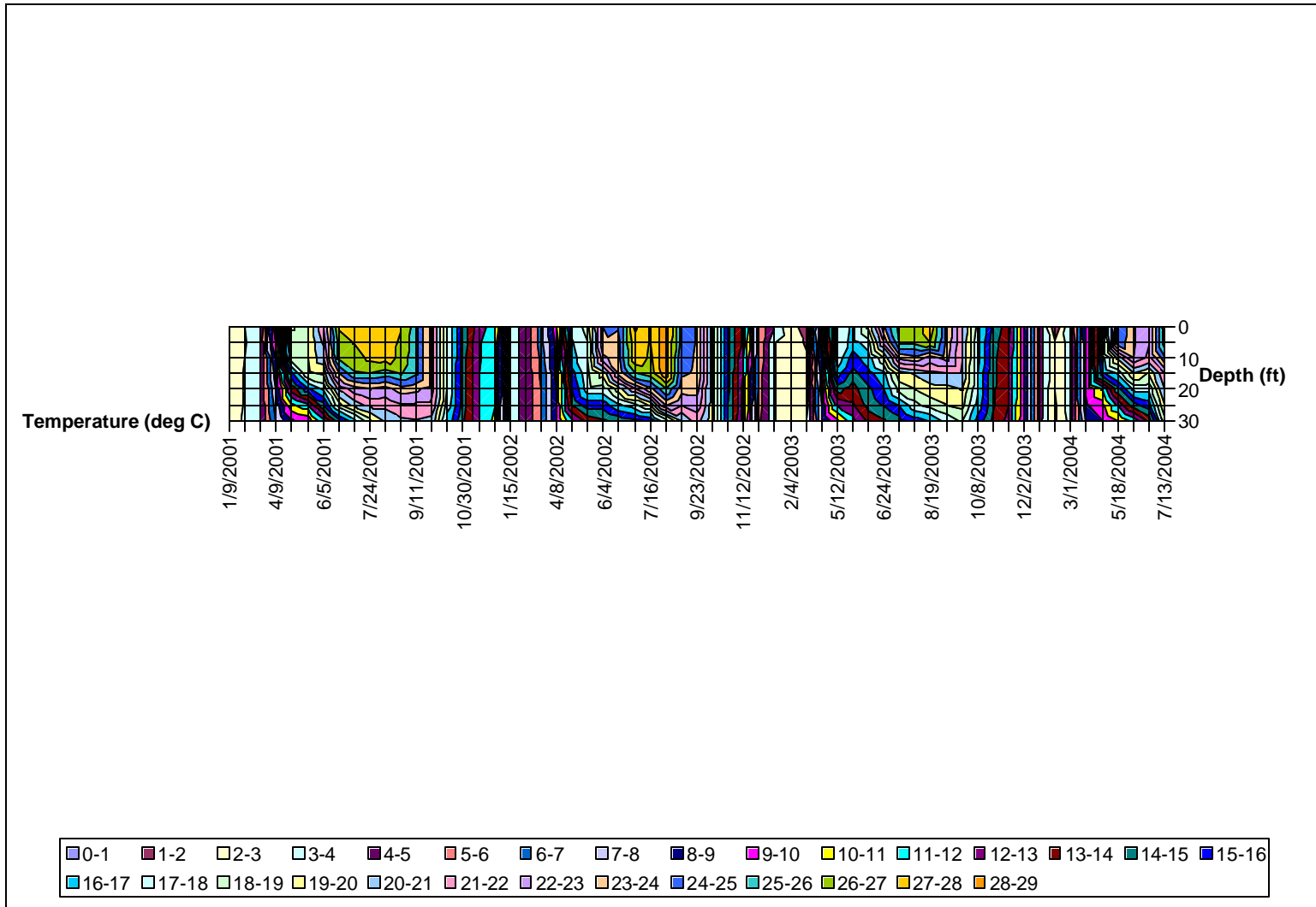
Figure A16: Isothermal Contours, Loch Raven Reservoir, Middle Sampling Location, 2001-2004
