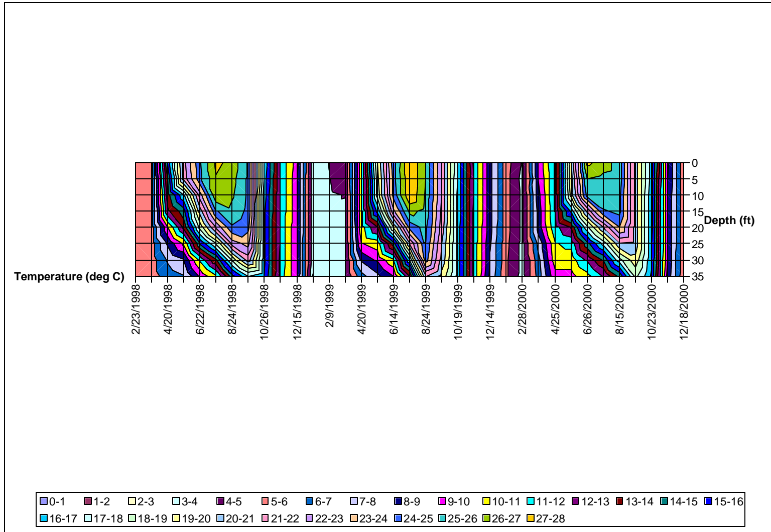
Figure A7: Isothermal Contours, Prettyboy Reservoir, Middle Sampling Location, 1998-2000
