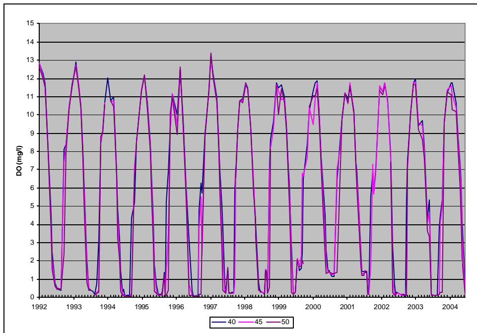
Figure A24: Average Bottom Dissolved Oxygen. Middle Sampling Locations, Loch Raven Reservoir.
