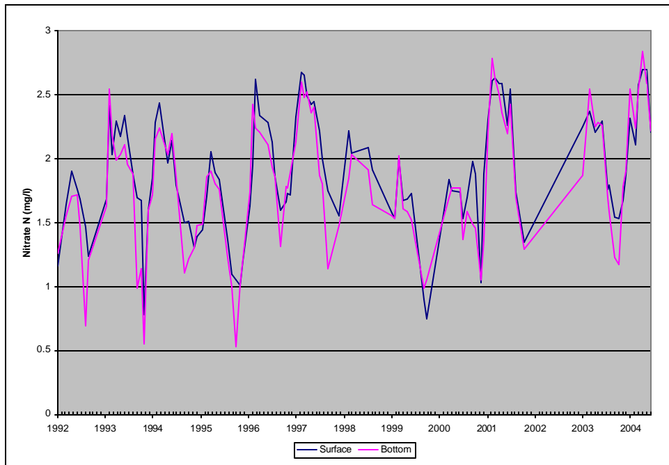
Figure A42: Average Nitrate Nitrogen. Middle Sampling Location, Prettyboy Reservoir.
