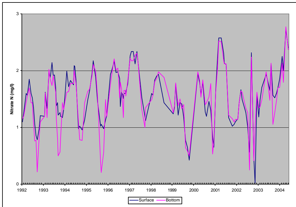
Figure A44: Average Nitrate Nitrogen. Middle Sampling Locations, Loch Raven Reservoir.
