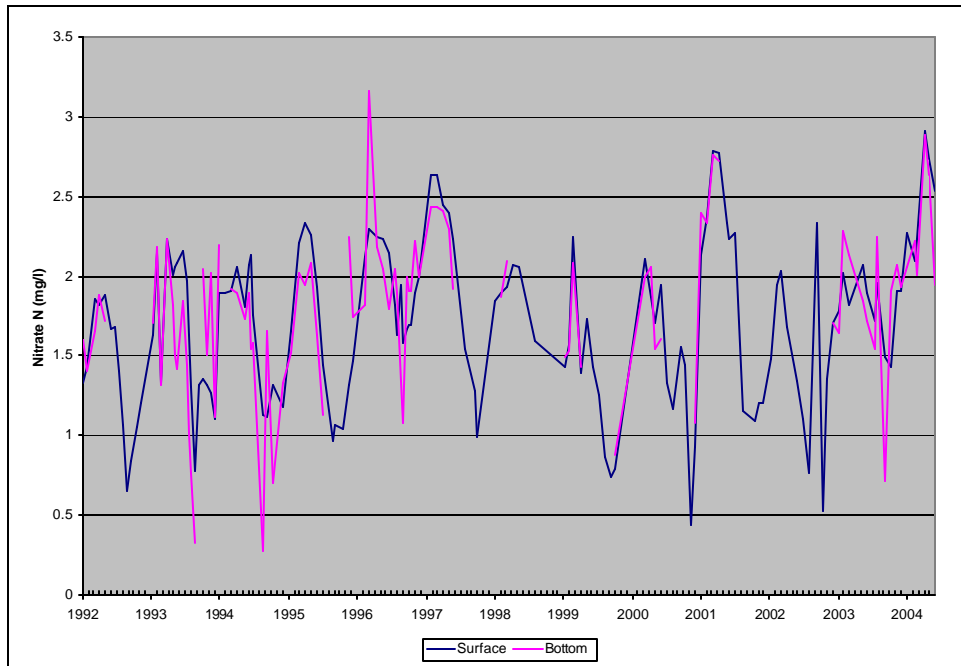
Figure A45: Average Nitrate Nitrogen. Upper Sampling Locations, Loch Raven Reservoir.
