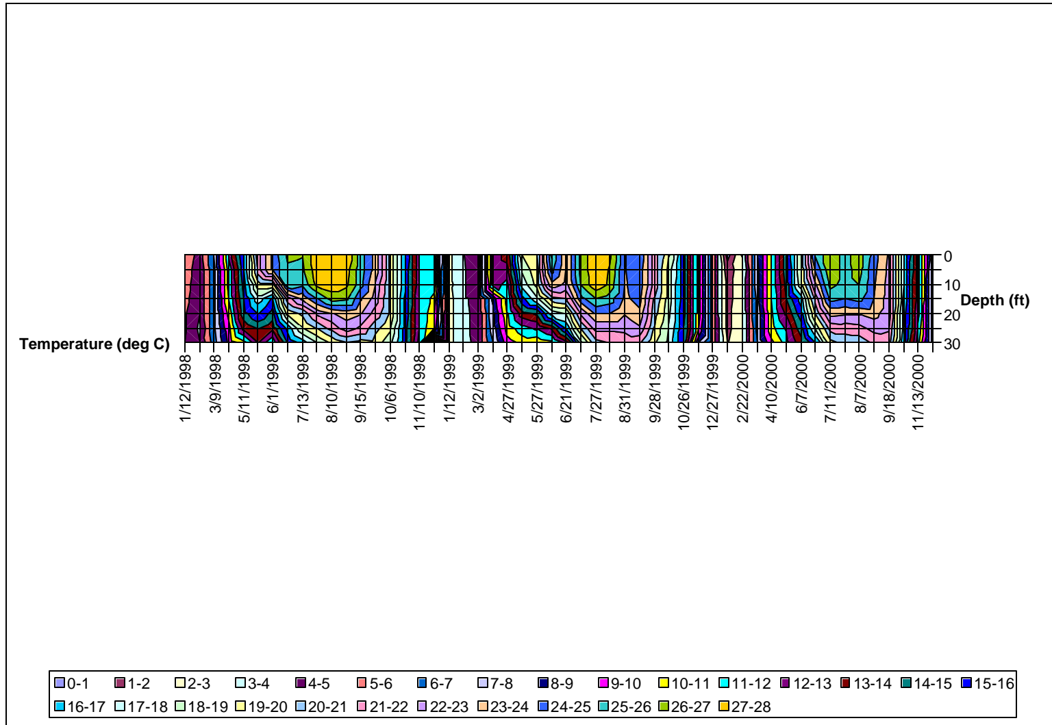
Figure A19: Isothermal Contours, Loch Raven Reservoir, Upper Sampling Location, 1998-2000
