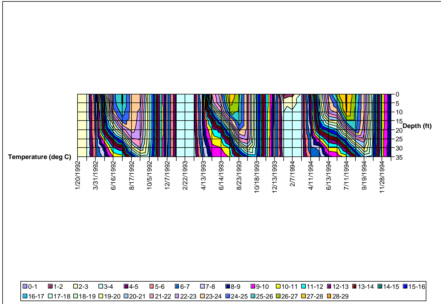
Figure A5: Isothermal Contours, Prettyboy Reservoir, Middle Sampling Location, 1992-1994
