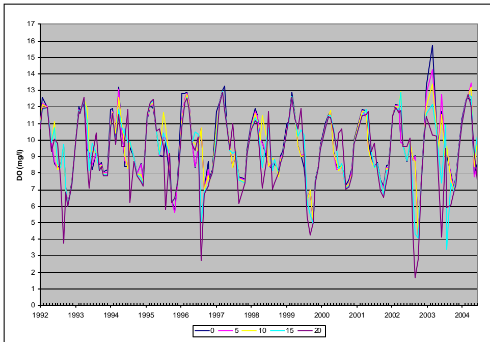
Figure A26: Average Surface Dissolved Oxygen. Lower Sampling Locations, Prettyboy Reservoir.
