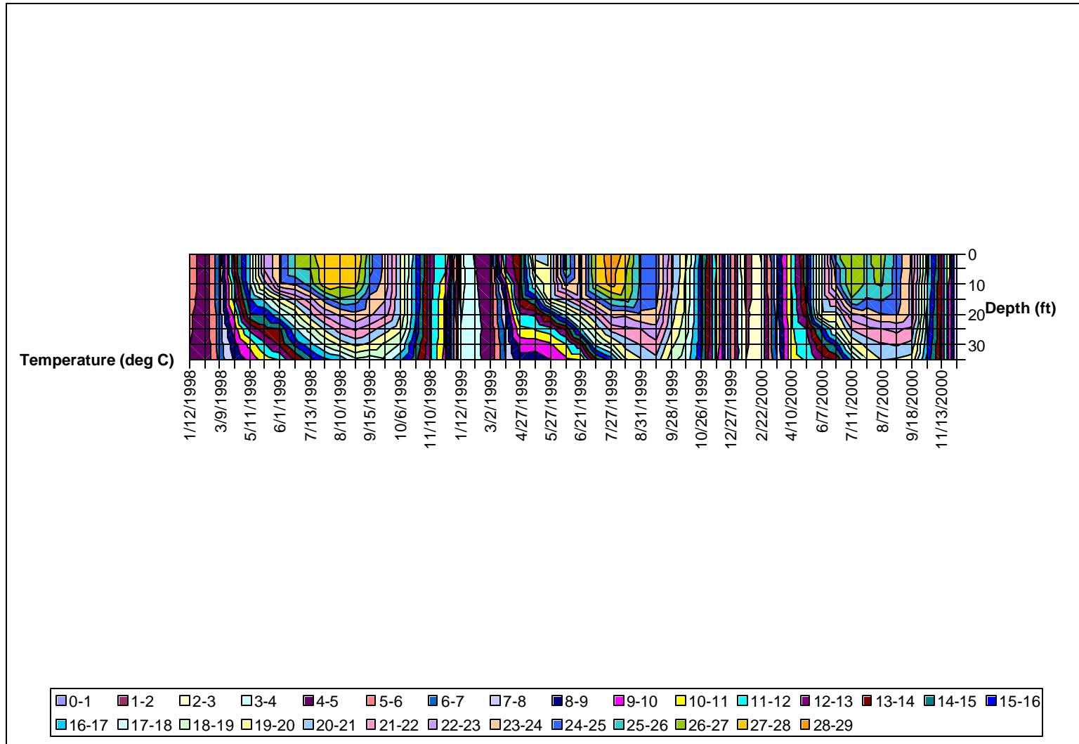
Figure A15: Isothermal Contours, Loch Raven Reservoir, Middle Sampling Location, 1998-2000
