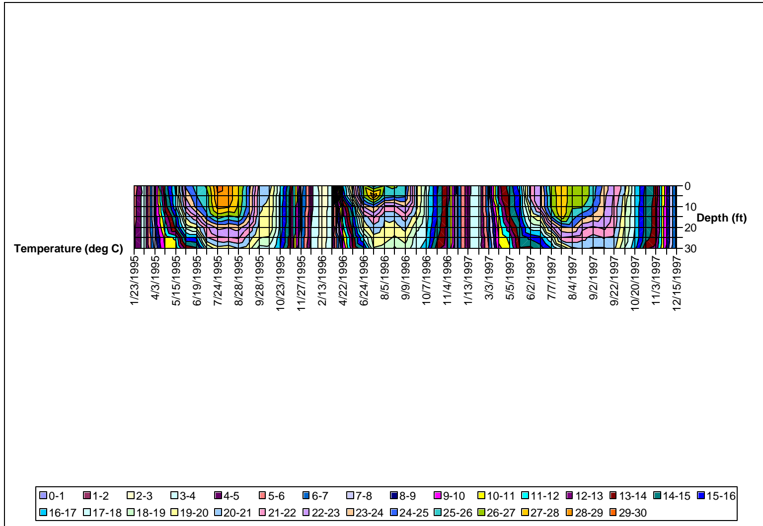
Figure A18: Isothermal Contours, Loch Raven Reservoir, Upper Sampling Location, 1995-1997
