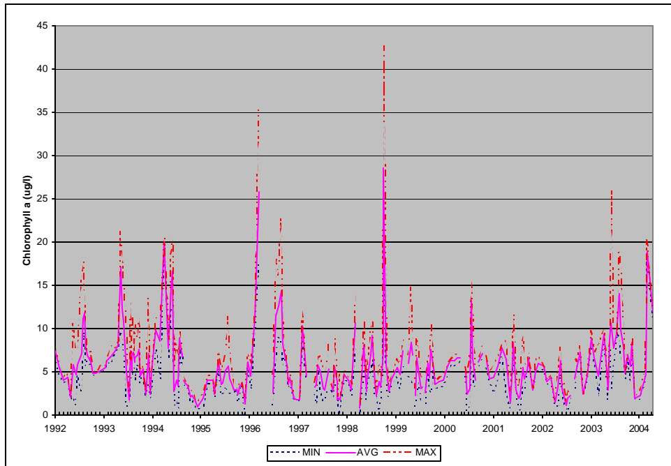
Figure A48: Surface Chlorophyll a. Lower Sampling Location, Loch Raven Reservoir.
