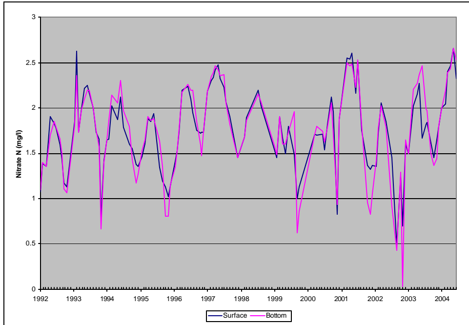
Figure A41: Average Nitrate Nitrogen. Lower Sampling Locations, Prettyboy Reservoir.
