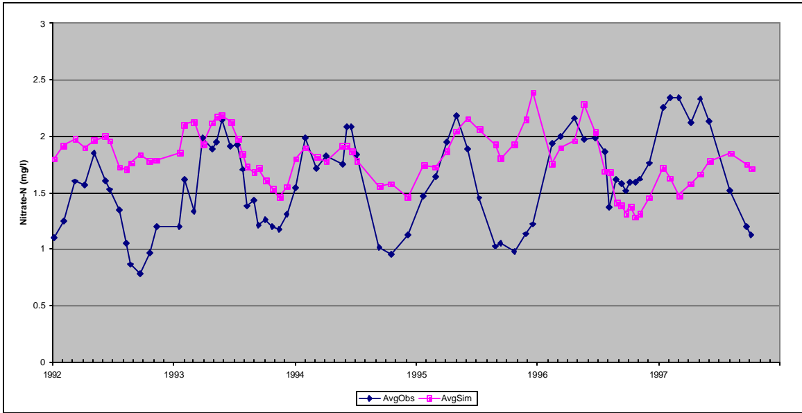
Figure C27: Observed and Simulated Average Surface Nitrate Concentrations, Middle Station, Calibration Scenario, Loch Raven Reservoir.
