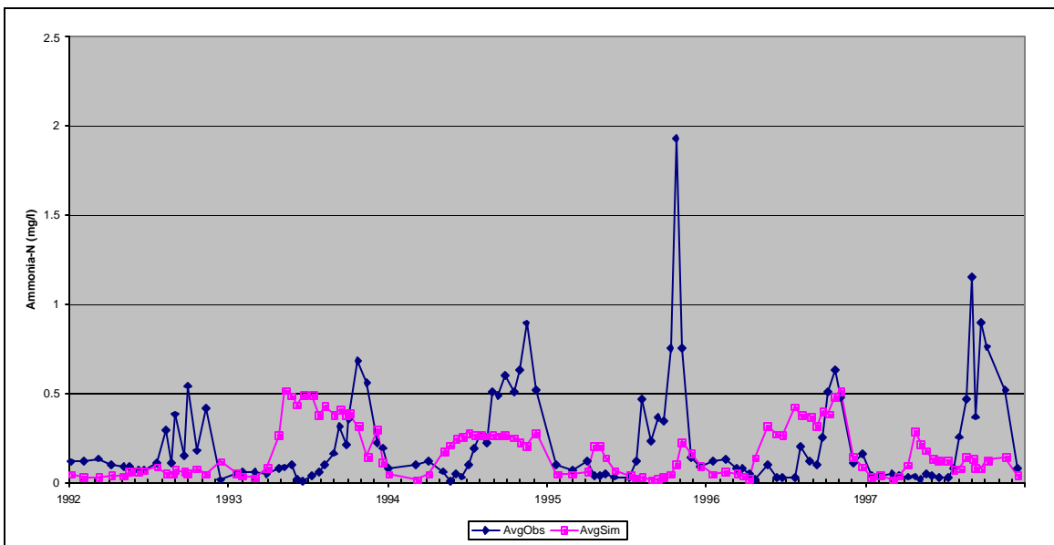
Figure C24: Observed and Simulated Average Bottom Ammonia Concentrations, Lower Station, Calibration Scenario, Loch Raven Reservoir.
