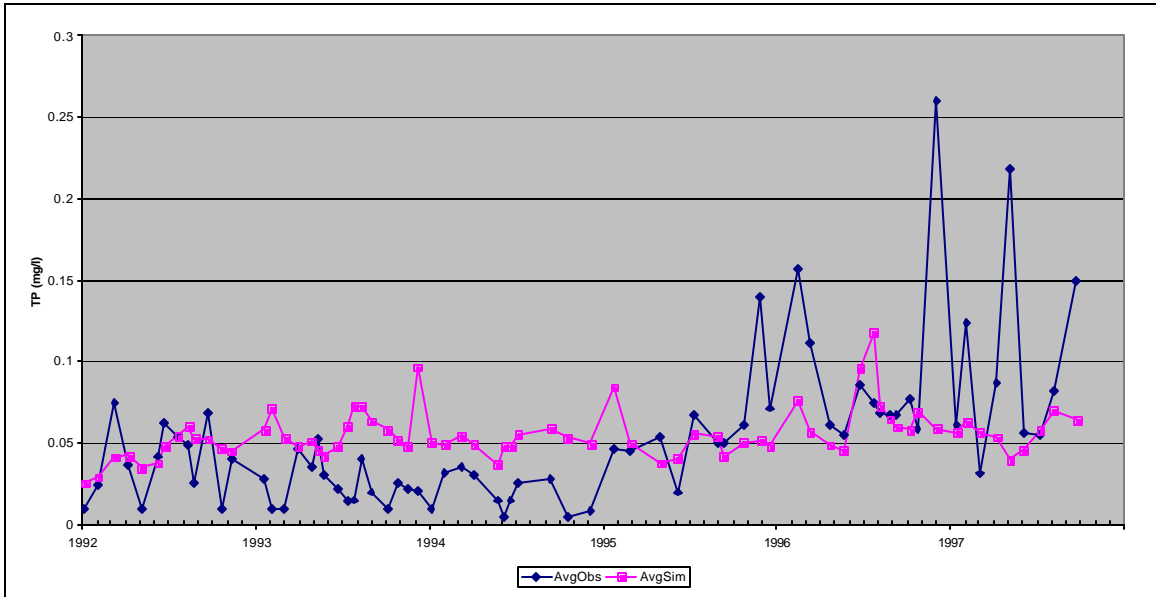
Figure C15: Observed and Simulated Total Average Surface Phosphorus Concentrations, Middle Station, Calibration Scenario, Loch Raven Reservoir.
