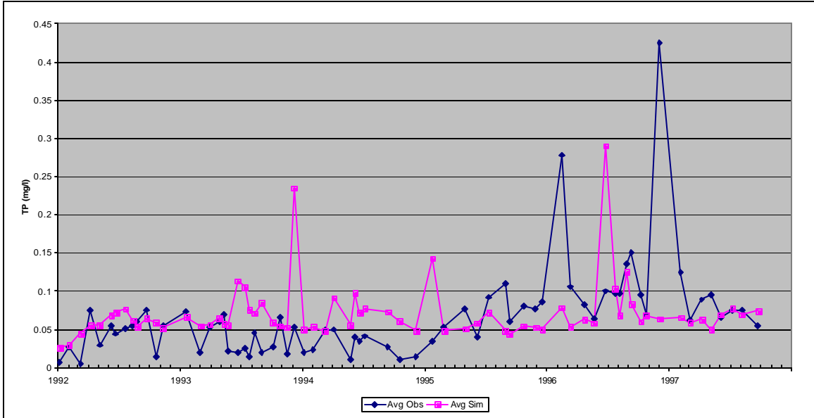
Figure C13: Observed and Simulated Total Average Surface Phosphorus Concentrations, Upper Station, Calibration Scenario, Loch Raven Reservoir.
