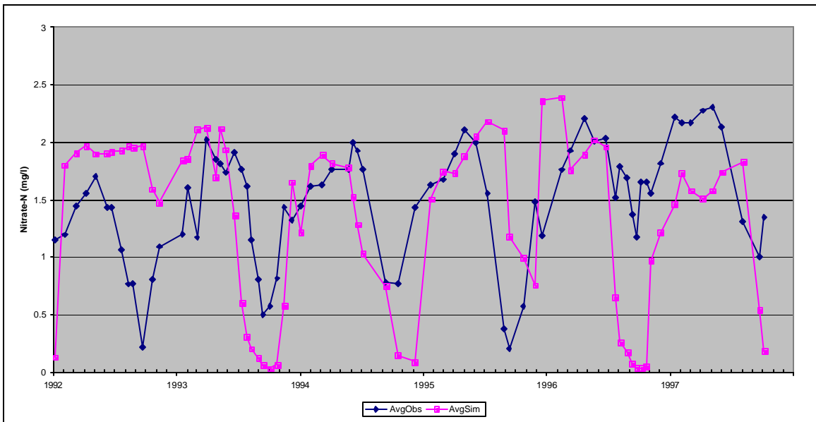
Figure C28: Observed and Simulated Average Bottom Nitrate Concentrations, Middle Station, Calibration Scenario, Loch Raven Reservoir.
