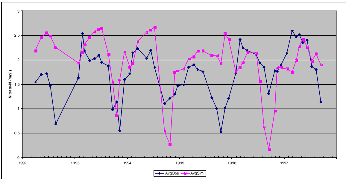
Figure C10: Observed and Simulated Average Bottom Nitrate Concentrations, Middle Station, Calibration Scenario, Prettyboy Reservoir.
