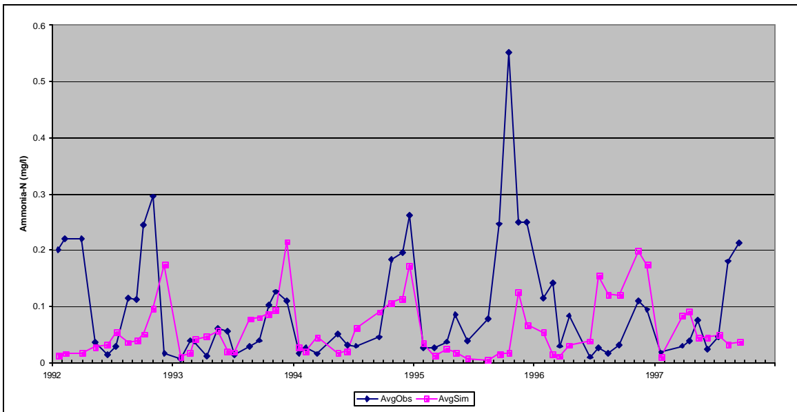
Figure C8: Observed and Simulated Average Bottom Ammonia Concentrations, Lower Station, Calibration Scenario, Prettyboy Reservoir.
