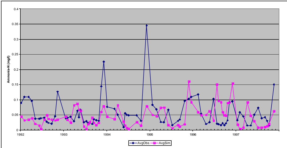
Figure C21: Observed and Simulated Average Surface Ammonia Concentrations, Middle Station, Calibration Scenario, Loch Raven Reservoir.
