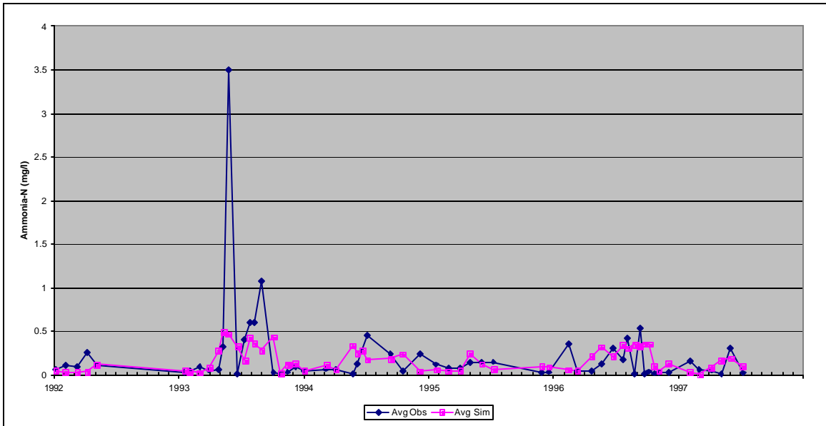
Figure C20: Observed and Simulated Average Bottom Ammonia Concentrations, Upper Station, Calibration Scenario, Loch Raven Reservoir.
