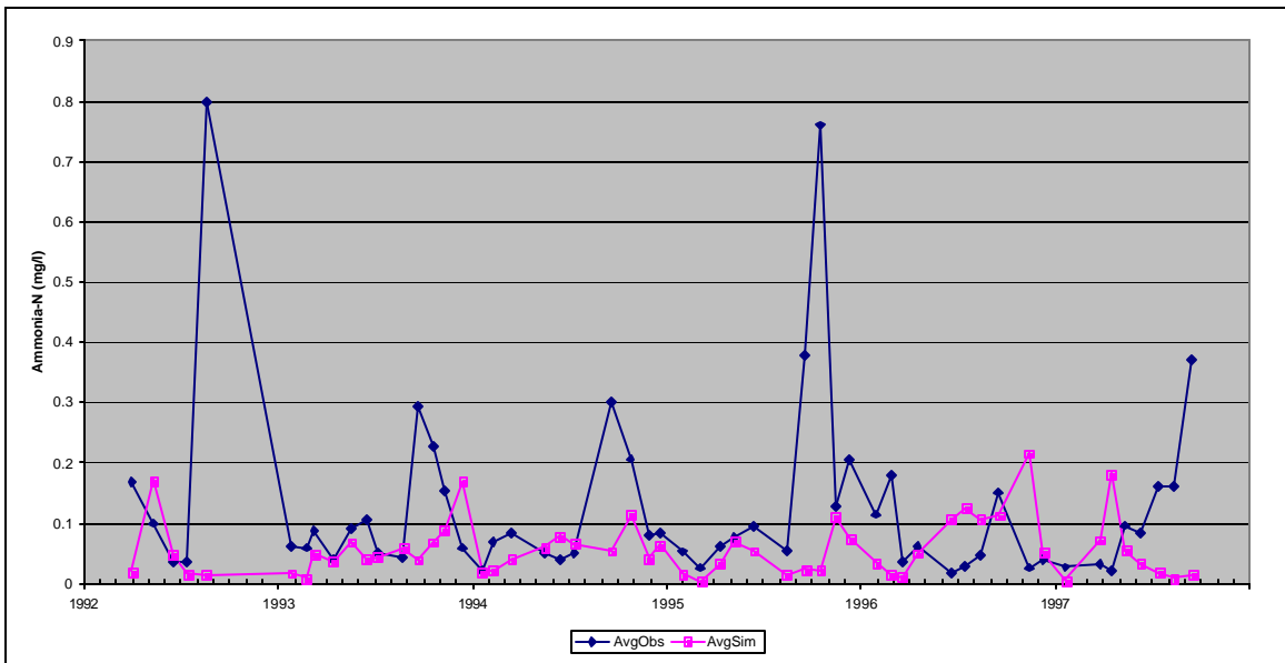
Figure C6: Observed and Simulated Average Bottom Ammonia Concentrations, Middle Station, Calibration Scenario, Prettyboy Reservoir.
