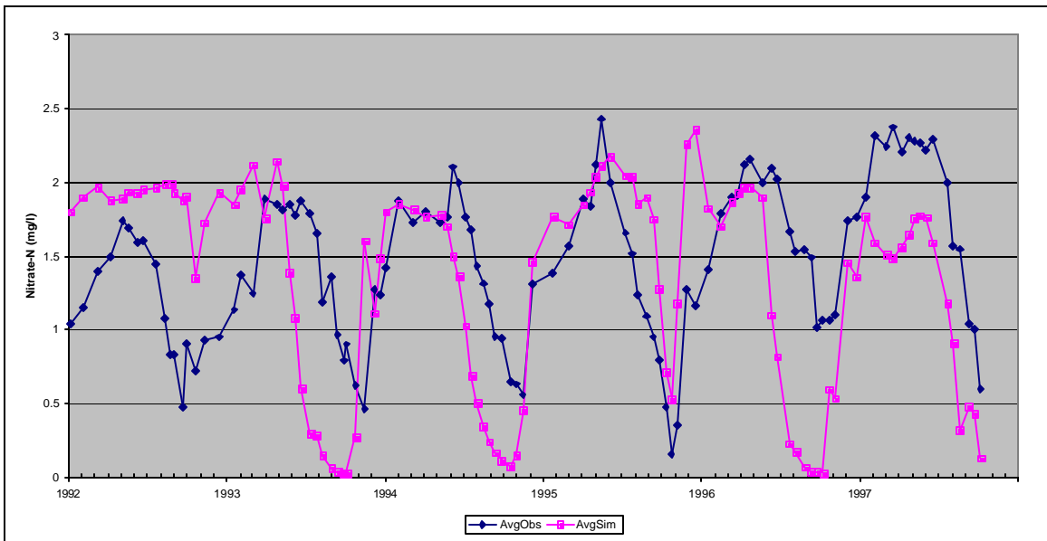
Figure C30: Observed and Simulated Average Bottom Nitrate Concentrations, Lower Station, Calibration Scenario, Loch Raven Reservoir.
