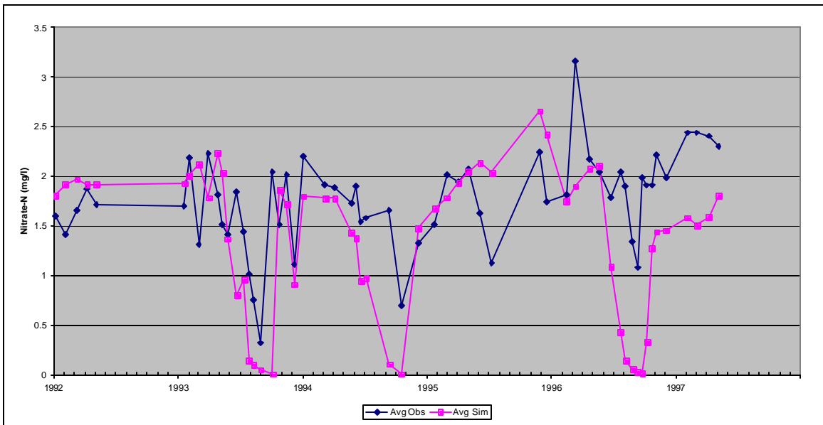
Figure C26: Observed and Simulated Average Bottom Nitrate Concentrations, Upper Station, Calibration Scenario, Loch Raven Reservoir.
