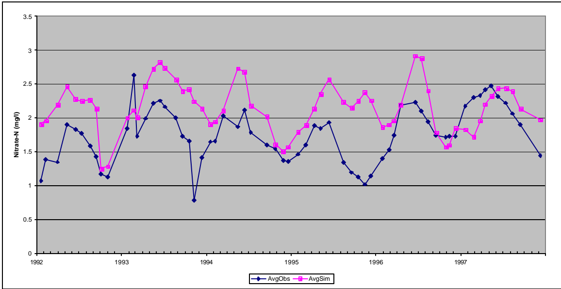
Figure C11: Observed and Simulated Average Surface Nitrate Concentrations, Lower Station, Calibration Scenario, Prettyboy Reservoir.
