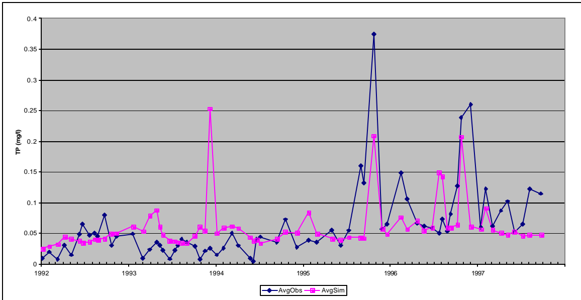
Figure C16: Observed and Simulated Total Average Bottom Phosphorus Concentrations, Middle Station, Calibration Scenario, Loch Raven Reservoir.
