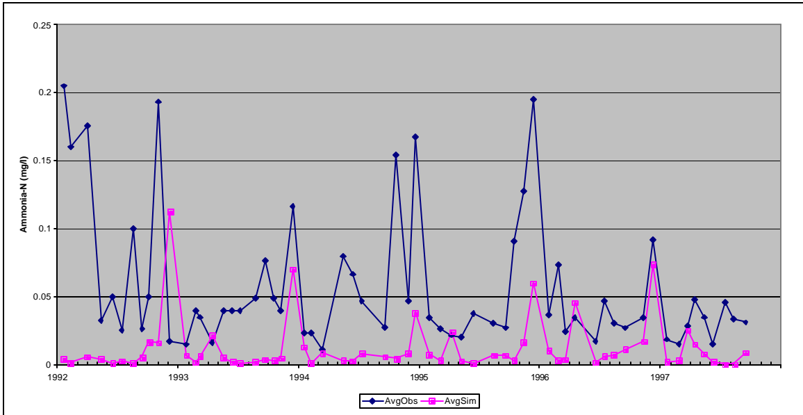
Figure C7: Observed and Simulated Average Surface Ammonia Concentrations, Lower Station, Calibration Scenario, Prettyboy Reservoir.
