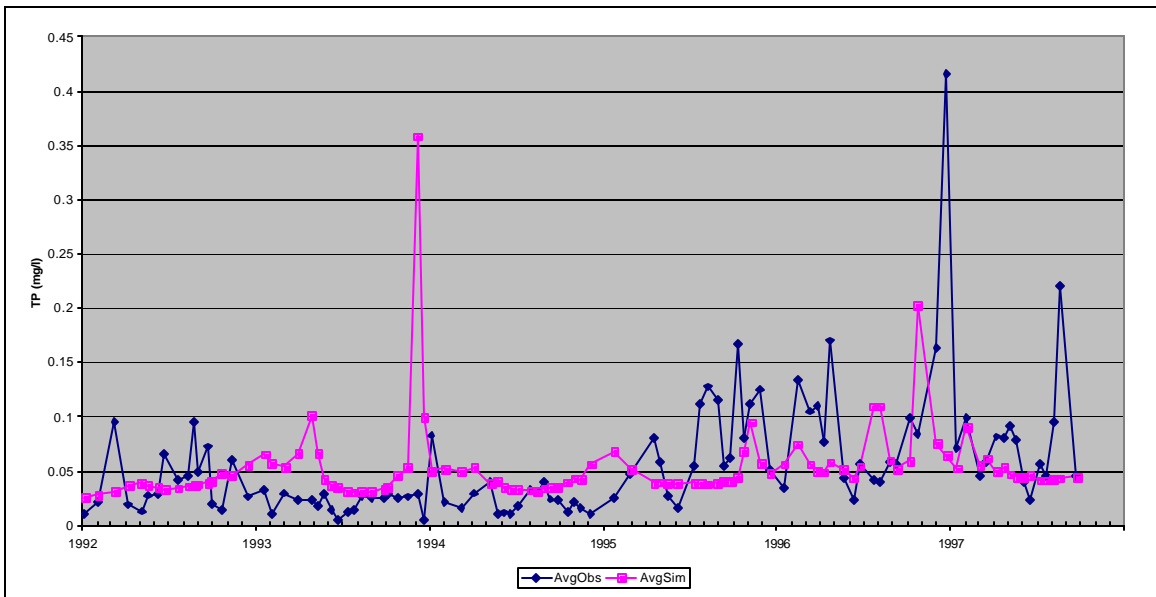
Figure C18: Observed and Simulated Total Average Bottom Phosphorus Concentrations, Lower Station, Calibration Scenario, Loch Raven Reservoir.
