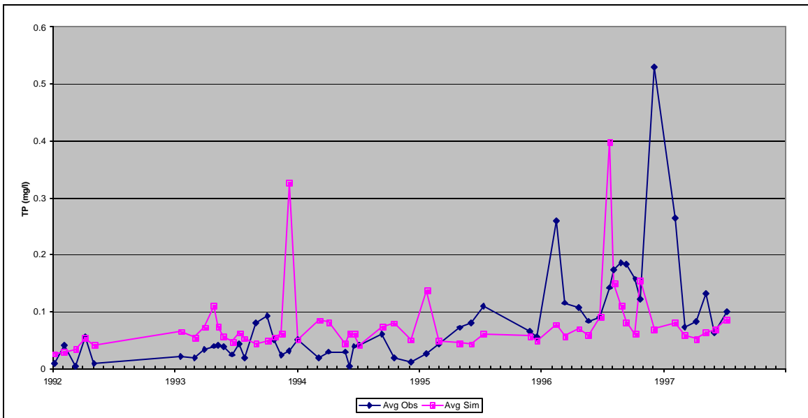
Figure C14: Observed and Simulated Total Average Bottom Phosphorus Concentrations, Upper Station, Calibration Scenario, Loch Raven Reservoir.
