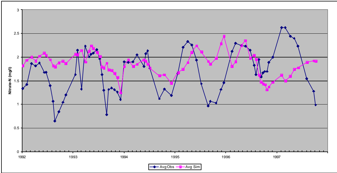
Figure C25: Observed and Simulated Average Surface Nitrate Concentrations, Upper Station, Calibration Scenario, Loch Raven Reservoir.
