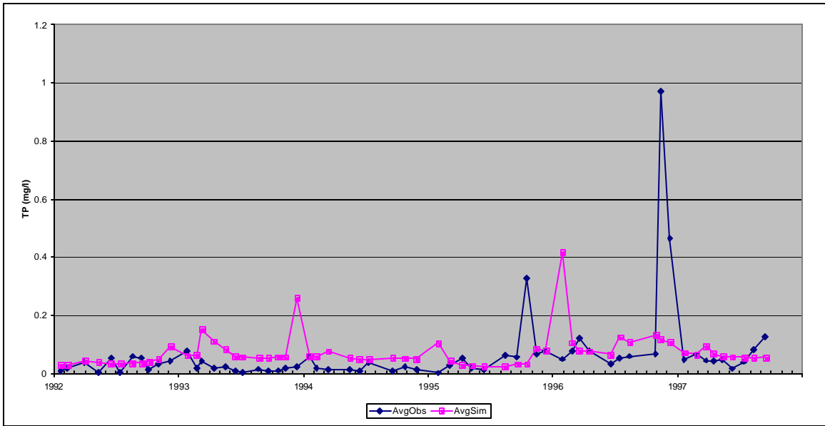
Figure C4: Observed and Simulated Average Bottom Total Phosphorus Concentrations, Lower Station, Calibration Scenario, Prettyboy Reservoir.
