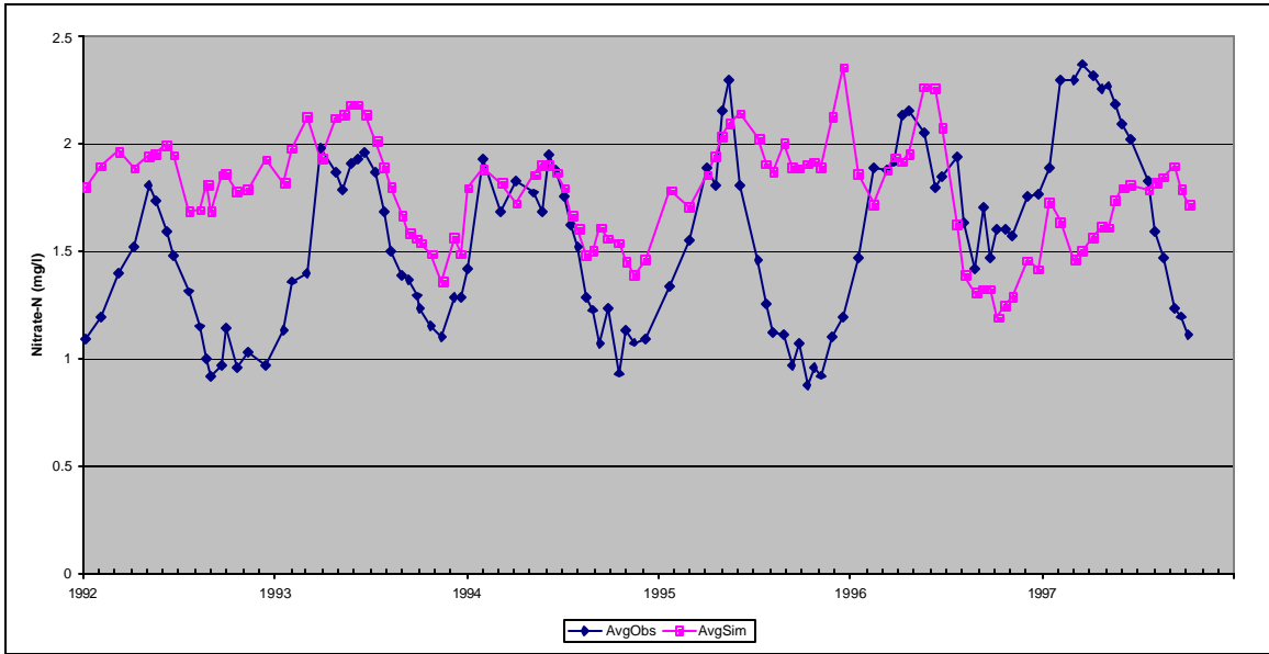
Figure C29: Observed and Simulated Average Surface Nitrate Concentrations, Lower Station, Calibration Scenario, Loch Raven Reservoir.
