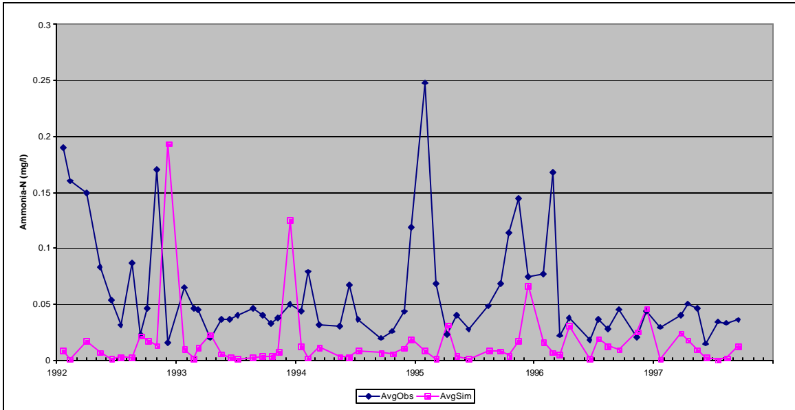
Figure C5: Observed and Simulated Average Surface Ammonia Concentrations, Middle Station, Calibration Scenario, Prettyboy Reservoir.
