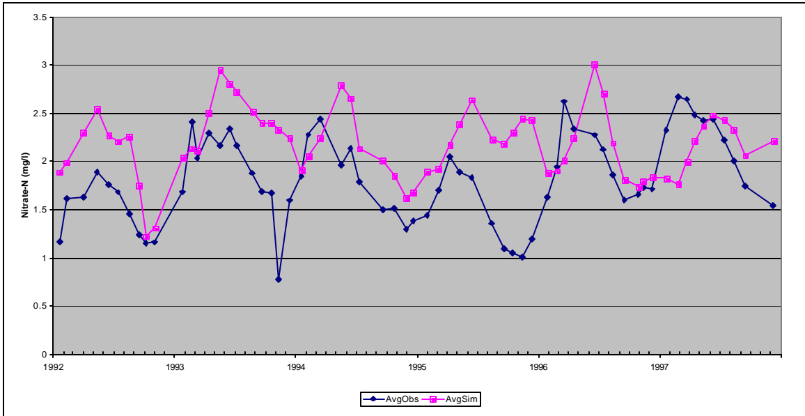
Figure C9: Observed and Simulated Average Surface Nitrate Concentrations, Middle Station, Calibration Scenario, Prettyboy Reservoir.
