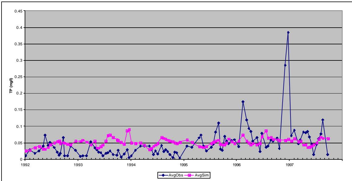
Figure C17: Observed and Simulated Total Average Surface Phosphorus Concentrations, Lower Station, Calibration Scenario, Loch Raven Reservoir.
