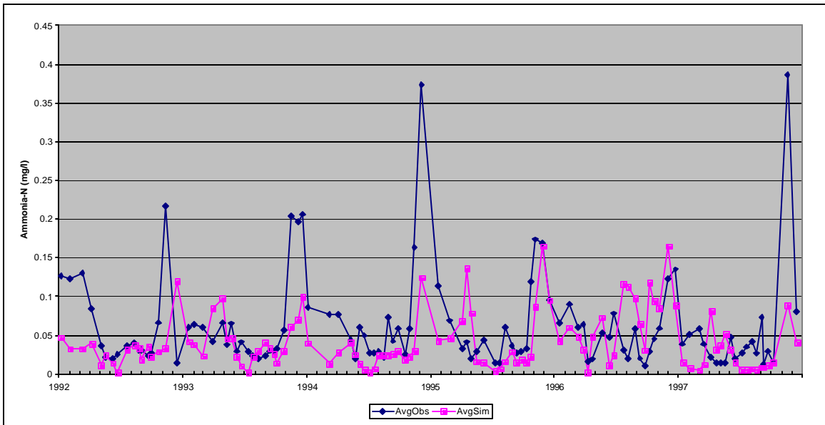
Figure C23: Observed and Simulated Average Surface Ammonia Concentrations, Lower Station, Calibration Scenario, Loch Raven Reservoir.
