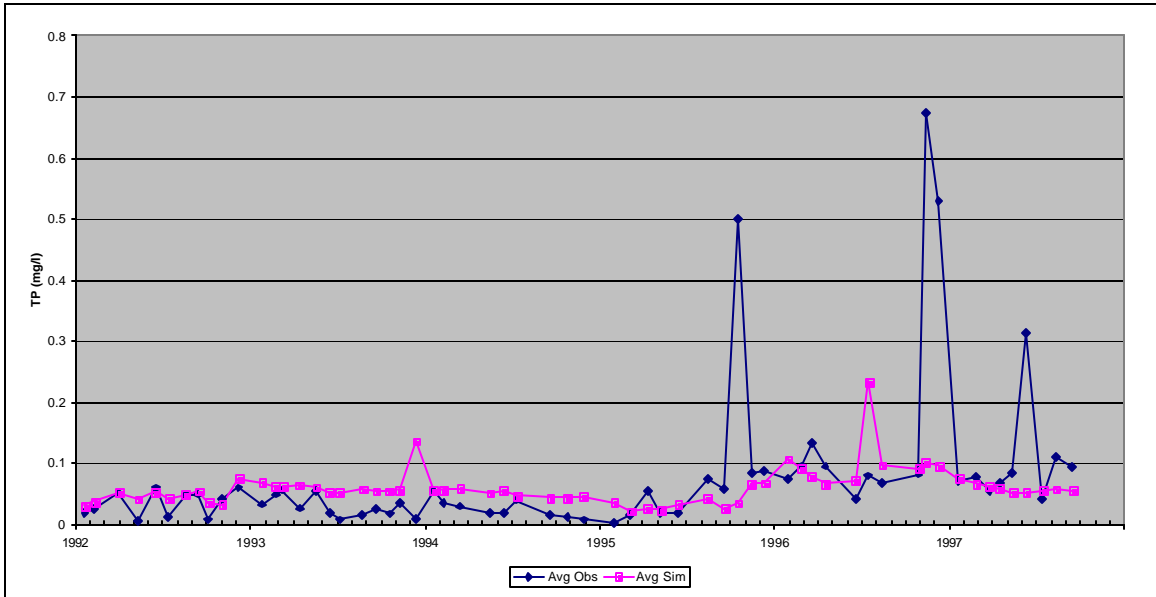
Figure C1: Observed and Simulated Average Surface Total Phosphorus Concentrations, Middle Station, Calibration Scenario, Prettyboy Reservoir.
