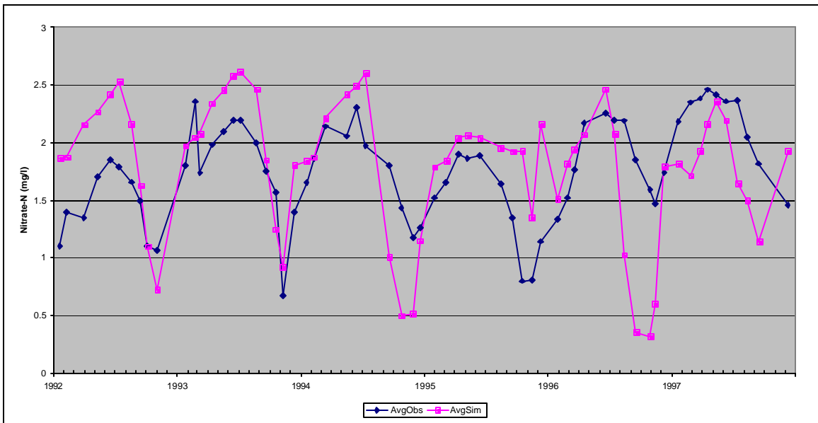
Figure C12: Observed and Simulated Average Bottom Nitrate Concentrations, Lower Station, Calibration Scenario, Prettyboy Reservoir.
