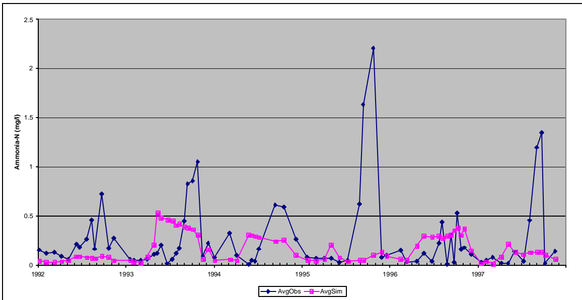
Figure C22: Observed and Simulated Average Bottom Ammonia Concentrations, Middle Station, Calibration Scenario, Loch Raven Reservoir.
