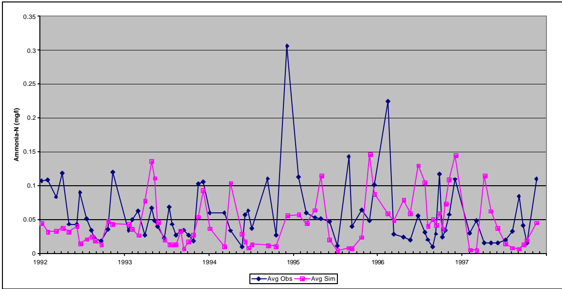
Figure C19: Observed and Simulated Average Surface Ammonia Concentrations, Upper Station, Calibration Scenario, Loch Raven Reservoir.
