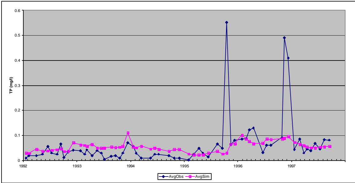
Figure C3: Observed and Simulated Average Surface Total Phosphorus Concentrations, Lower Station, Calibration Scenario, Prettyboy Reservoir.
