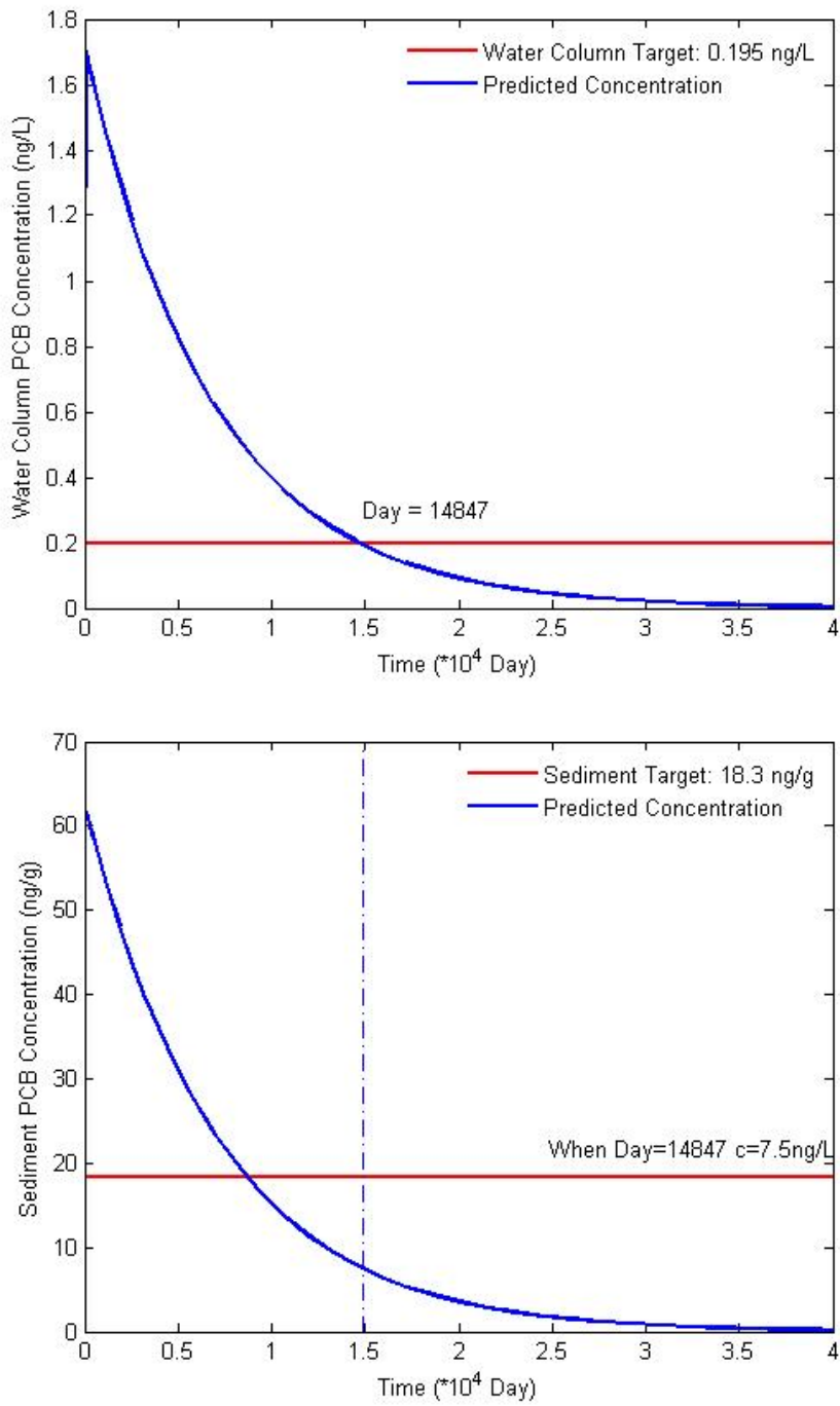
Figure 7: Change of Average Water Column and Bottom Sediment tPCB Concentrations with Time within the Severn River (100% Reduction to Watershed Load, WWTP load, & Atmospheric Deposition)
