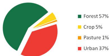
Land use in the South River watershed
