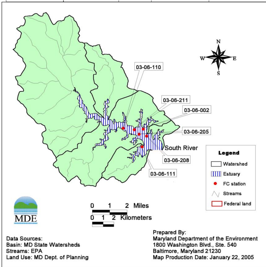
Figure 2.2.1: Shellfish Monitoring Stations in South River
