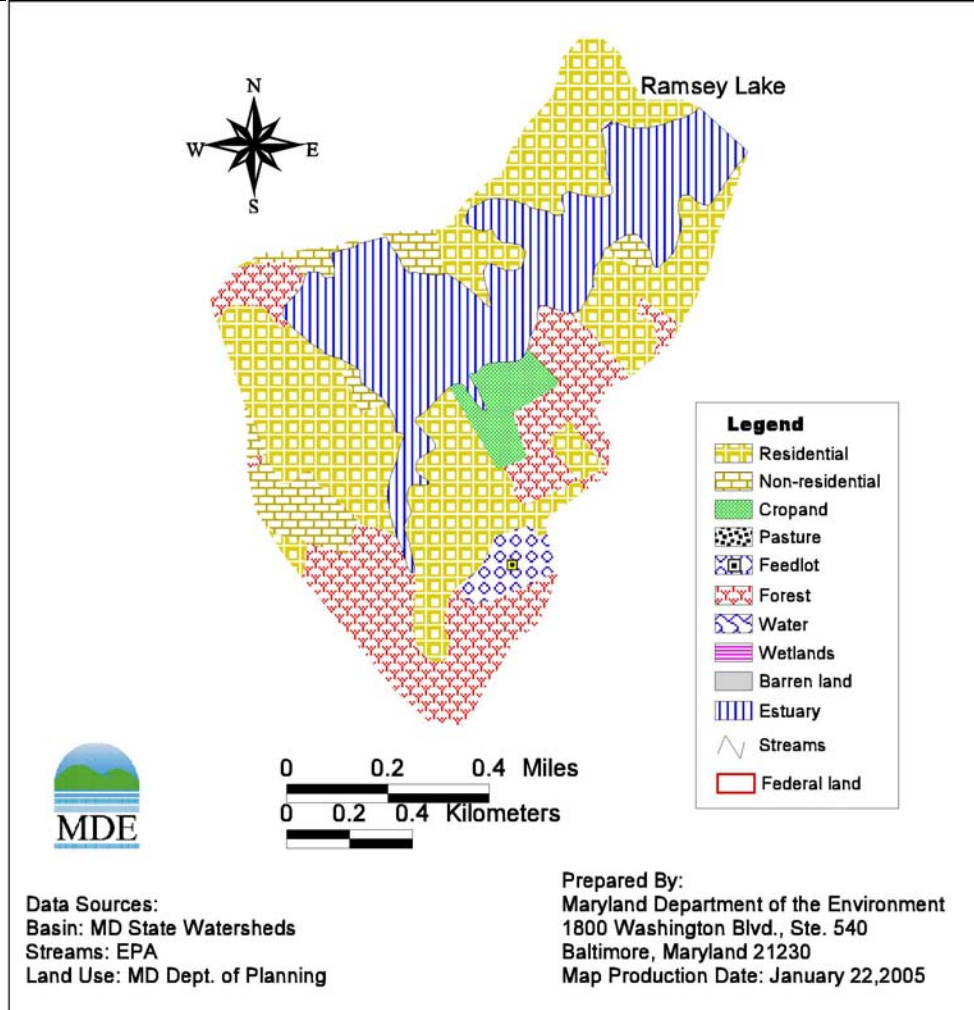
Figure 2.1.5: Land Use in the Ramsey Lake Watershed
