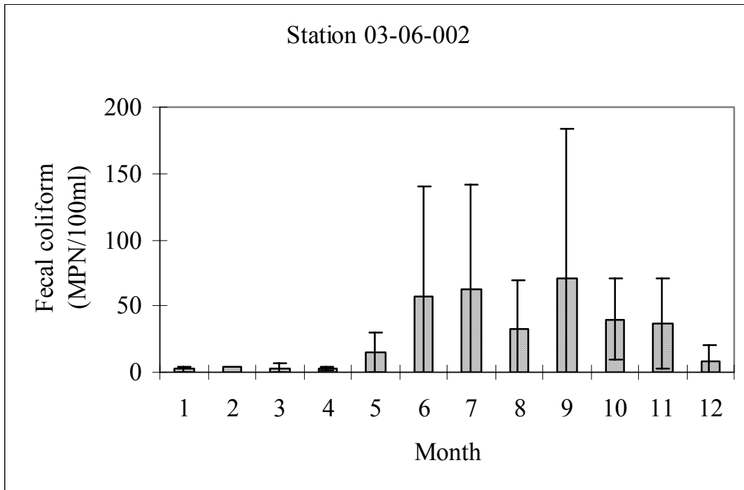
Figure E-3: Seasonality analysis of fecal coliform at South River Station 03-06-002
