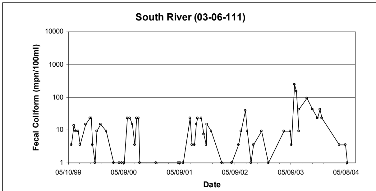
Figure 2.2.7: Observed Fecal Coliform Concentrations at Station 03-06-111
