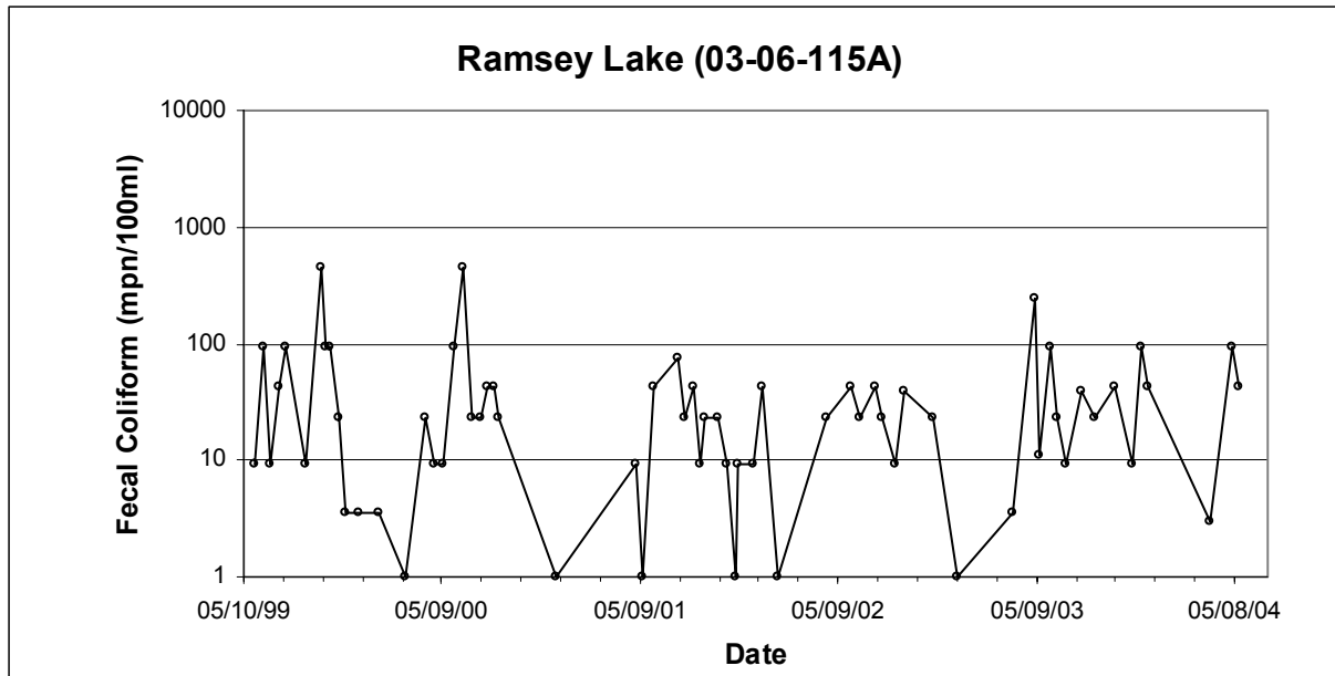
Figure 2.2.15: Observed Fecal Coliform Concentrations at Station 03-06-115A
