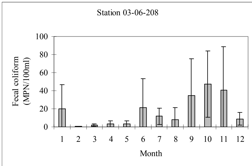
Figure E-5: Seasonality analysis of fecal coliform at South River Station 03-06-208
