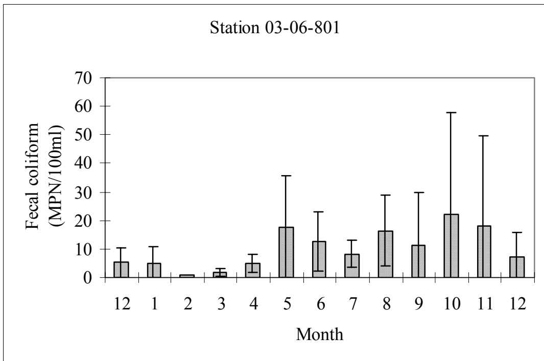
Figure E-9: Seasonality analysis of fecal coliform at Selby Bay Station 03-06-801
