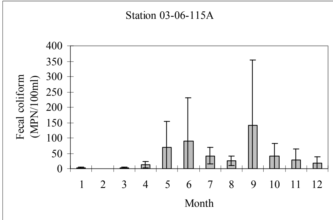
Figure E-11: Seasonality analysis of fecal coliform at Ramsey Lake Station 03-06-115A
