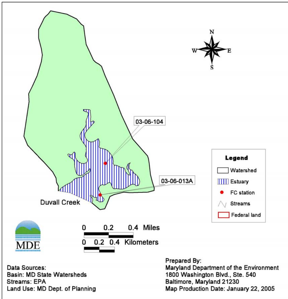
Figure 2.2.8: Shellfish Monitoring Stations in Duvall Creek
