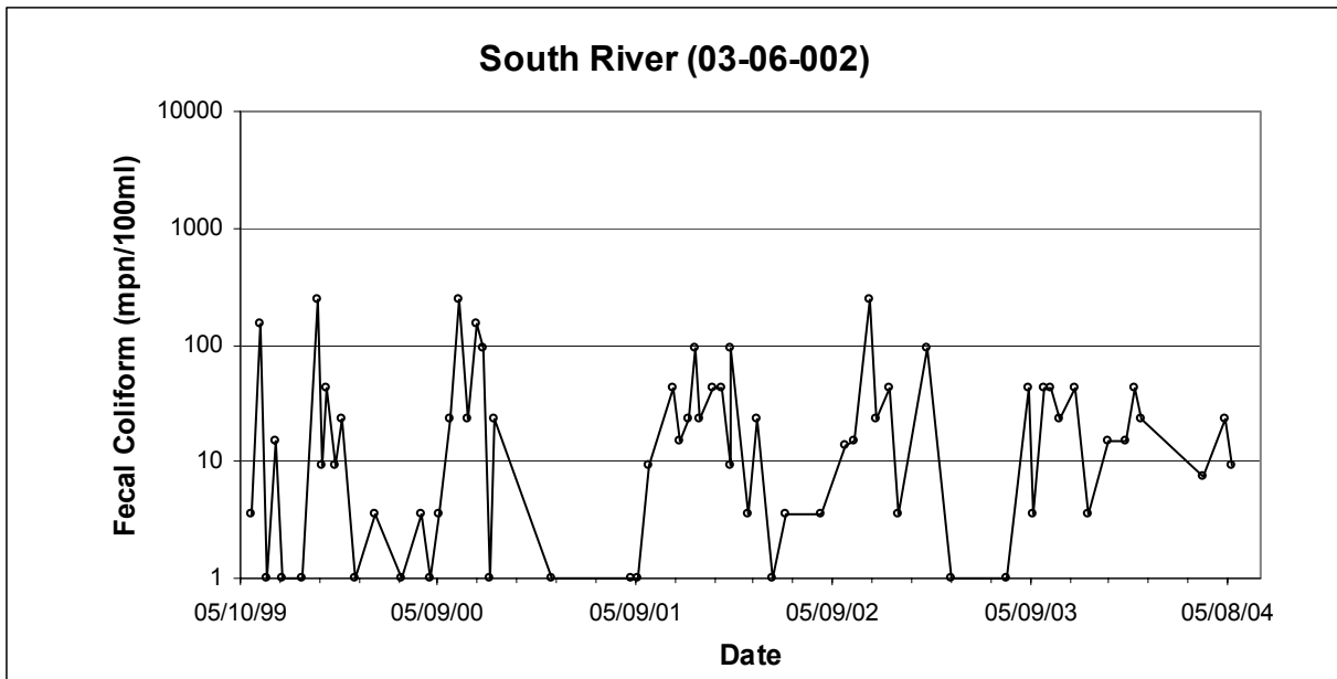
Figure 2.2.4: Observed Fecal Coliform Concentrations at Station 03-06-002
