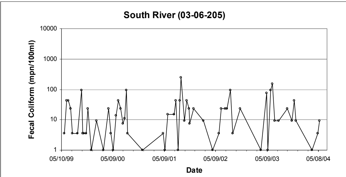
Figure 2.2.5: Observed Fecal Coliform Concentrations at Station 03-06-205
