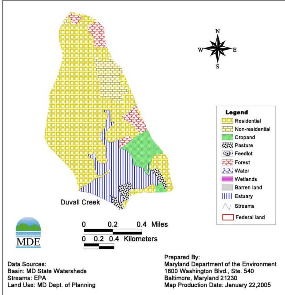
Figure 2.1.3: Land Use in the Duvall Creek Basin
