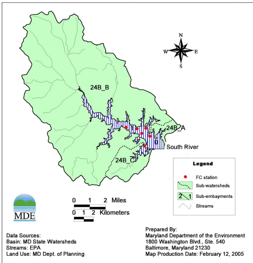
Figure B-1: Delineation for South River Basin
