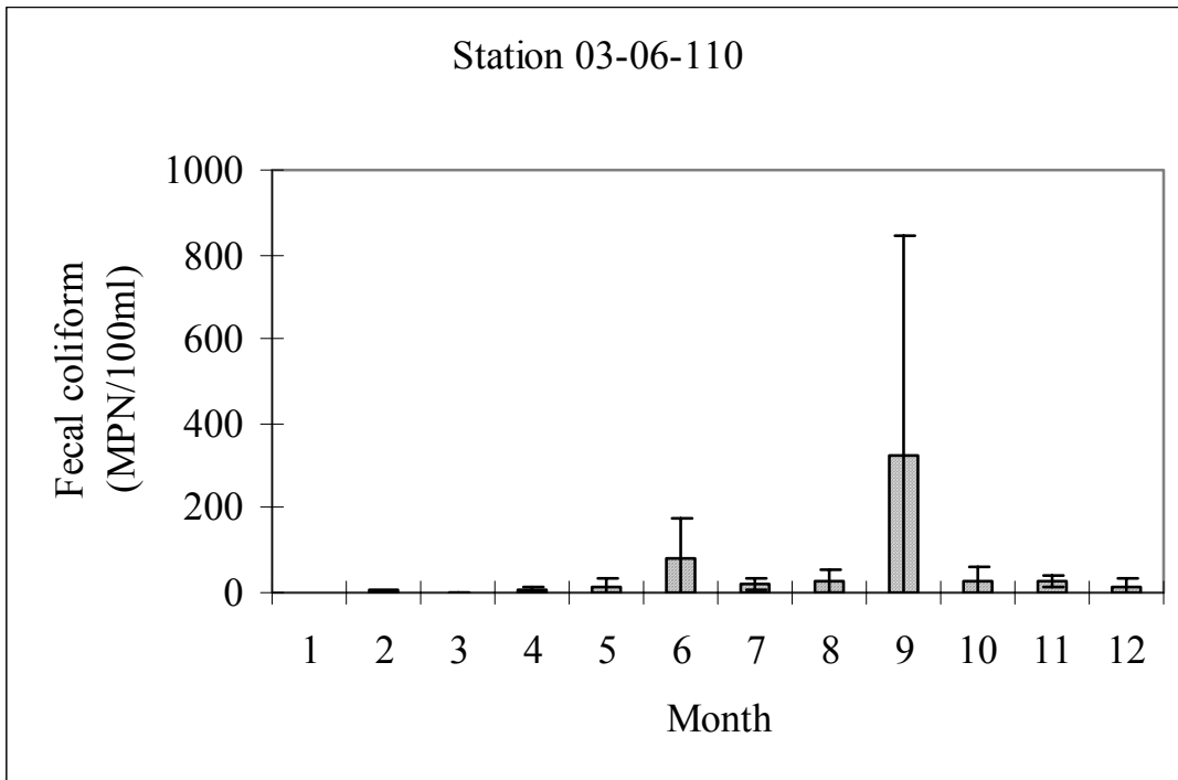
Figure E-1: Seasonality analysis of fecal coliform at South River Station 03-06-110
