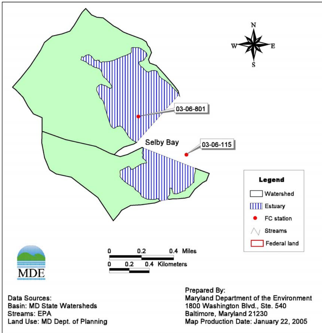
Figure 2.2.11: Shellfish Monitoring Stations in Selby Bay
