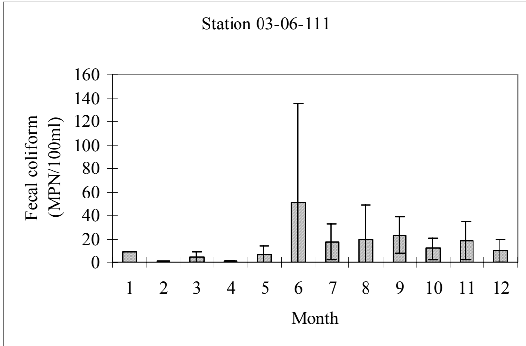
Figure E-6: Seasonality analysis of fecal coliform at South River Station 03-06-111
