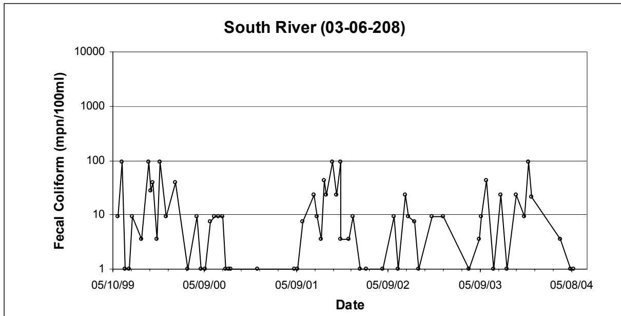
Figure 2.2.6: Observed Fecal Coliform Concentrations at Station 03-06-208
