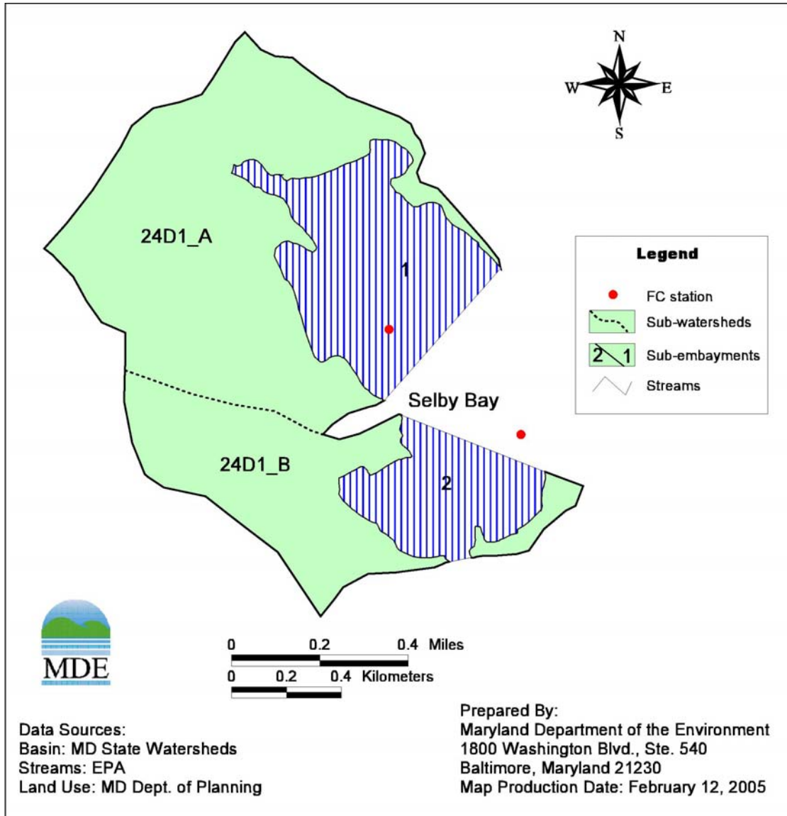
Figure B-2: Delineation for Selby Bay Basin
