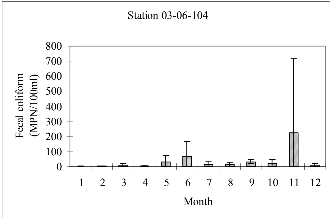
Figure E-7: Seasonality analysis of fecal coliform at Duvall Creek Station 03-06-104
