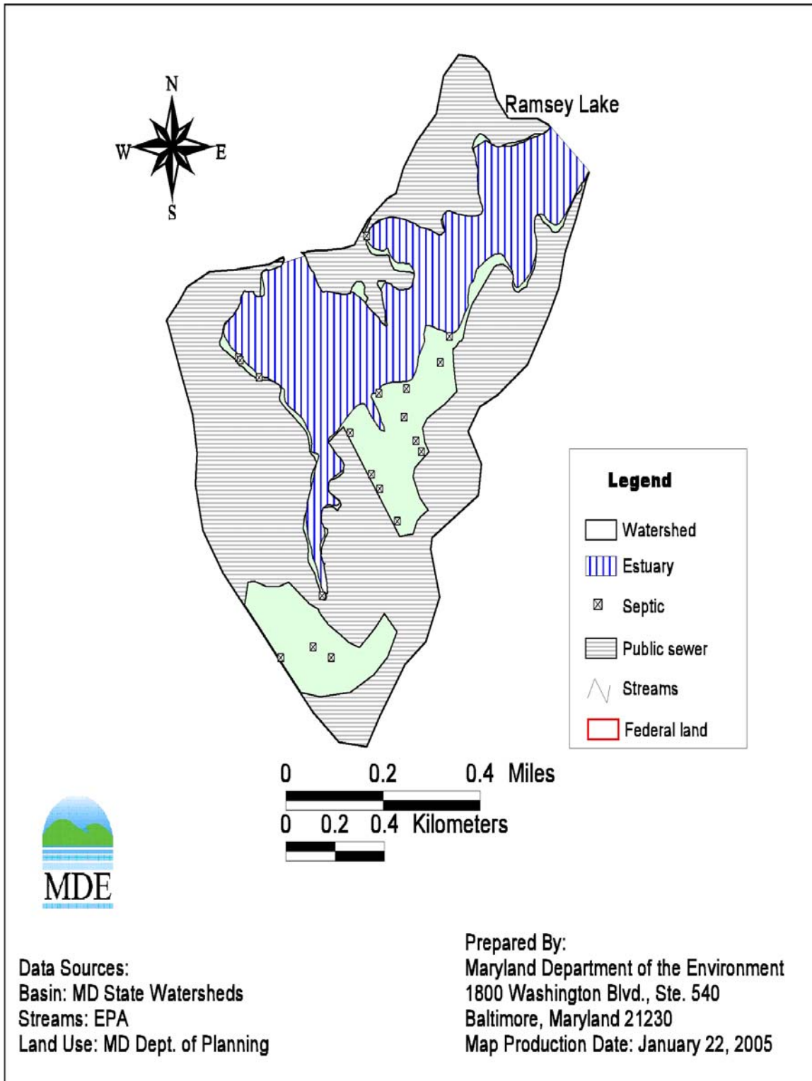
Figure D-4: Distribution of Septic Systems in the Ramsey Lake Watershed
