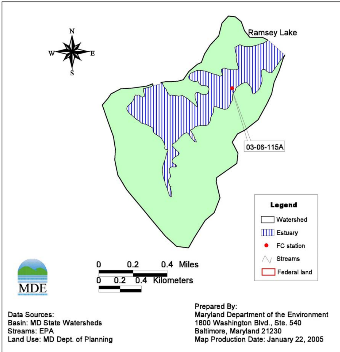
Figure 2.2.14: Shellfish Monitoring Stations in Ramsey Lake
