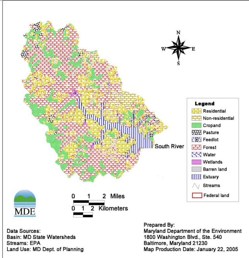
Figure 2.1.2: Land Use in the South River Basin
