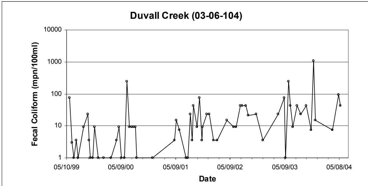
Figure 2.2.9: Observed Fecal Coliform Concentrations at Station 03-06-104
