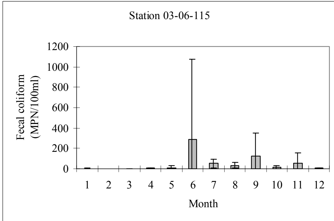
Figure E-10: Seasonality analysis of fecal coliform at Selby Bay Station 03-06-115
