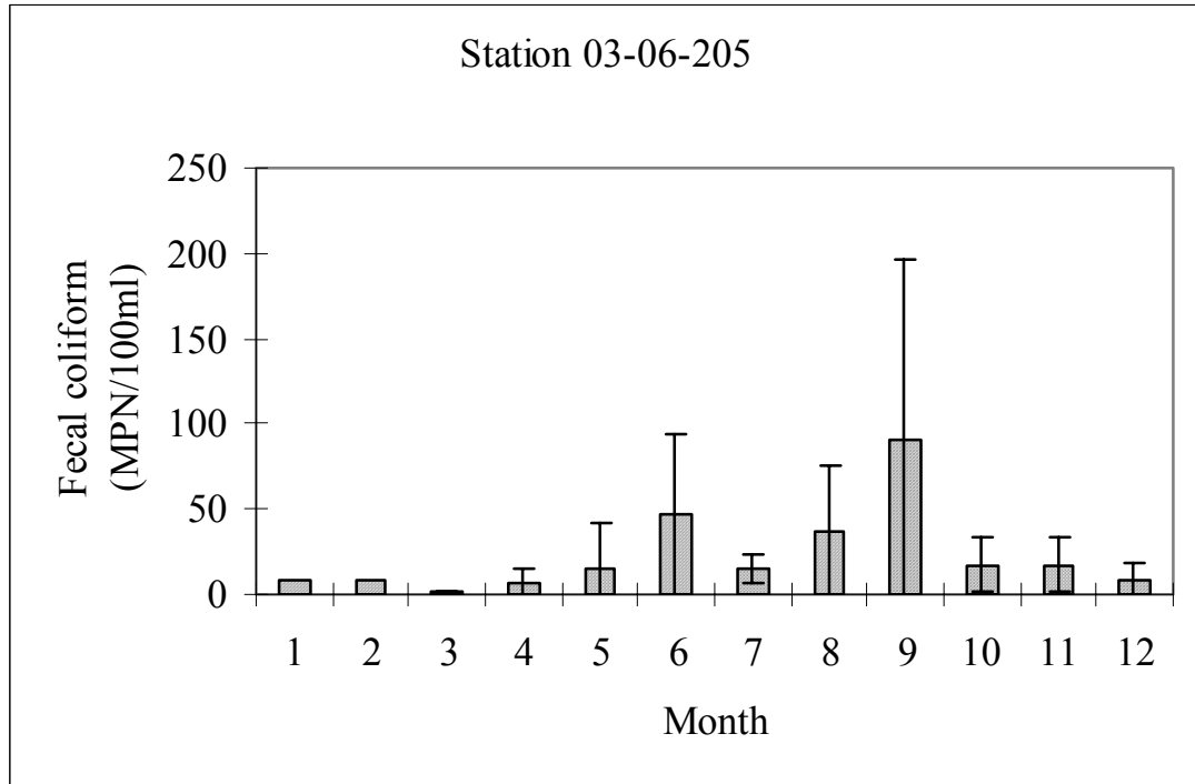
Figure E-4: Seasonality analysis of fecal coliform at South River Station 03-06-205
