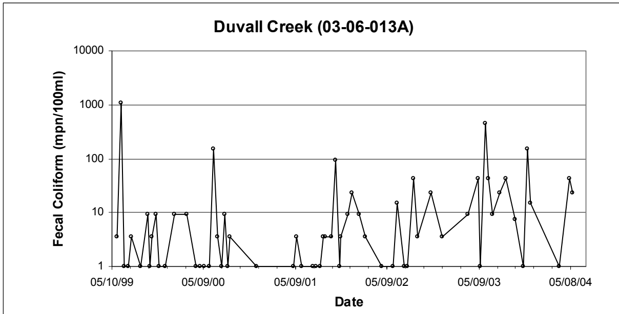
Figure 2.2.10: Observed Fecal Coliform Concentrations at Station 03-06-013A
