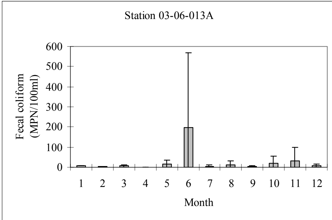
Figure E-8: Seasonality analysis of fecal coliform at Duvall Creek Station 03-06-013A
