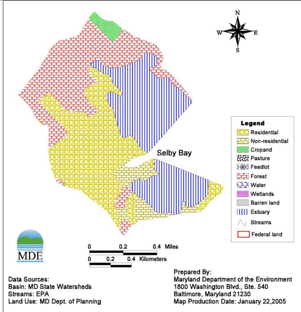
Figure 2.1.4: Land Use in the Selby Bay Watershed
