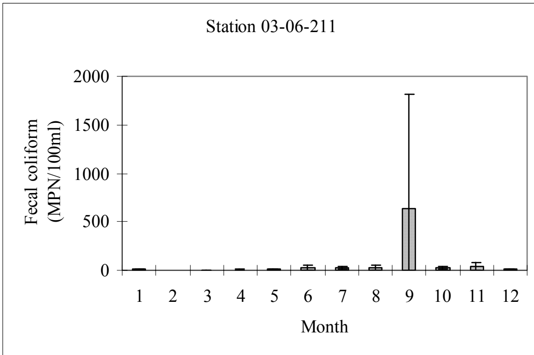
Figure E-2: Seasonality analysis of fecal coliform at South River Station 03-06-211
