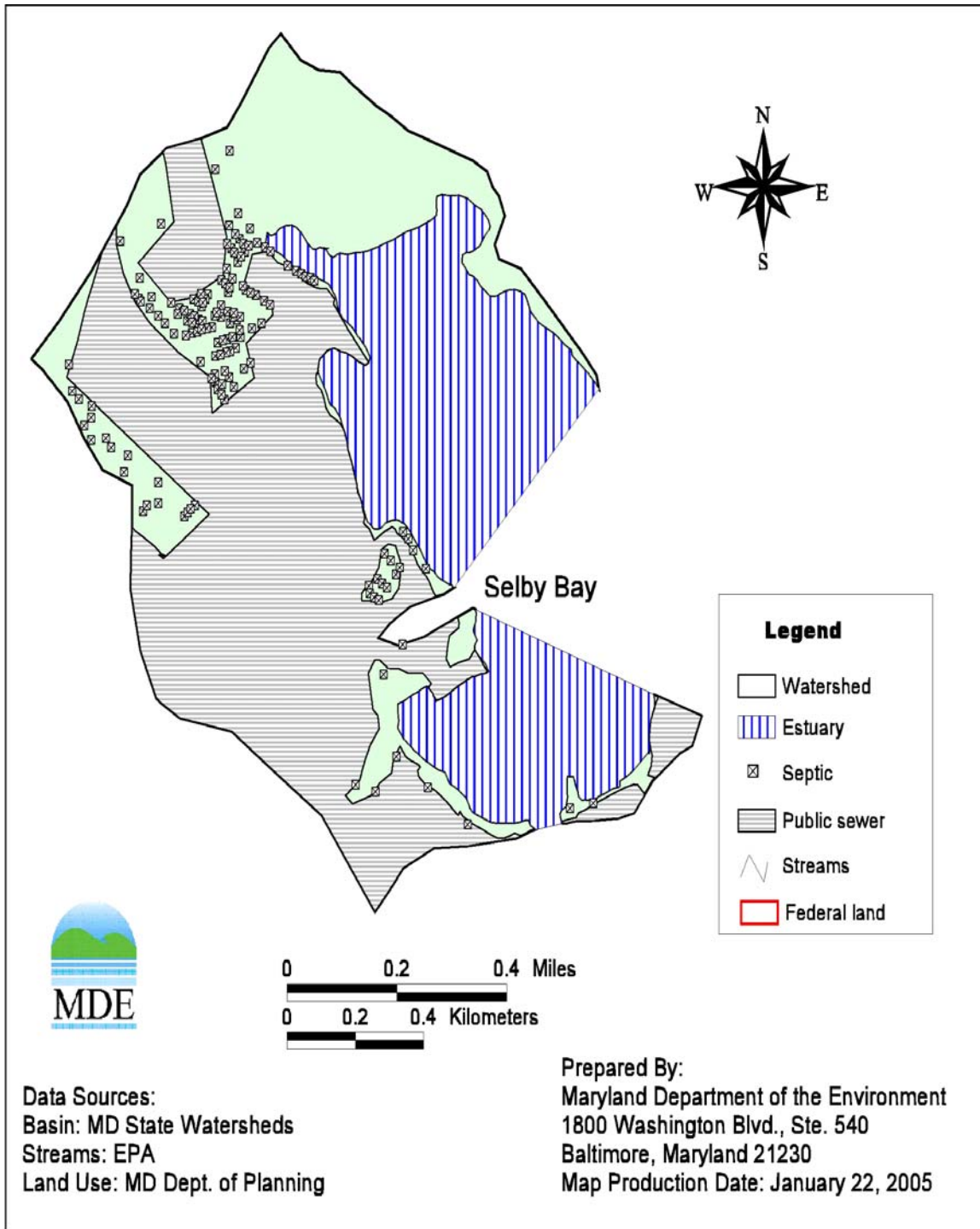
Figure D-3: Distribution of Septic Systems in the Selby Bay Watershed
