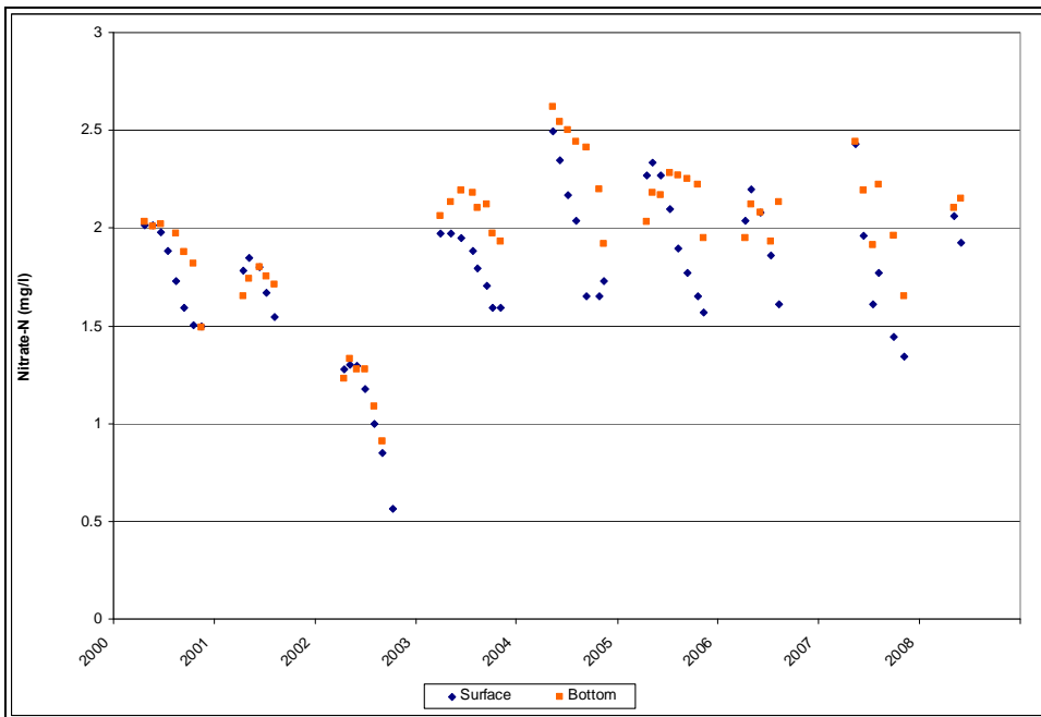
Figure B-22: Liberty Reservoir BCDPW Station NPA0059 Average Nitrate (2000-2008)
