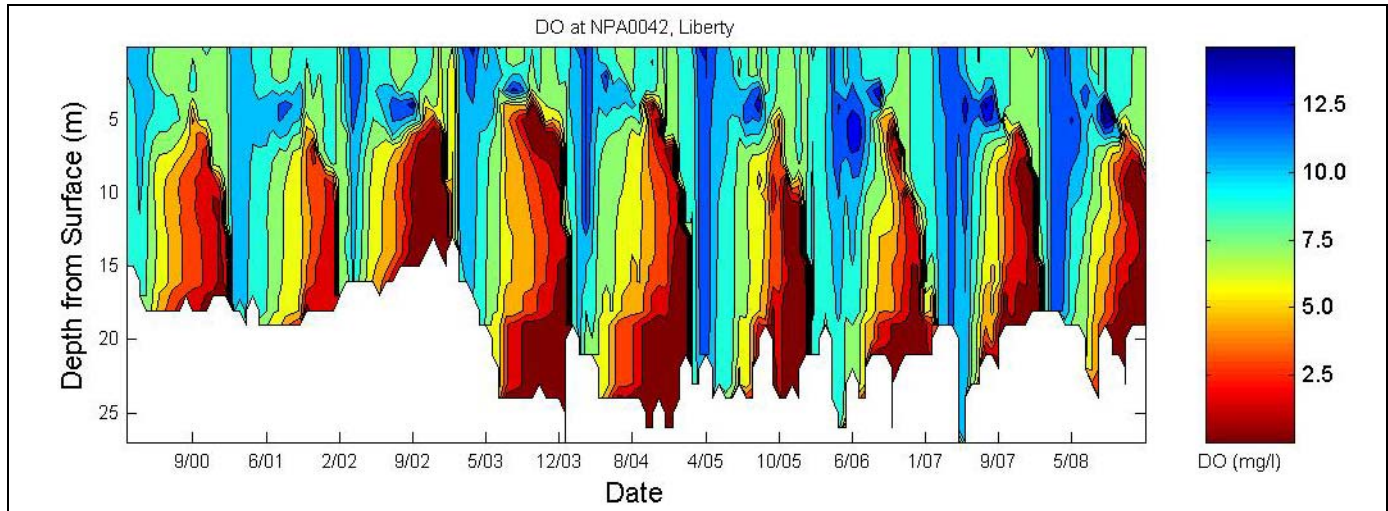
Figure B-5: Liberty Reservoir BCDPW Station NPA0042 DO Contours (2000-2008)
