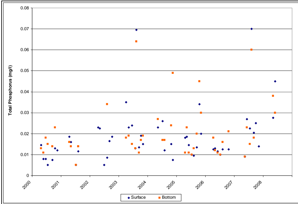
Figure B-15: Liberty Reservoir BCDPW Station NPA0067 Average Total Phosphorus (2000-2008)
