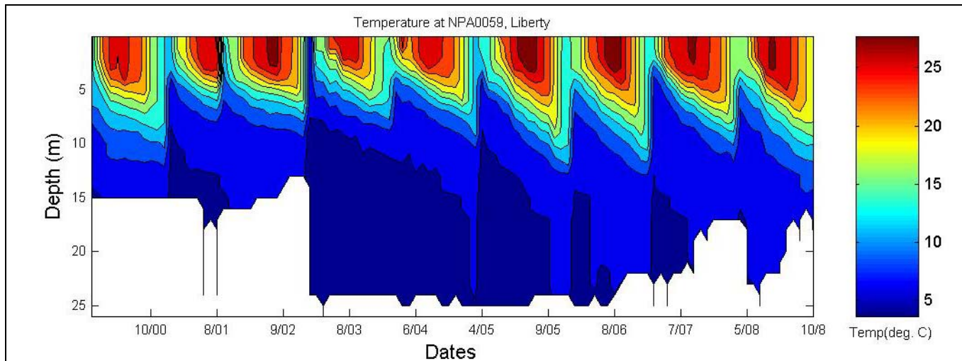
Figure B-2: Liberty Reservoir BCDPW Station NPA0059 Isothermal Contours (2000–2008)
