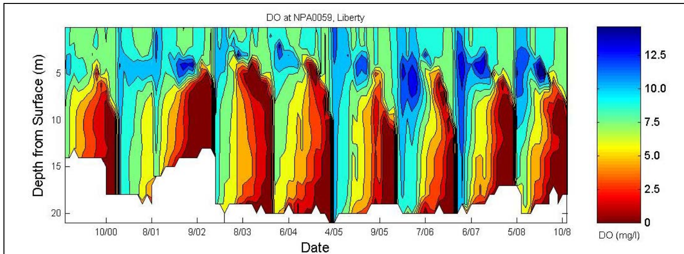
Figure B-6: Liberty Reservoir BCDPW Station NPA0059 DO Contours (2000-2008)
