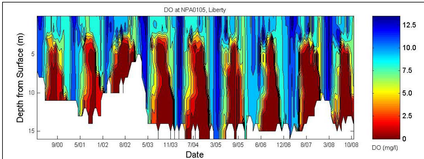
Figure B-8: Liberty Reservoir BCDPW Station NPA0105 DO Contours (2000-2008)
