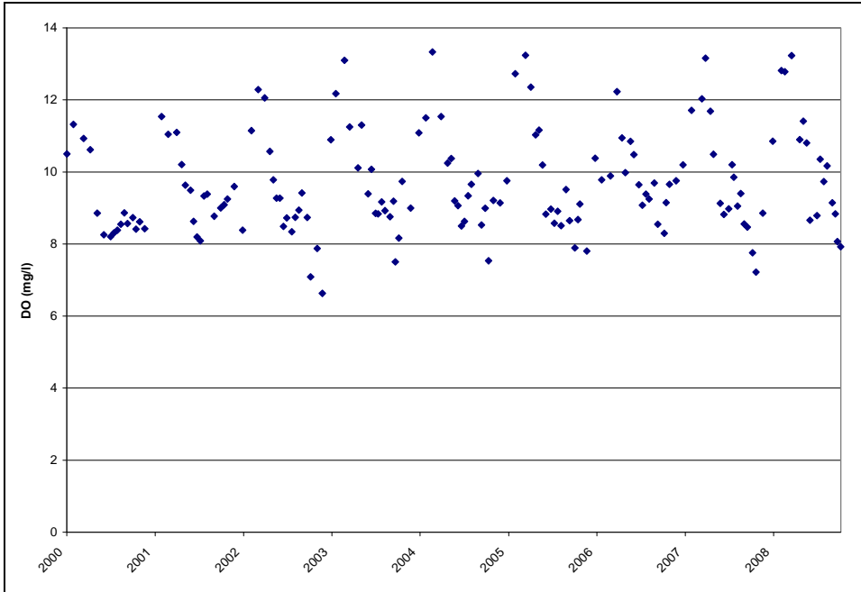
Figure B-9: Liberty Reservoir BCDPW Station NPA0042 Average Surface Dissolved Oxygen (2000-2008)
