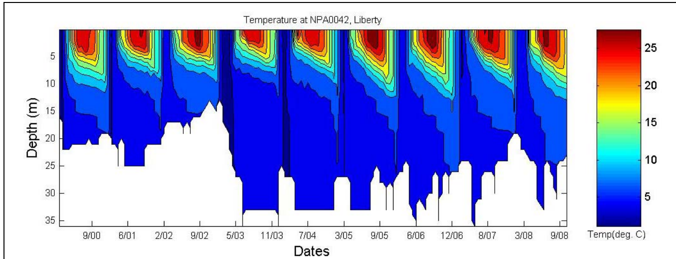
Figure B-1: Liberty Reservoir BCDPW Station NPA0042 Isothermal Contours (2000–2008)
