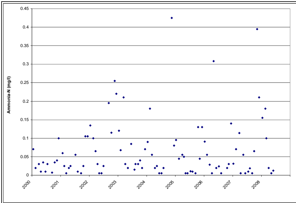
Figure B-20: Liberty Reservoir BCDPW Station NPA0105 Average Ammonia (2000-2008)
