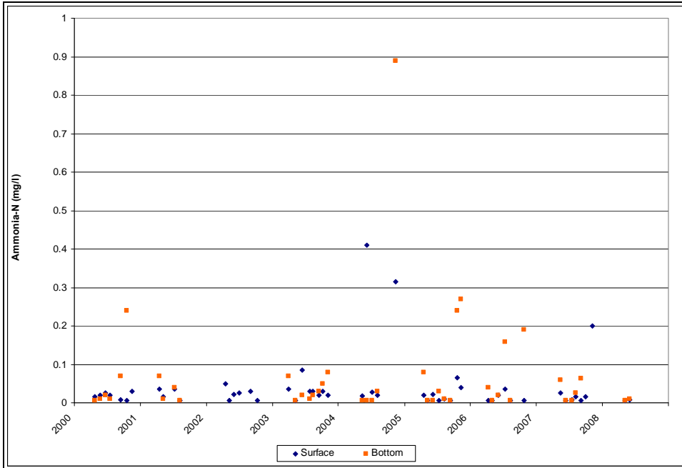
Figure B-19: Liberty Reservoir BCDPW Station NPA0067 Average Ammonia (2000-2008)
