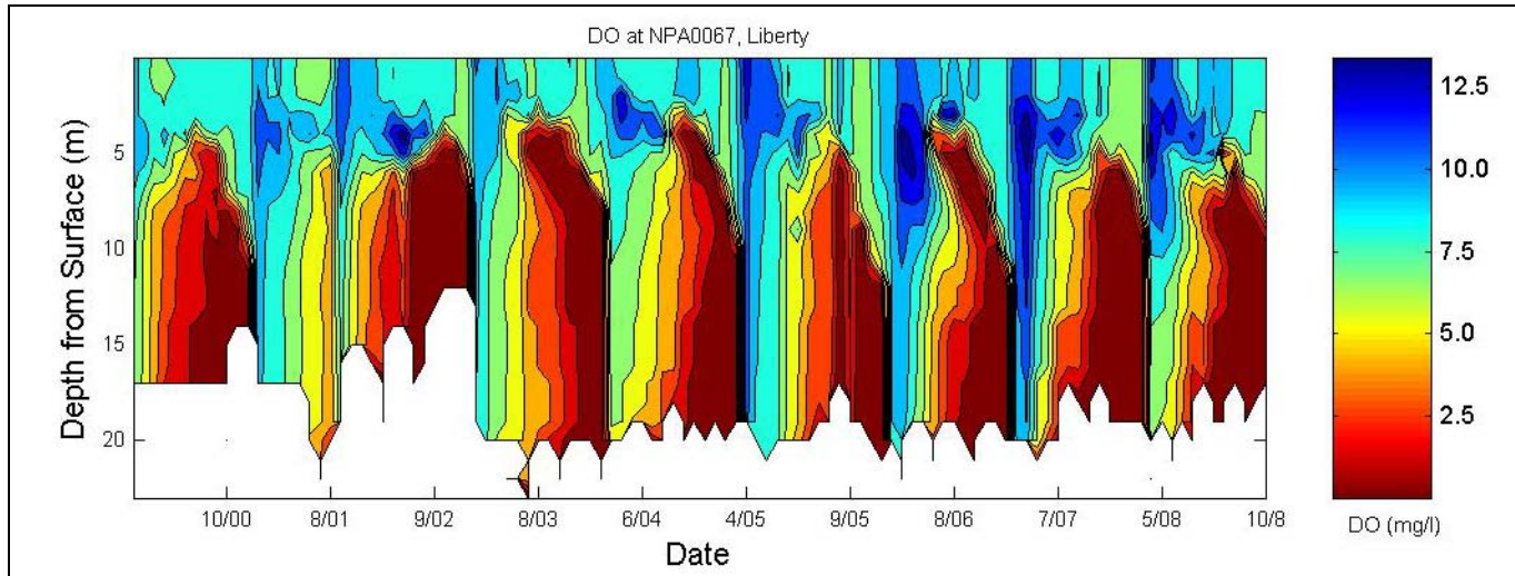
Figure B-7: Liberty Reservoir BCDPW Station NPA0067 DO Contours (2000-2008)
