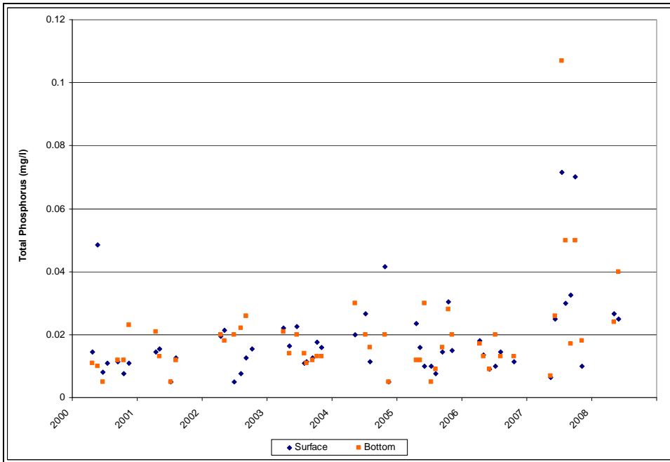
Figure B-14: Liberty Reservoir BCDPW Station NPA0059 Average Total Phosphorus (2000-2008)
