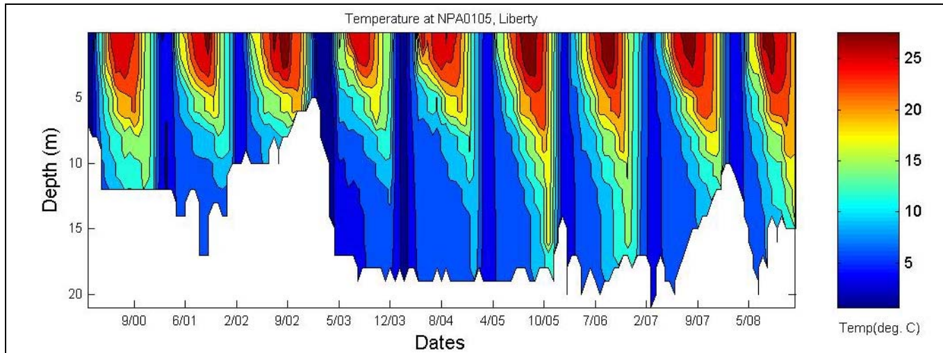
Figure B-4: Liberty Reservoir BCDPW Station NPA0105 Isothermal Contours (2000-2008)
