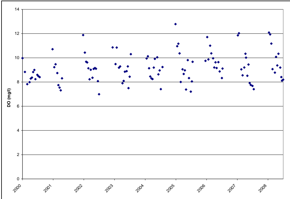
Figure B-11: Liberty Reservoir BCDPW Station NPA0067 Average Surface Dissolved Oxygen (2000-2008)
