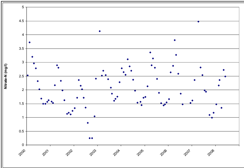
Figure B-24: Liberty Reservoir BCDPW Station NPA0105 Average Nitrate (2000-2008)
