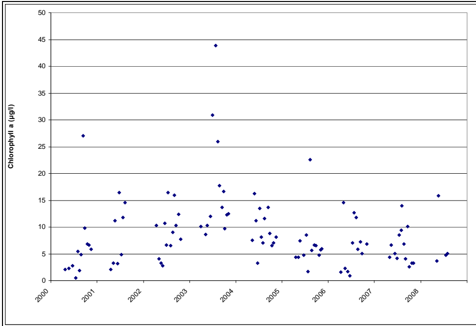
Figure B-27: Liberty Reservoir BCDPW Station NPA0067 Maximum Surface Chlorophyll a- (2000-2008)
