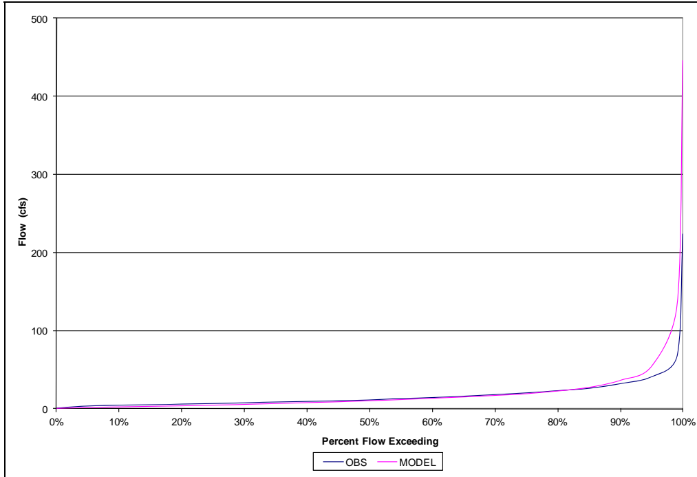
Figure A-7: Cumulative Distribution of Observed and Simulated Flows, Beaver Run
