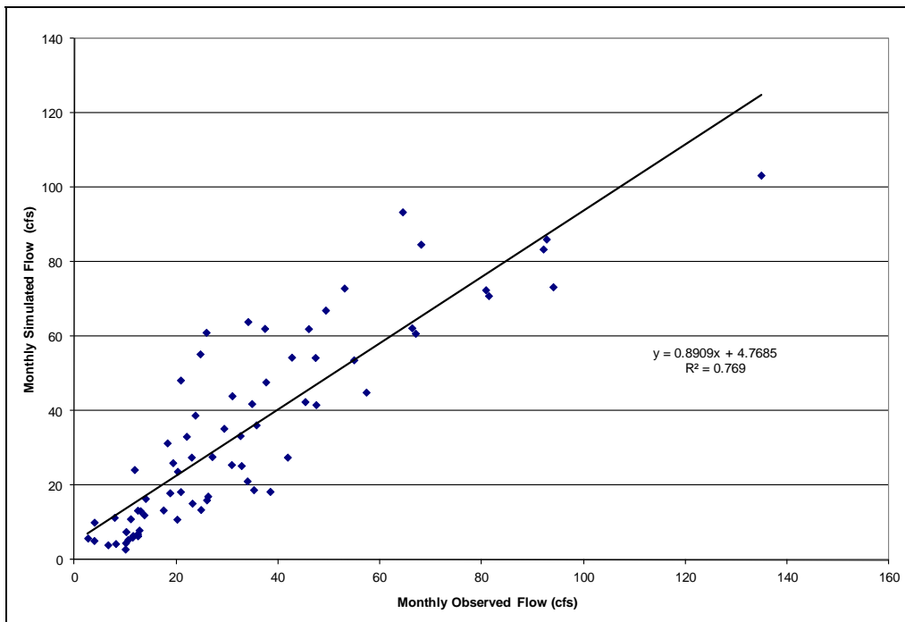
Figure A-12: Observed vs. Simulated Monthly Flows, Morgan Run
