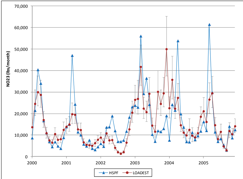
Figure A-57: Time Series of LOADEST and HSPF Monthly Nitrate Loads, Morgan Run
