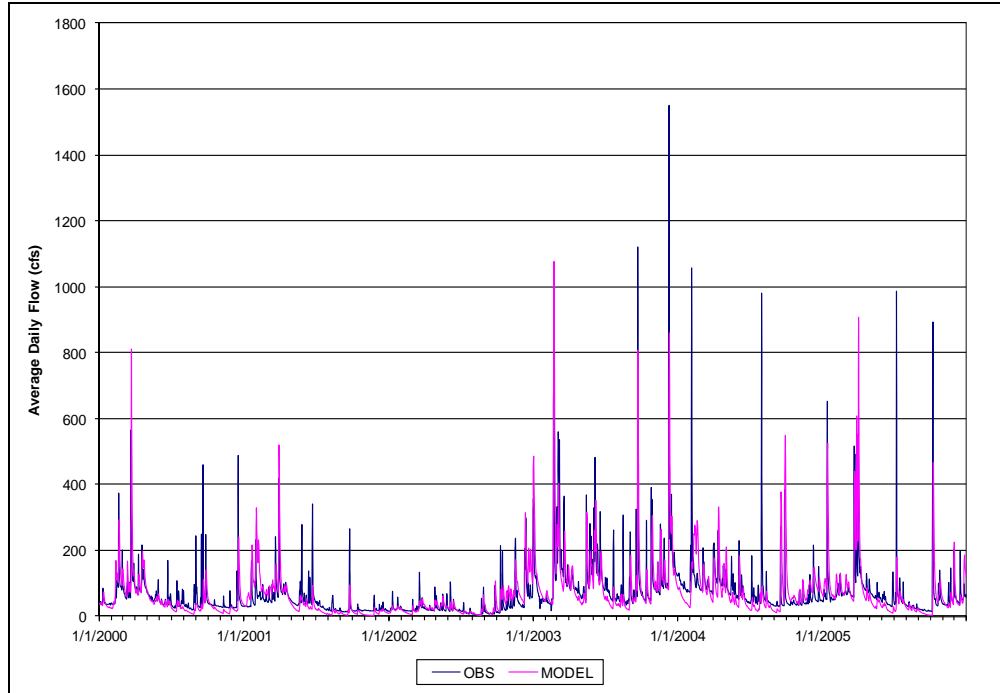
Figure A-1: Daily Observed and Simulated Flows, North Branch Patapsco River
