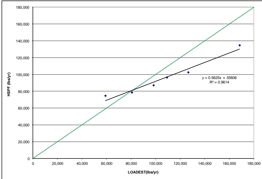
Figure A-53: Scatter Plot, ESTIMATOR and HSPF Annual Nitrate Loads, Beaver Run
