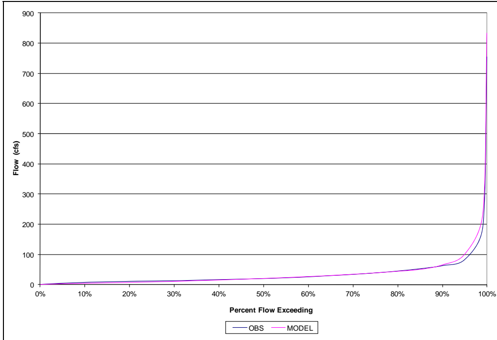
Figure A-11: Cumulative Distribution of Observed and Simulated Flows, Morgan Run
