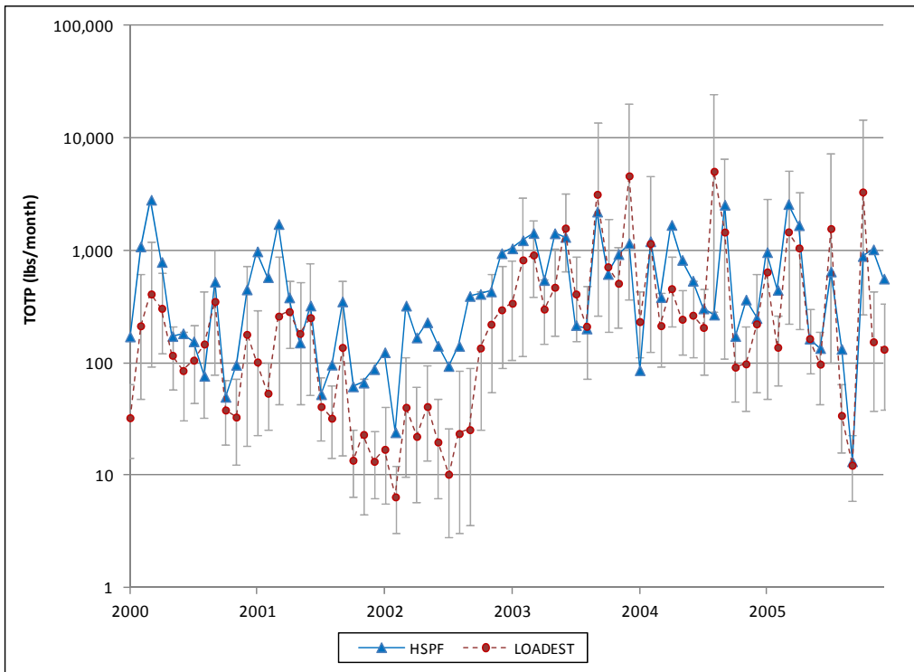
Figure A-32: Time Series of LOADEST and HSPF Monthly Total Phosphorus Loads, Beaver Run
