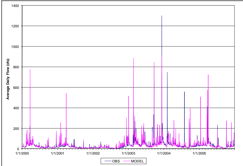
Figure A-9: Daily Observed and Simulated Flows, Morgan Run
