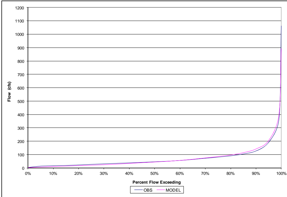
Figure A-3: Cumulative Distribution of Observed and Simulated Flows, North Branch Patapsco River
