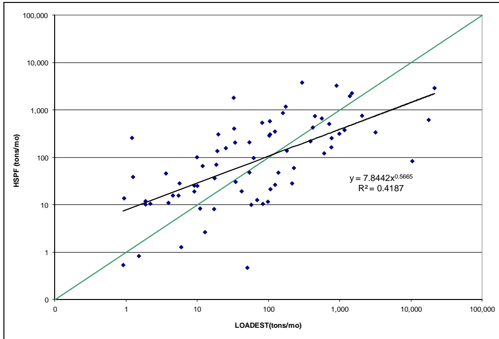
Figure A-24: Scatter Plot, ESTIMATOR and HSPF Monthly Sediment Loads, Morgan Run
