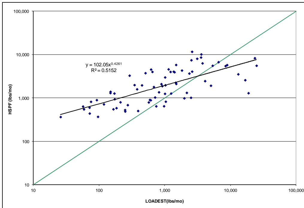
Figure A-34: Scatter Plot, ESTIMATOR and HSPF Monthly Total Phosphorus Loads, North Branch Patapsco River
