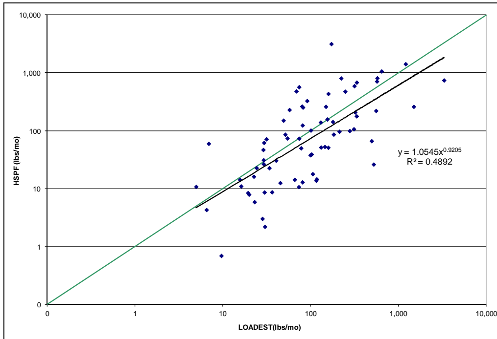
Figure A-48: Scatter Plot, ESTIMATOR and HSPF Monthly Ammonia Loads, Morgan Run
