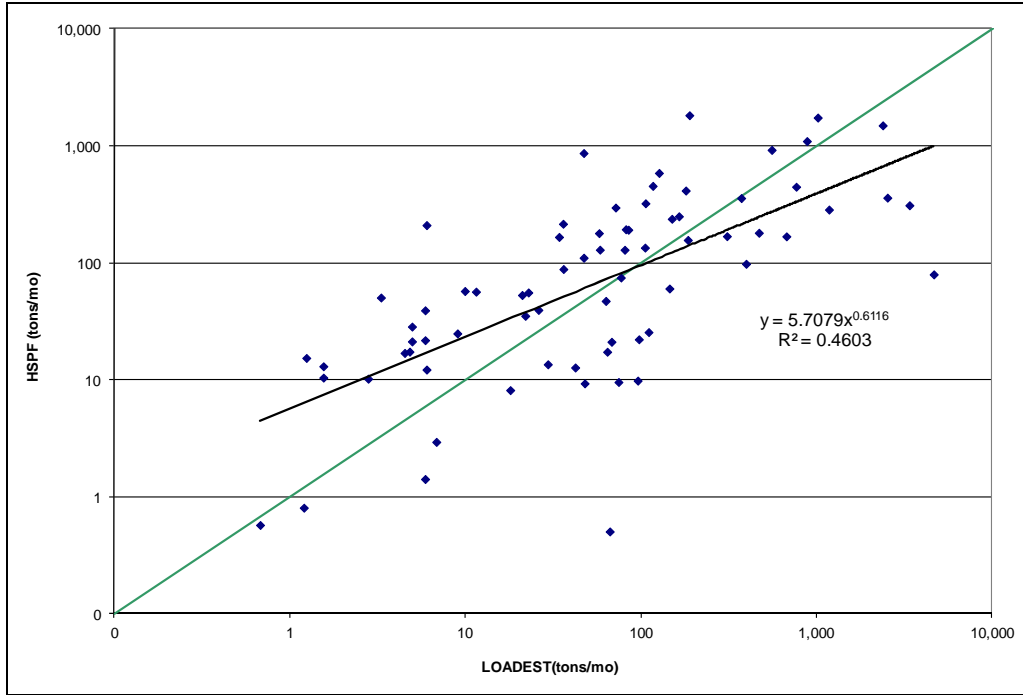
Figure A-23: Scatter Plot, ESTIMATOR and HSPF Monthly Sediment Loads, Beaver Run
