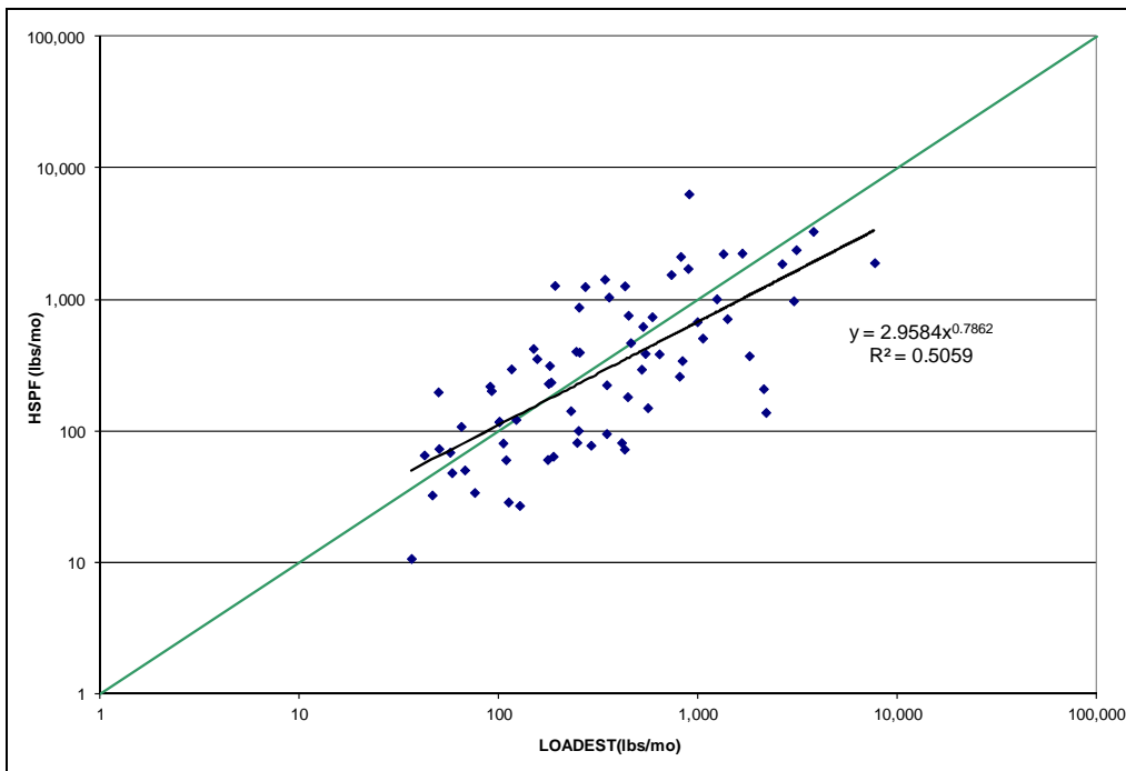
Figure A-46: Scatter Plot, ESTIMATOR and HSPF Monthly Ammonia Loads, North Branch Patapsco River
