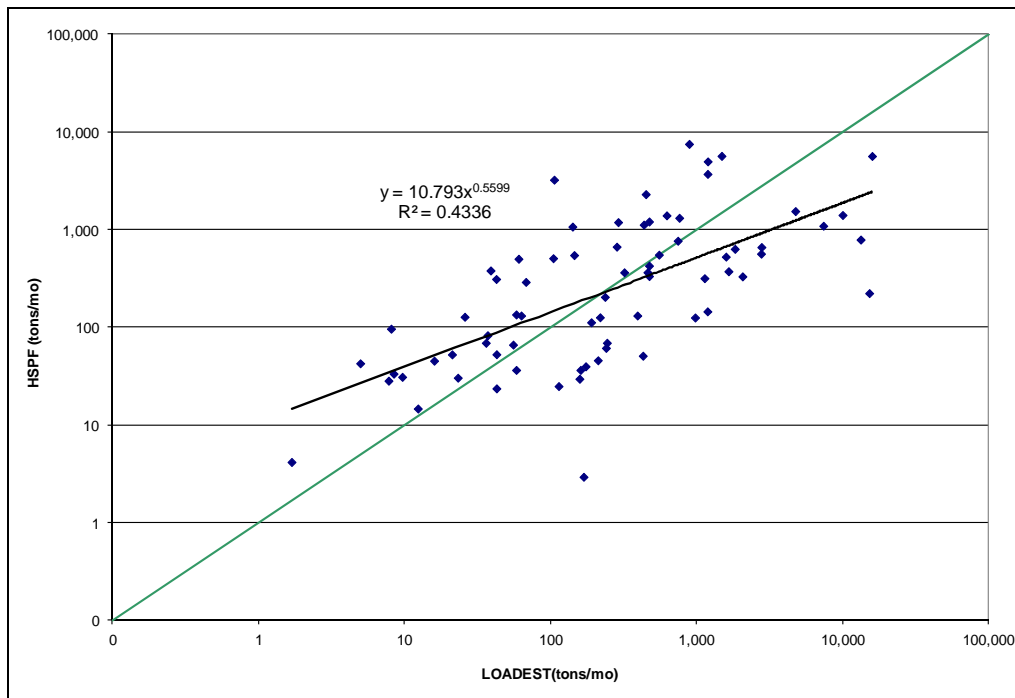
Figure A-22: Scatter Plot, ESTIMATOR and HSPF Monthly Sediment Loads, North Branch Patapsco River
