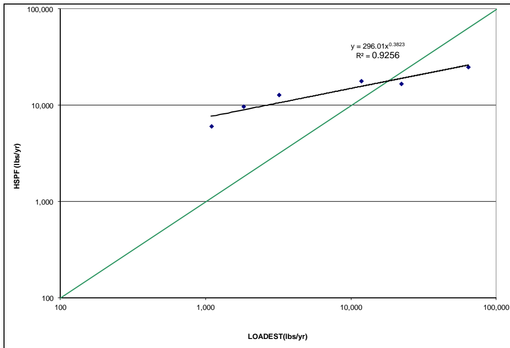
Figure A-30: Scatter Plot, ESTIMATOR and HSPF Annual Total Phosphorus Loads, Morgan Run
