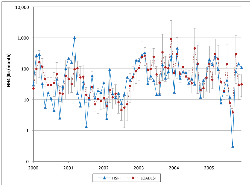
Figure A-44: Time Series of LOADEST and HSPF Monthly Ammonia Loads, Beaver Run
