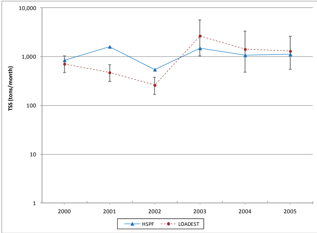
Figure A-39: Time Series of LOADEST and HSPF Annual Ammonia Loads, Morgan Run
