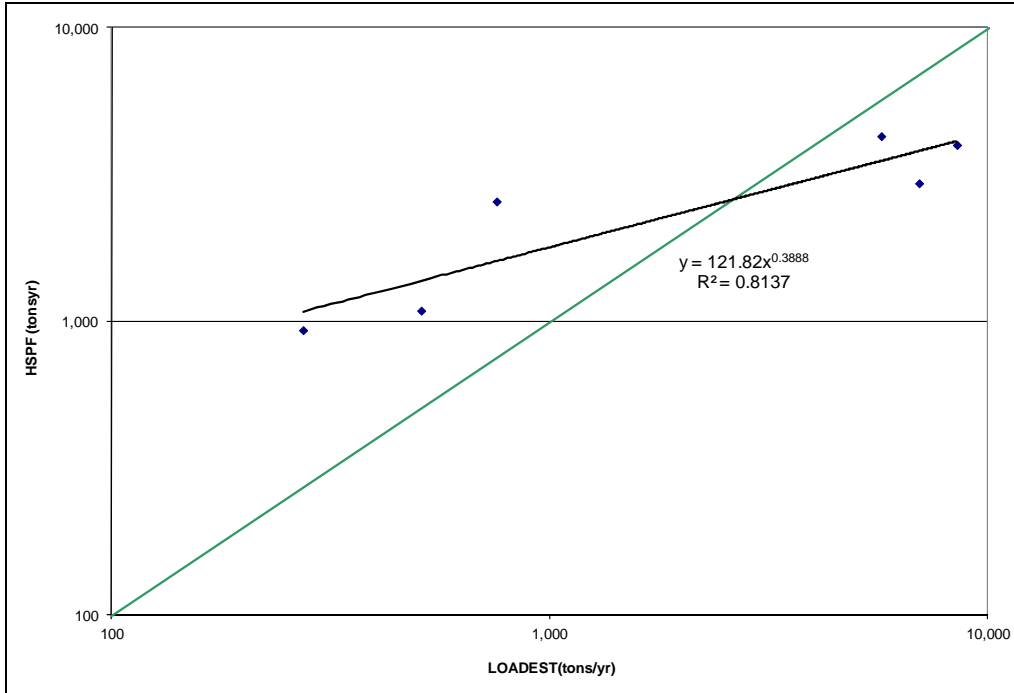
Figure A-17: Scatter Plot, ESTIMATOR and HSPF Annual Sediment Loads, Beaver Run
