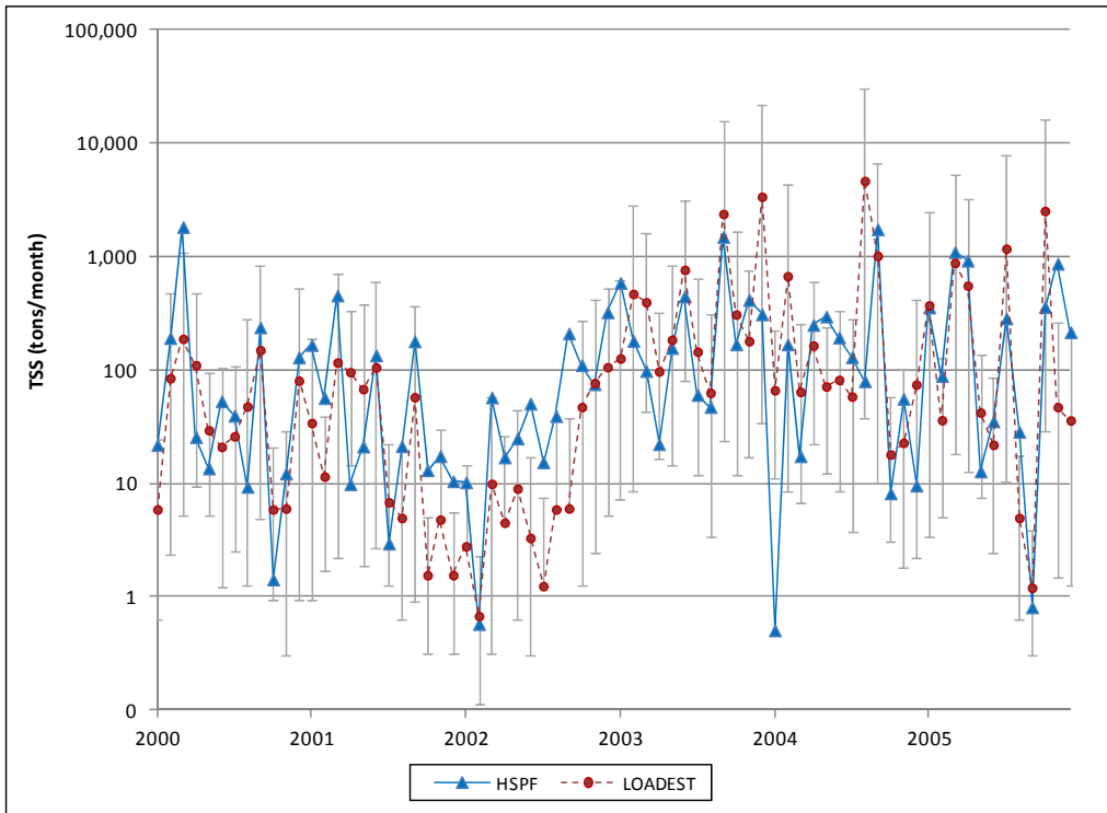
Figure A-20: Time Series of LOADEST and HSPF Monthly Sediment Loads, Beaver Run
