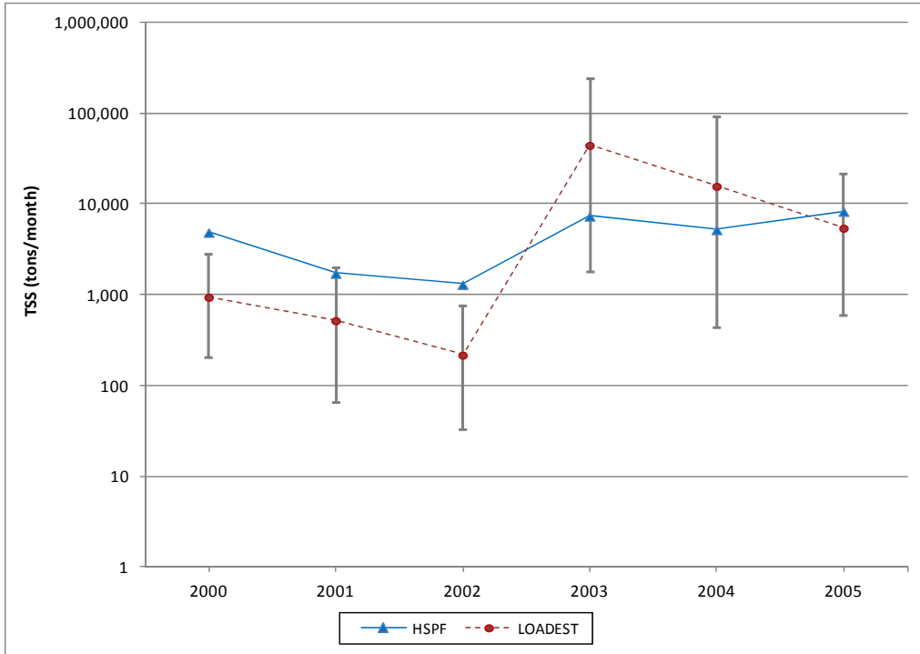
Figure A-15: Time Series of LOADEST and HSPF Annual Sediment Loads, Morgan Run
