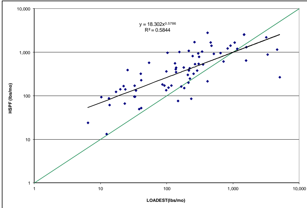
Figure A-35: Scatter Plot, ESTIMATOR and HSPF Monthly Total Phosphorus Loads, Beaver Run
