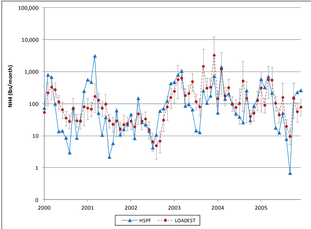
Figure A-45: Time Series of LOADEST and HSPF Monthly Ammonia Loads, Morgan Run
