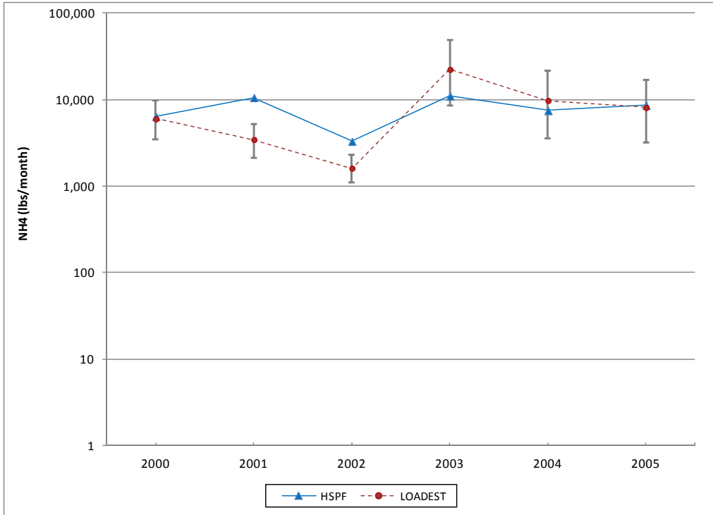
Figure A-37: Time Series of LOADEST and HSPF Annual Ammonia Loads, North Branch Patapsco River
