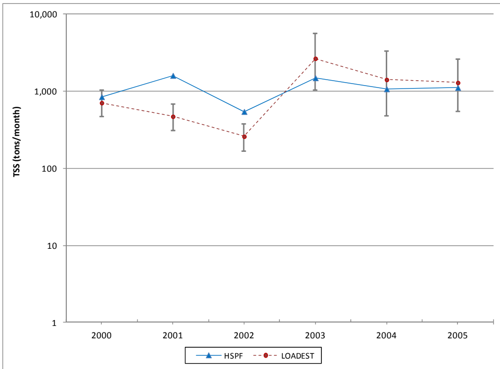
Figure A-38: Time Series of LOADEST and HSPF Annual Ammonia Loads, Beaver Run
