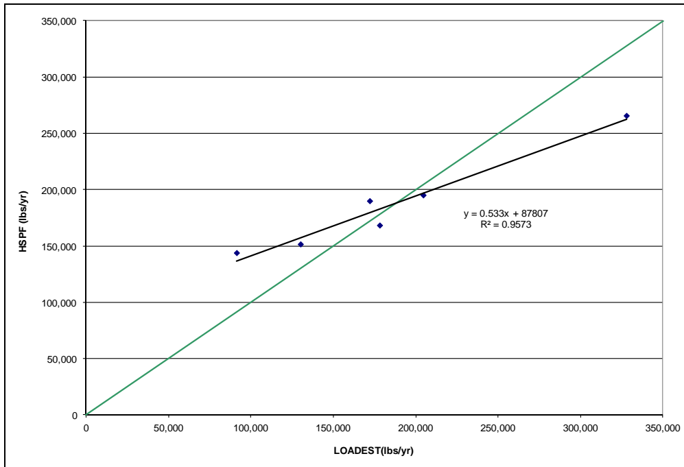
Figure A-54: Scatter Plot, ESTIMATOR and HSPF Annual Nitrate Loads, Morgan Run
