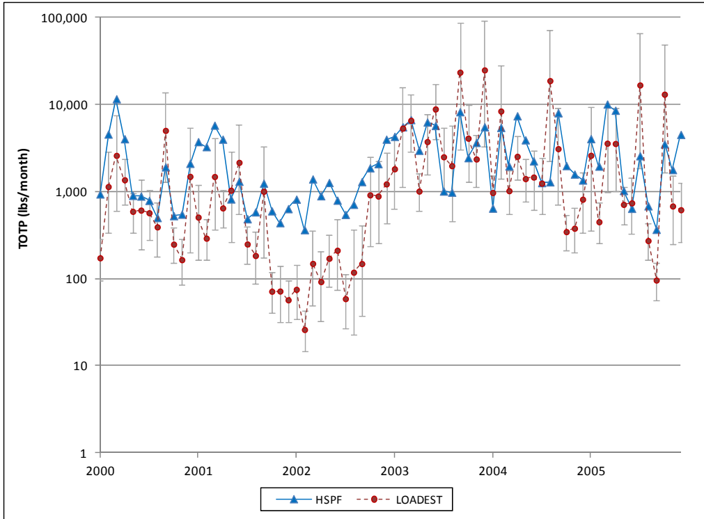
Figure A-31: Time Series of LOADEST and HSPF Monthly Total Phosphorus Loads, North Branch Patapsco River
