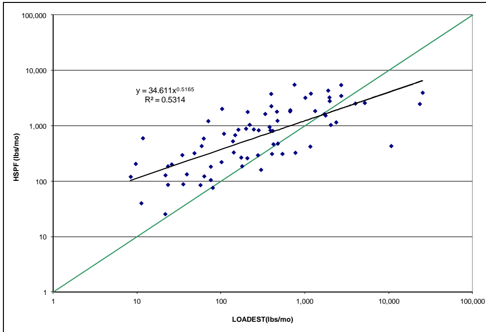
Figure A-36: Scatter Plot, ESTIMATOR and HSPF Monthly Total Phosphorus Loads, Morgan Run
