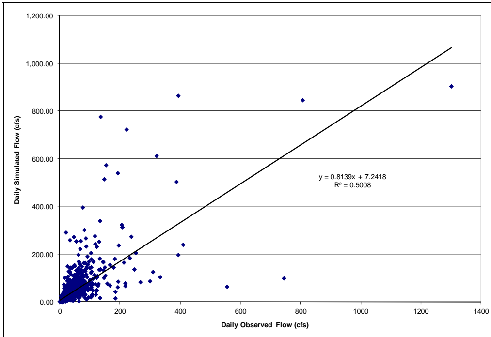
Figure A-10: Observed vs. Simulated Daily Flows, Morgan Run
