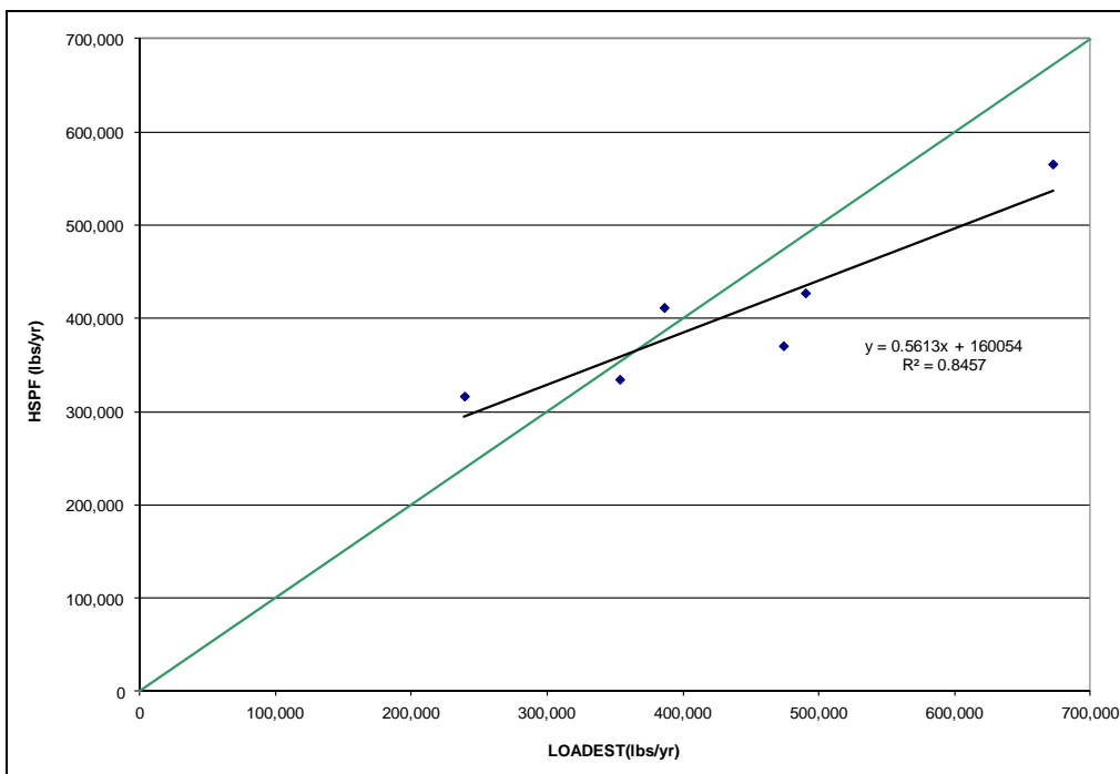
Figure A-52: Scatter Plot, ESTIMATOR and HSPF Annual Nitrate Loads, North Branch Patapsco River
