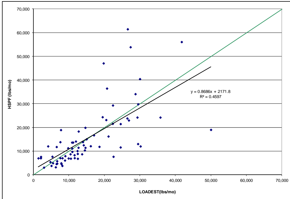
Figure A-60: Scatter Plot, ESTIMATOR and HSPF Monthly Nitrate Loads, Morgan Run
