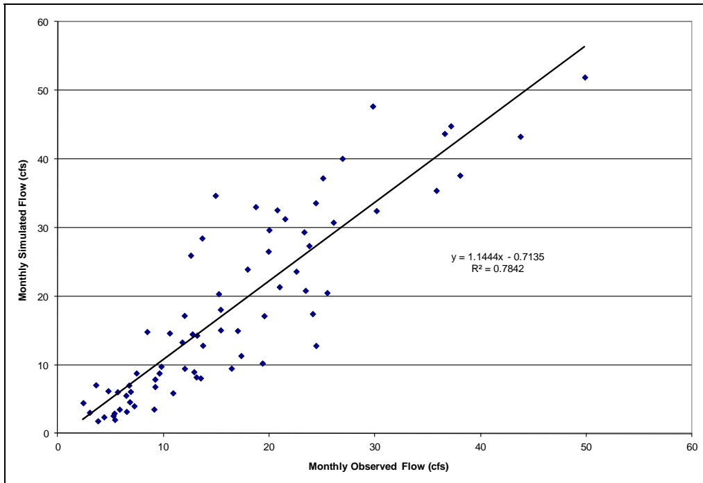
Figure A-8: Observed vs. Simulated Monthly Flows, Beaver Run
