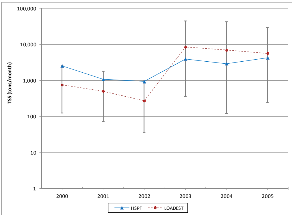
Figure A-14: Time Series of LOADEST and HSPF Annual Sediment Loads, Beaver Run
