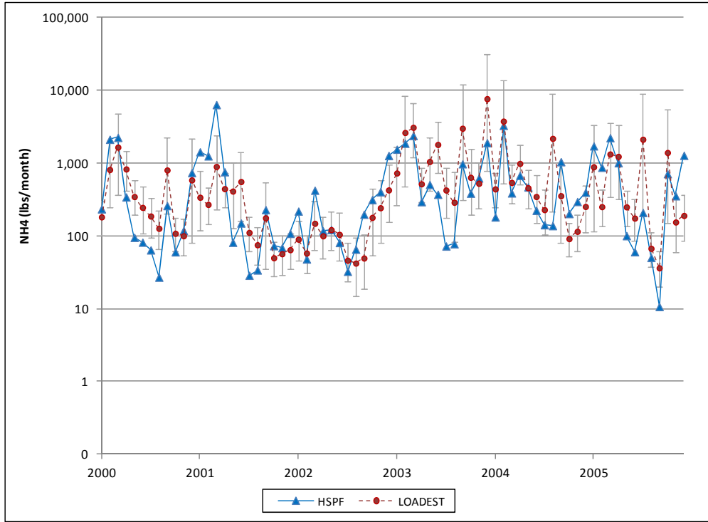
Figure A-43: Time Series of LOADEST and HSPF Monthly Ammonia Loads, North Branch Patapsco River
