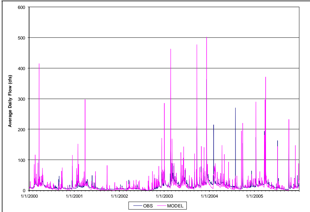
Figure A-5: Daily Observed and Simulated Flows, Beaver Run
