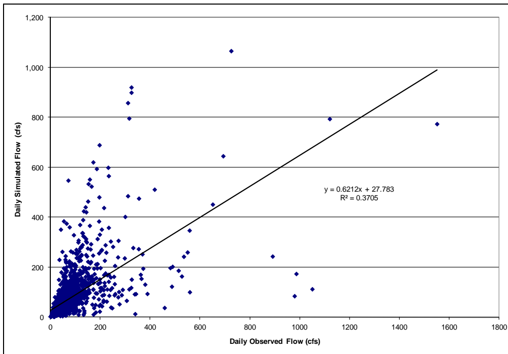
Figure A-2: Observed vs. Simulated Daily Flows, North Branch Patapsco River
