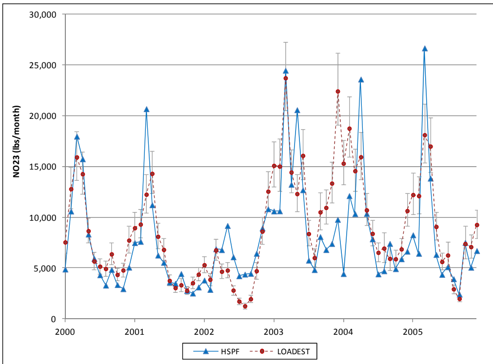
Figure A-56: Time Series of LOADEST and HSPF Monthly Nitrate Loads, Beaver Run
