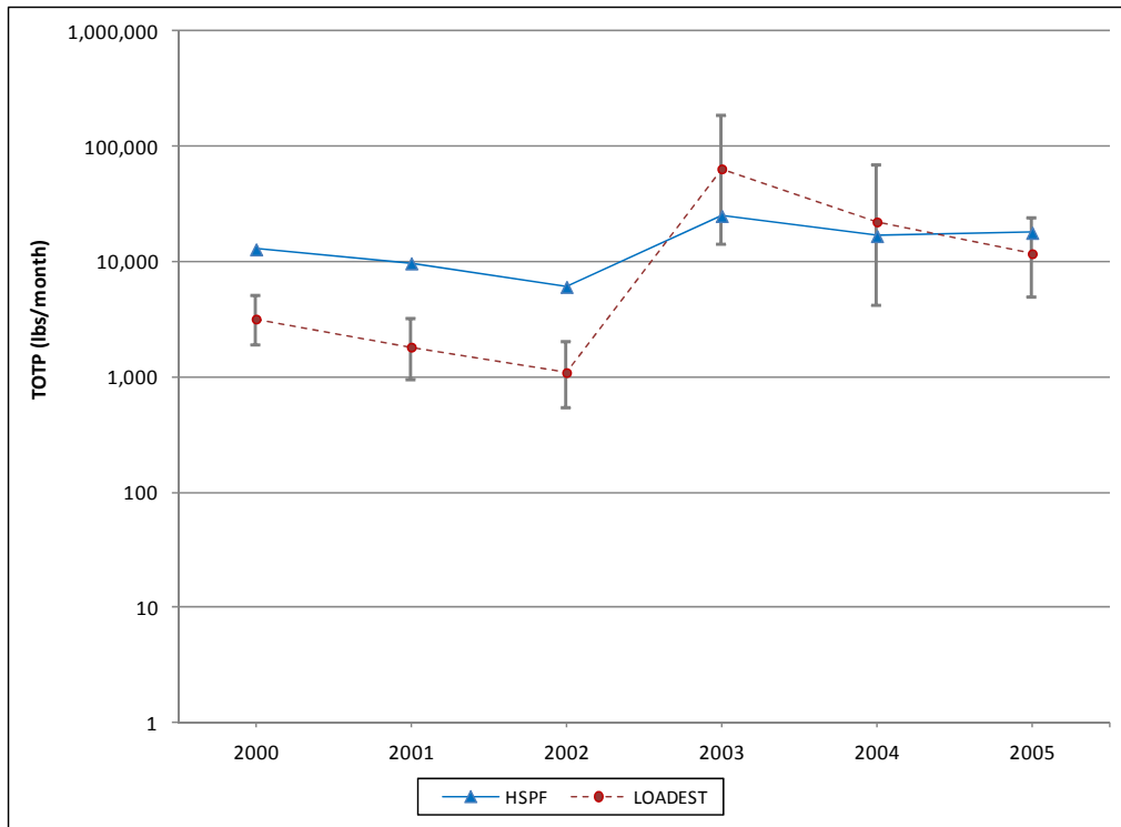
Figure A-27: Time Series of LOADEST and HSPF Annual Total Phosphorus Loads, Morgan Run
