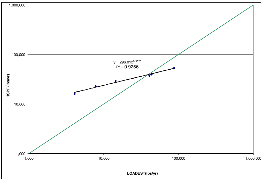
Figure A-28: Scatter Plot, ESTIMATOR and HSPF Annual Total Phosphorus Loads, North Branch Patapsco River
