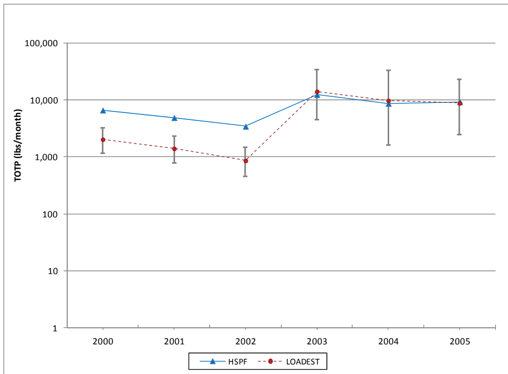
Figure A-26: Time Series of LOADEST and HSPF Annual Total Phosphorus Loads, Beaver Run
