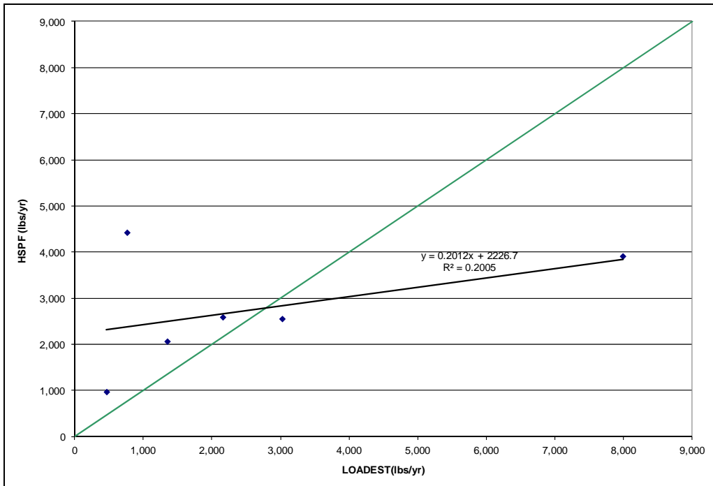
Figure A-42: Scatter Plot, ESTIMATOR and HSPF Annual Ammonia Loads, Morgan Run
