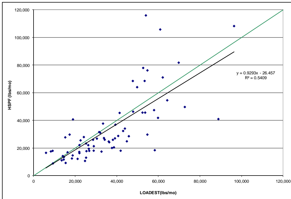
Figure A-58: Scatter Plot, ESTIMATOR and HSPF Monthly Nitrate Loads, North Branch Patapsco River
