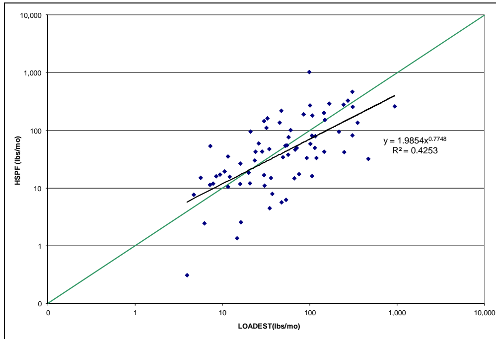
Figure A-47: Scatter Plot, ESTIMATOR and HSPF Monthly Ammonia Loads, Beaver Run
