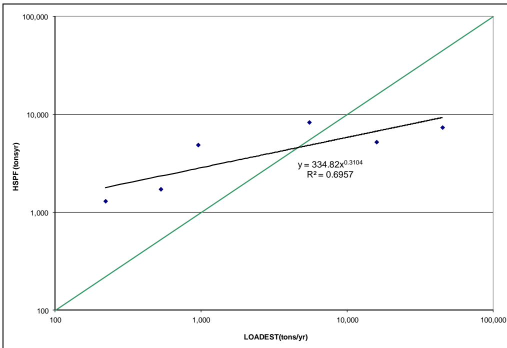
Figure A-18: Scatter Plot, ESTIMATOR and HSPF Annual Sediment Loads, Morgan Run
