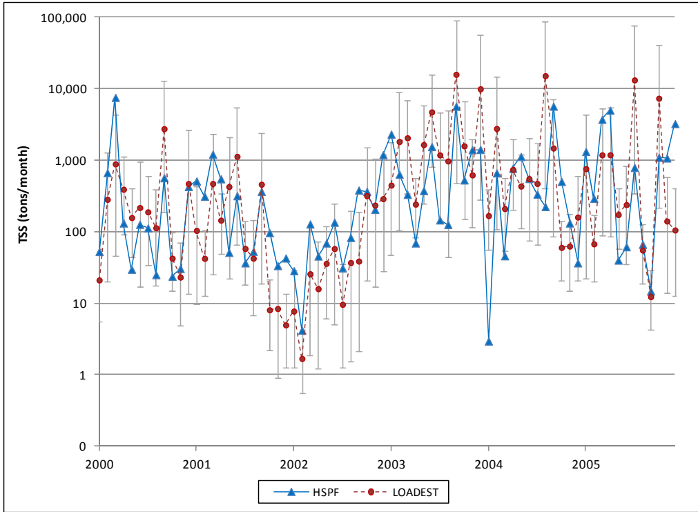
Figure A-19: Time Series of LOADEST and HSPF Monthly Sediment Loads, North Branch Patapsco River
