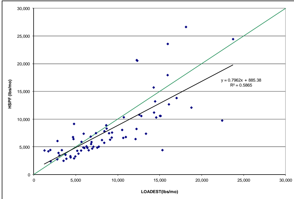
Figure A-59: Scatter Plot, ESTIMATOR and HSPF Monthly Nitrate Loads, Beaver Run
