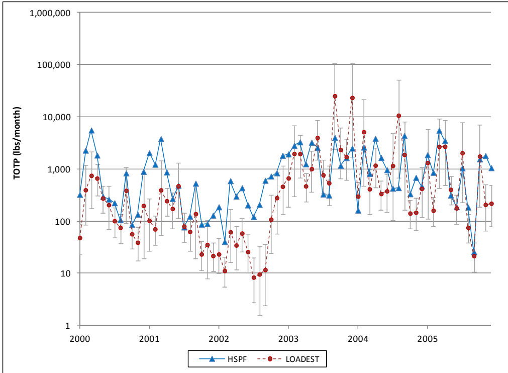
Figure A-33: Time Series of LOADEST and HSPF Monthly Total Phosphorus Loads, Morgan Run
