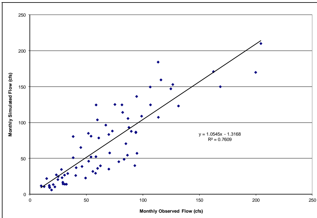
Figure A-4: Observed vs. Simulated Monthly Flows, North Branch Patapsco River
