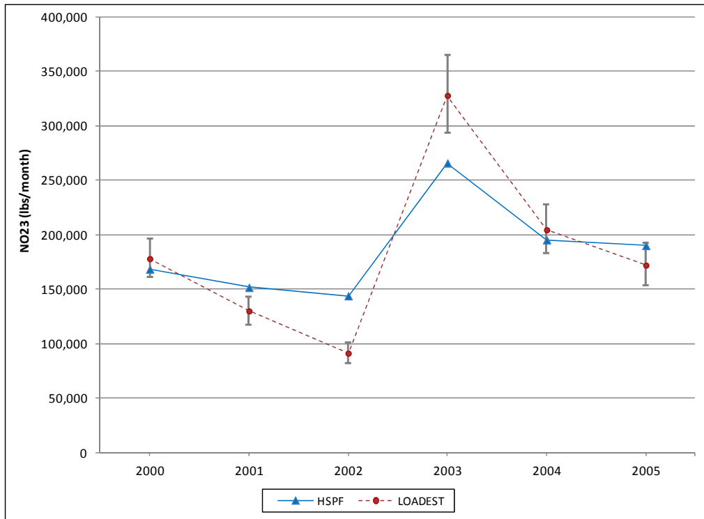
Figure A-51: Time Series of LOADEST and HSPF Annual Nitrate Loads, Morgan Run
