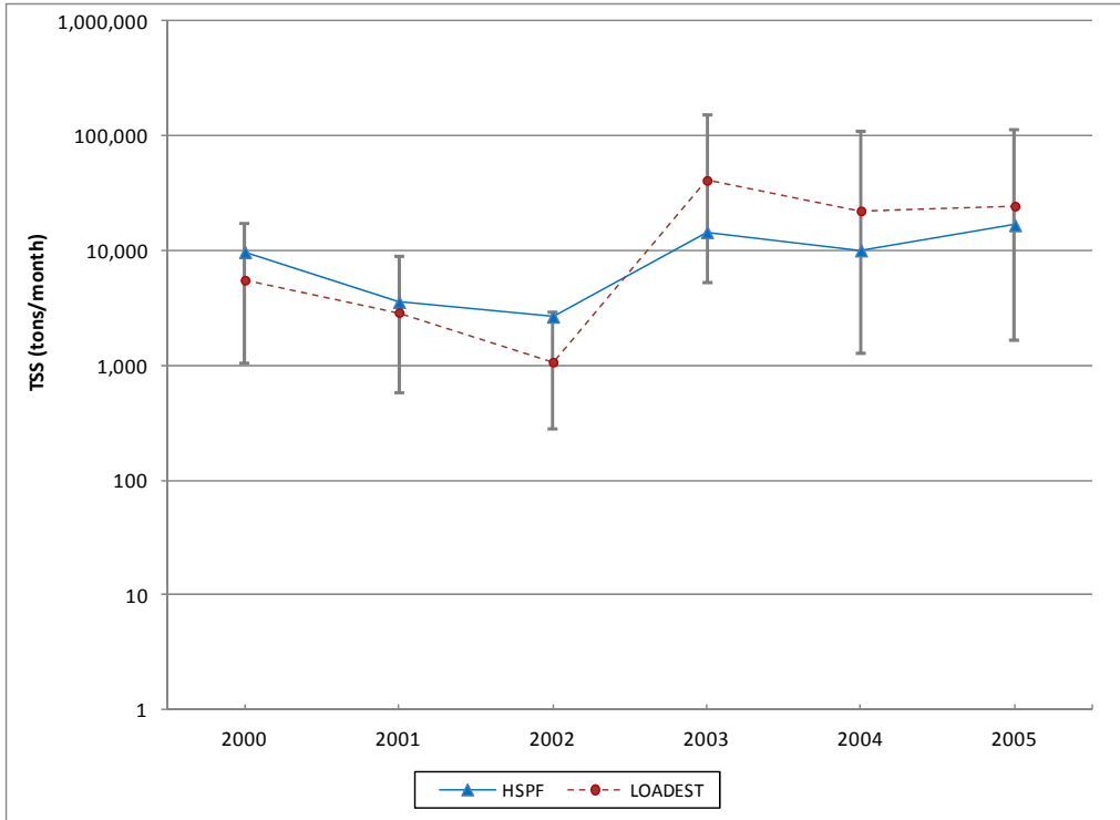
Figure A-13: Time Series of LOADEST and HSPF Annual Sediment Loads, North Branch Patapsco River
