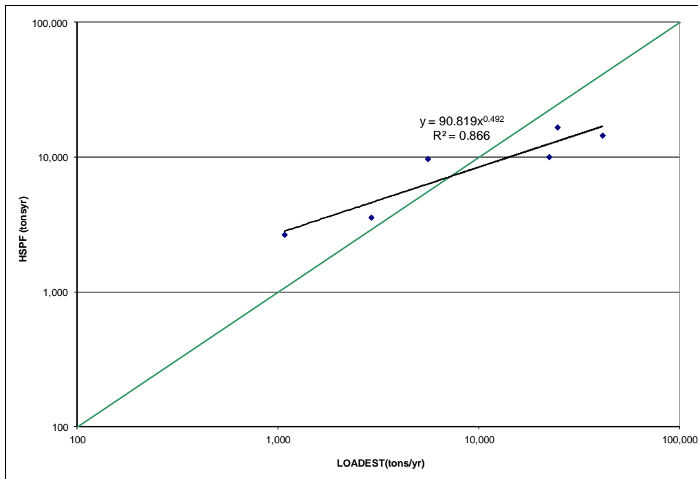
Figure A-16: Scatter Plot, ESTIMATOR and HSPF Annual Sediment Loads, North Branch Patapsco River
