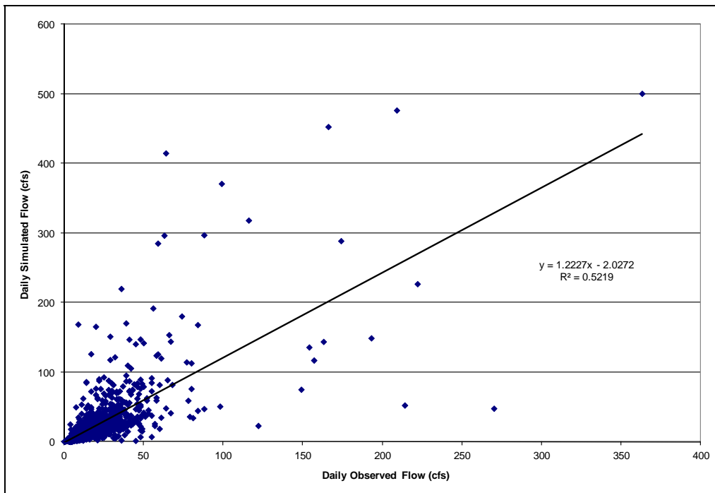
Figure A-6: Observed vs. Simulated Daily Flows, Beaver Run
