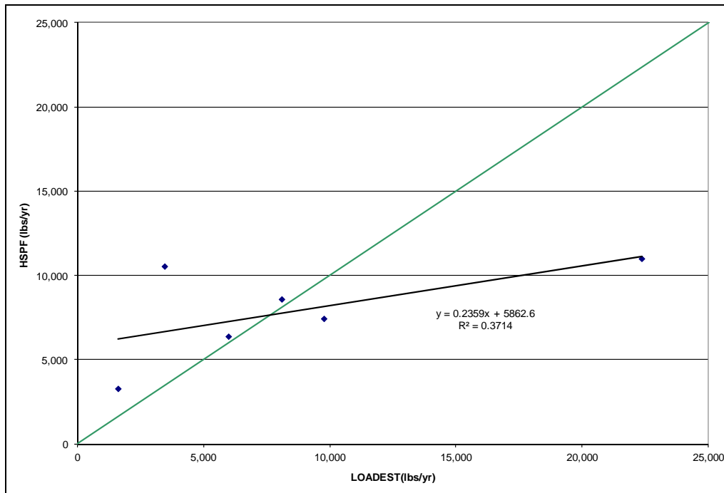
Figure A-40: Scatter Plot, ESTIMATOR and HSPF Annual Ammonia Loads, North Branch Patapsco River
