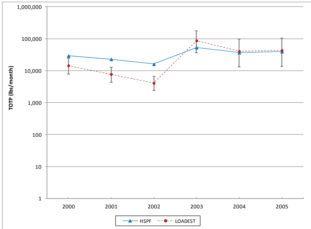
Figure A-25: Time Series of LOADEST and HSPF Annual Total Phosphorus Loads, North Branch Patapsco River
