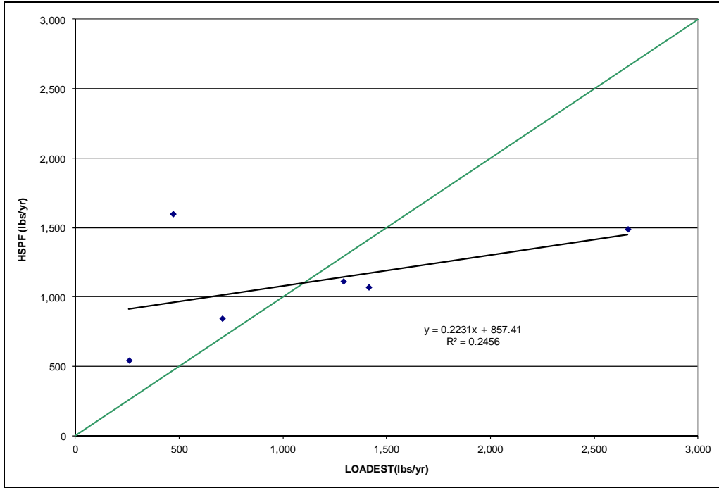
Figure A-41: Scatter Plot, ESTIMATOR and HSPF Annual Ammonia Loads, Beaver Run
