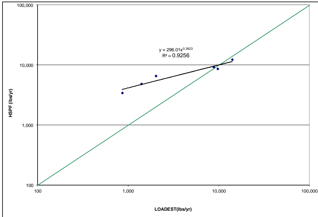
Figure A-29: Scatter Plot, ESTIMATOR and HSPF Annual Total Phosphorus Loads, Beaver Run
