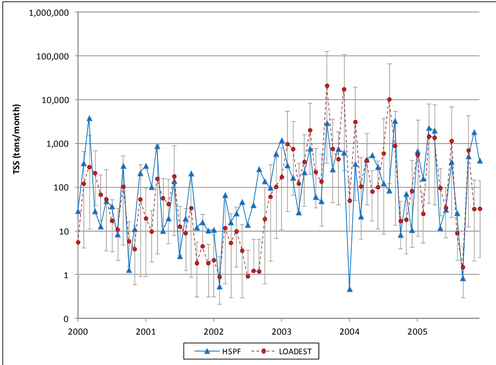
Figure A-21 Time Series of LOADEST and HSPF Monthly Sediment Loads, Morgan Run
