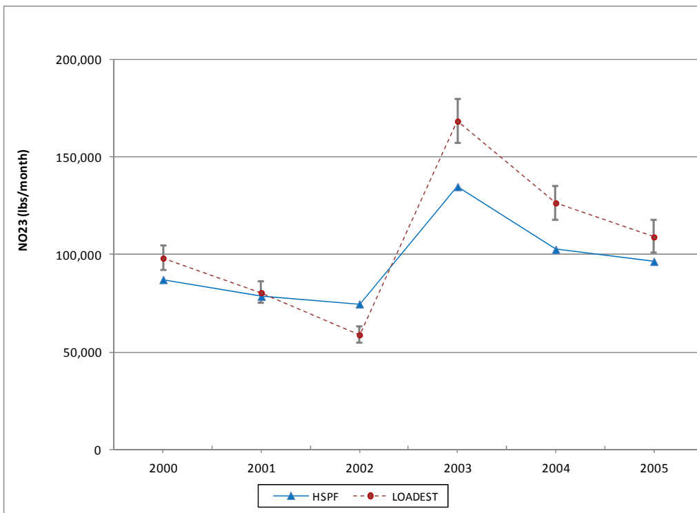
Figure A-50: Time Series of LOADEST and HSPF Annual Nitrate Loads, Beaver Run
