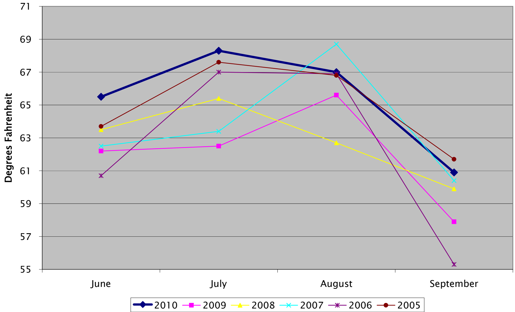
Average Temperature by Month for Selected Years
